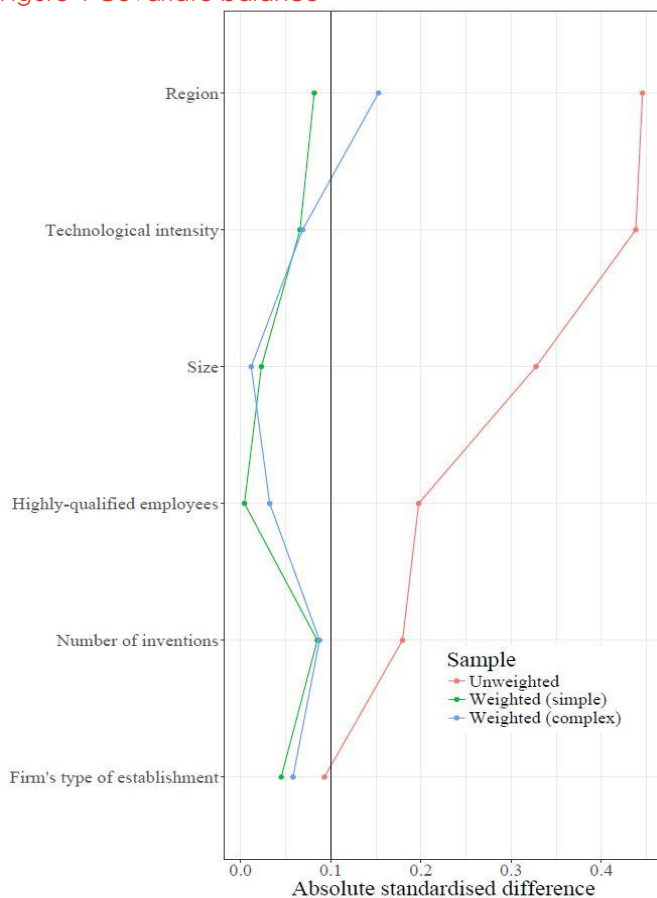
Figure 4 Covariate balance
