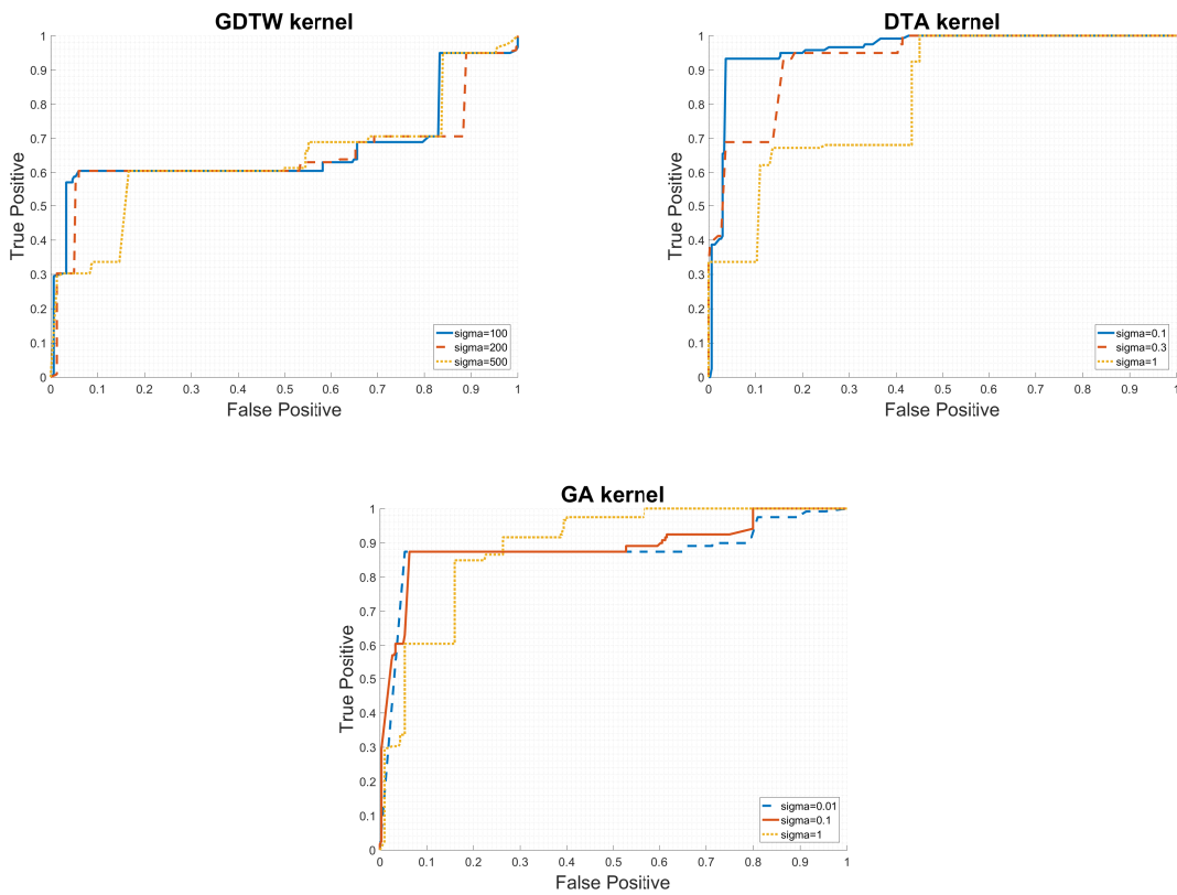
Figure 5-4 – ROC curves of multiple kernels of the one-class SVM model. From left to right, and then down are the ROC curves of three kernels GDTW, DTA, GA respectively.
