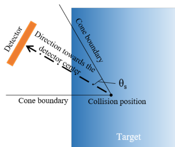
Figure 3.2 – Illustration of the initial directions of virtual ions.
