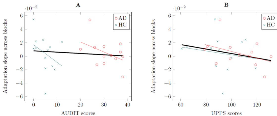
Figure 6.2 – Correlations between AUDIT (A) and UPPS scores (B) with the PBI adaptation slope across blocks during the AX-CPT task in the entire sample ( N = 26 , black lines). Red circles represent the alcohol-dependent patients group (AD) and the green crosses represent the matched controls group (HC).
