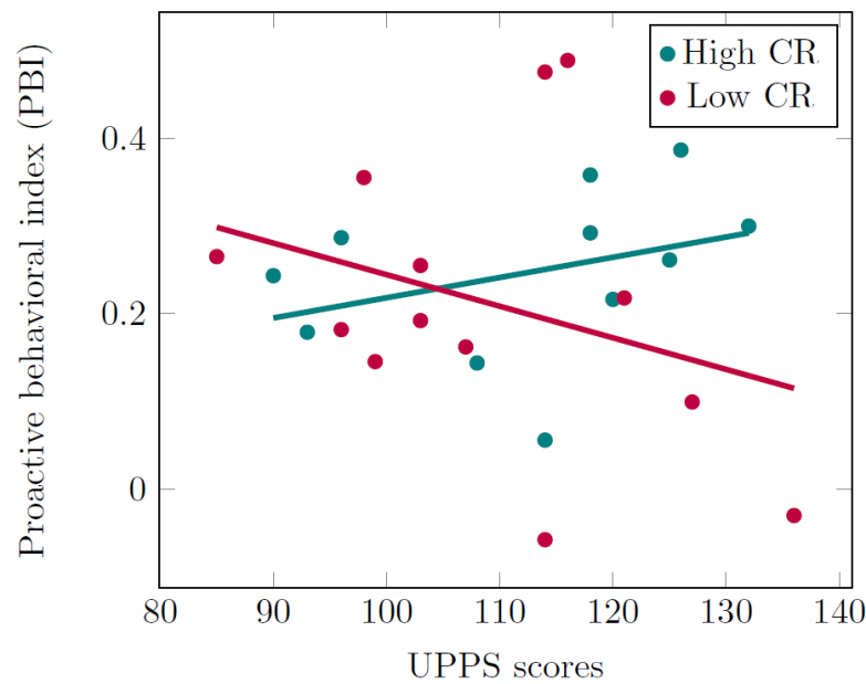
Figure 5.7 – Proactive behavioral index as a function of the UPPS scores and the correction ratio (CR) . High and low CR groups were created using the median-split method for visualization purposes only.
