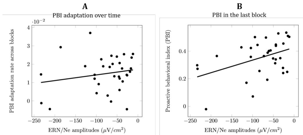
Figure 8.5 – Correlations between the the ERN/Ne amplitudes ( \mu\text{V}/\text{cm}^2 ) and (A) the adaptation of the proactive behavioral index (PBI) across blocks and (B) the PBI in the last block.
