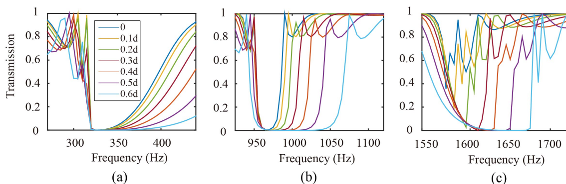
Figure 5.16: Numerical transmission as a function of water level. (a-c) Numerical transmission spectra around the 0th, 1st and 2nd locally resonant band gaps are shown as a function of the height of water.
