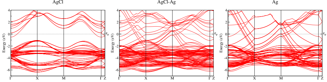
Figure 12.11: Valence and conduction band structure of the system with 10 layers. Left is pure silver chloride, right is pure silver and middle is the heterostructure.
