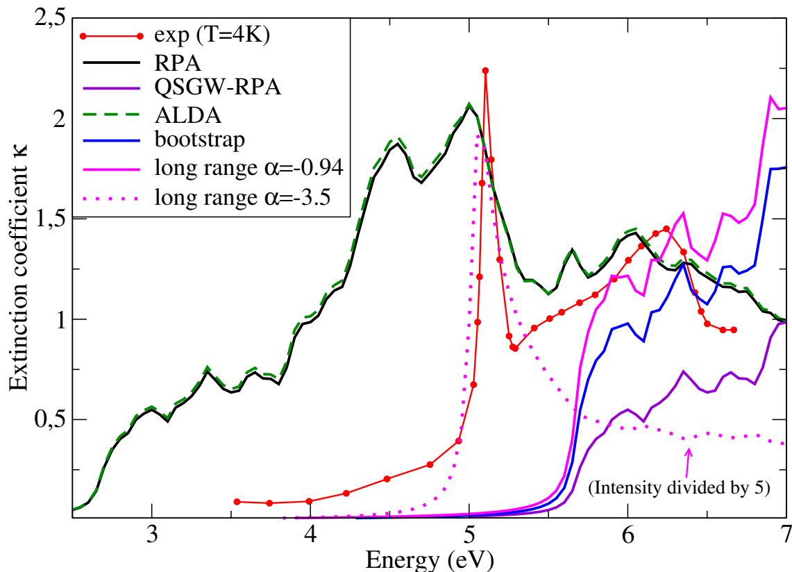
Figure 8.10: Comparison between the extinction coefficient of AgCl measured at 4 K with several TDDFT approximations. Since the energy range is limited to 3-7 eV, these spectra have been calculated with only 4 conduction bands.
