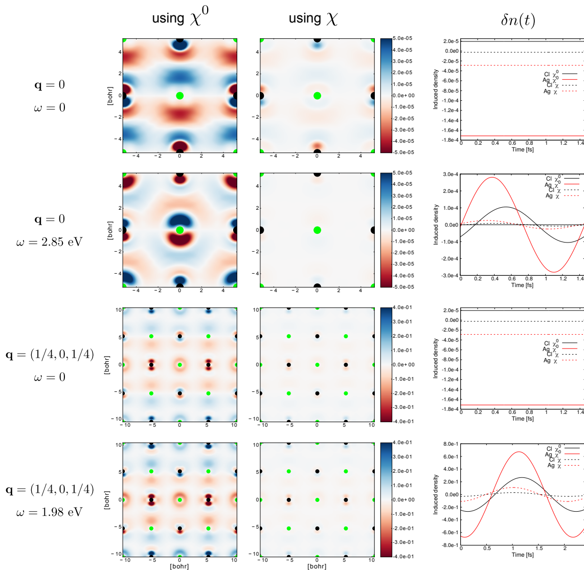
Figure 11.15: Response of silver chloride to plane-wave perturbations with different momenta and energies in the independent particle approximation and the random phase approximation. The left and center column show the induced density in a 2D plan passing by the atoms and perpendicular to the [001] direction. The left column presents the induced density computed with the independent particle polarizability while the center column presents the induced density computed with the RPA polarizability. The right column compares the independent-particle and RPA induced density as a function of time at two positions, one close to silver and the other close to chlorine atoms. These positions are chosen because they are a local maximum close to each atom. The first row shows a perturbation with vanishing momentum and energy, the second row shows a perturbation with vanishing momentum and \omega = 2.85 eV. The third row shows a perturbation with momentum \mathbf{q} = (1/4, 0, 1/4) and vanishing energy. The last row shows a perturbation with momentum \mathbf{q} = (1/4, 0, 1/4) and energy \omega = 1.98 eV.
