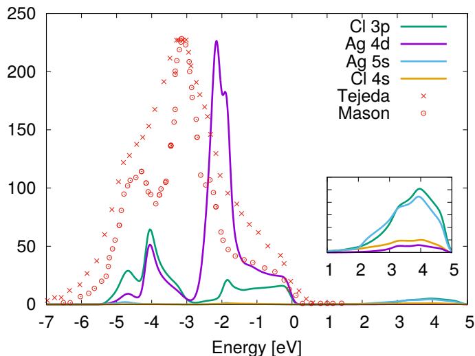
Figure 8.5: Projected density of states computed in LDA compared with experimental photoemission spectra from Mason[153] and Tejada et al. [151] at a photon energy h\nu = 1486.6 eV. The top valence is aligned with the origin of the abscissa axis. The insert shows a zoom of the calculated conduction bands.
