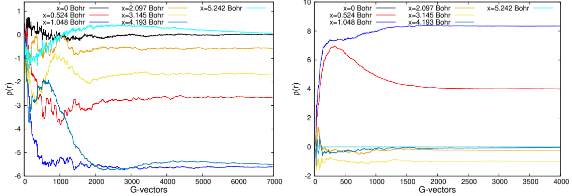
Figure 11.7: \tilde{\rho}(\mathbf{r}) = \sum_{\mathbf{G}}^{\mathbf{G}_{max}} e^{i\mathbf{G}\cdot\mathbf{r}} \tilde{\rho}(\mathbf{G}) as a function of \mathbf{G}_{max} . Calculations are made for different positions \mathbf{r} . The left panel shows a transition between top valence and bottom conduction at \mathbf{k}=(0.49,0.23,0.11) . The right panel shows a transition between top valence and bottom conduction at \mathbf{k} = \Gamma .
