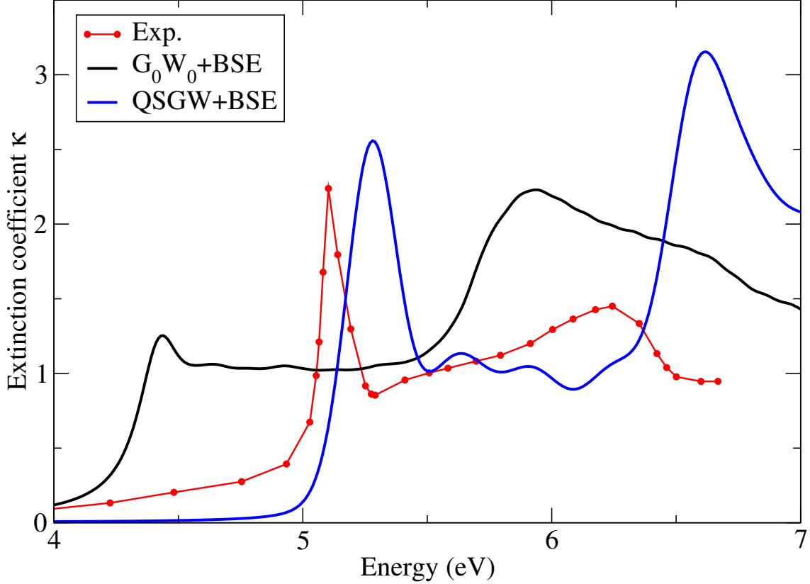
Figure 10.2: Extinction coefficient of AgCl: comparison between experimental results[51], and G_0W_0+BSE and QSGW+BSE calculations.
