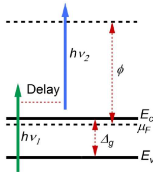
Figure 3.4: A time-resolved ARPES energy diagram. Here E_c is the bottom of the conduction band, E_v is the top of the valence band, E_F is the chemical potential, \phi is the
