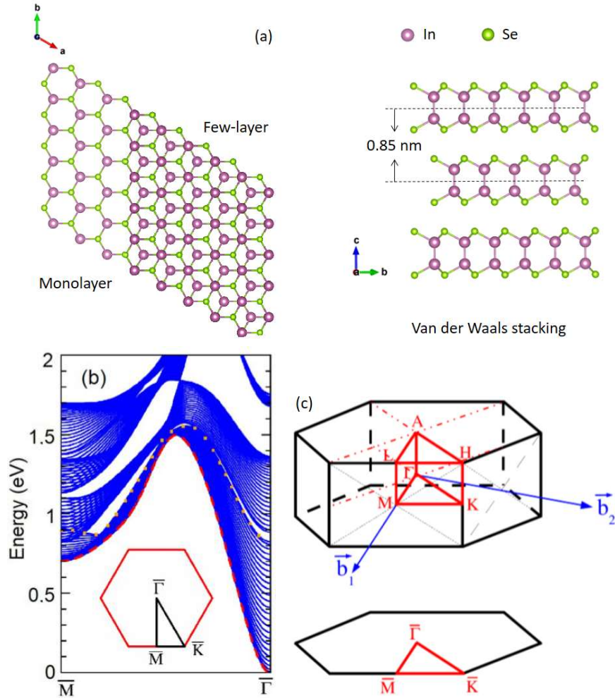
Figure 7.3: (a) Crystal structure of \epsilon -InSe. (b) Projected band structure along the high-symmetry direction \bar{\Gamma} - \bar{M} . (c) Bulk and surface Brillouin zone of \epsilon -InSe.
