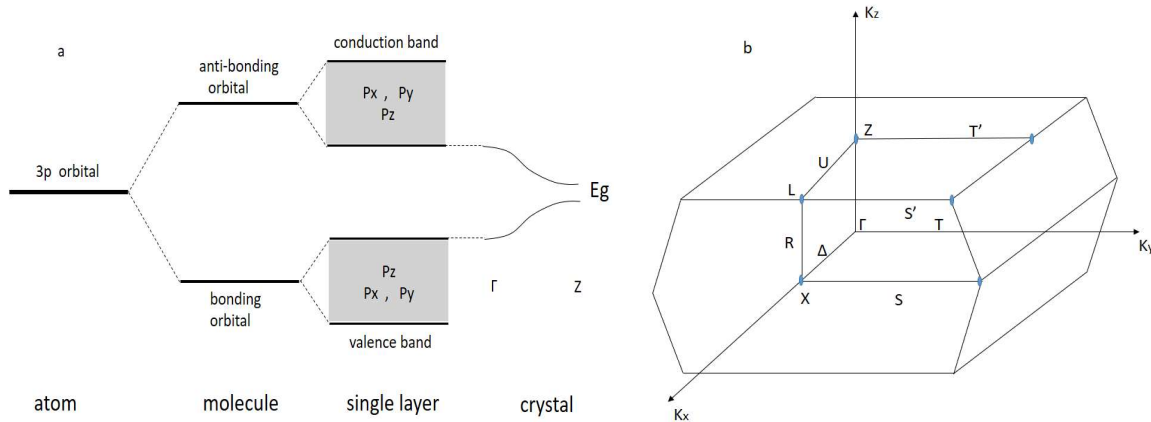
Figure 4.3: (a) Schematic energy-level diagram of phosphorous 3p orbital in atom, molecule, single puckered layer, and black phosphorous crystal. (b) The Brillouin zone of black phosphorous.
