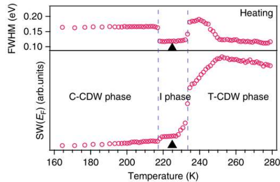
Figure 8.2: Temperature dependence of full width at half maximum (FWHM) and the spectral weight (SW) of the highest occupied band. The analyzed spectra are at the \Gamma point, where the Ta 5d band crosses E_F ( [-0.1, 0.1 eV], [-0.4, -0.3 \text{ \AA}^{-1}] ) upon heating [24].
