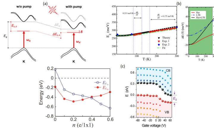
Figure 4.8: Bandgap renormalization of materials in the following conditions: (a) Electronic band structure (black line) of monolayer MoS 2 at the K point and the exciton energy (red line) in absence (left) and in presence (right) of pump pulse absorption. The overall shift of the excitonic absorption resonances ( \delta ) results from both the shrinkage of the electronic bandgap and the renormalization of the exciton binding energy, due to the presence of photoexcited carriers, i.e., \delta = \Delta E_g - \Delta E_b [35]. (b) Theoretical and experimental BP bandgap as a function of temperature. In the left frame different phononic contribution to the bandgap increase are shown [15]. (c) Calculated conduction band minimum and valence band maximum relative to chemical potential as a function of the doping level (left) [14] and Gate-controlled Stark effect in an 11-layer BP flake device: VBM (red balls), CBM (black balls) and bandgap ( E_g ) of 11-layer BP at different gate voltages (right) [12].
