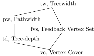
Figure 4.1: Relationships of considered parameters. Algorithmic results are inherited downwards (from \text{tw} to \text{vc} ), hardness results upwards.
