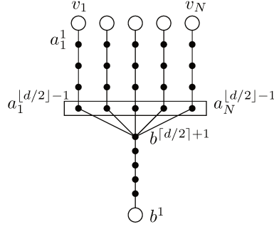
Figure 4.2: A general picture of the clause gadget \hat{C} for even and odd d . Note the box indicating vertices forming a clique for the case of even d .
