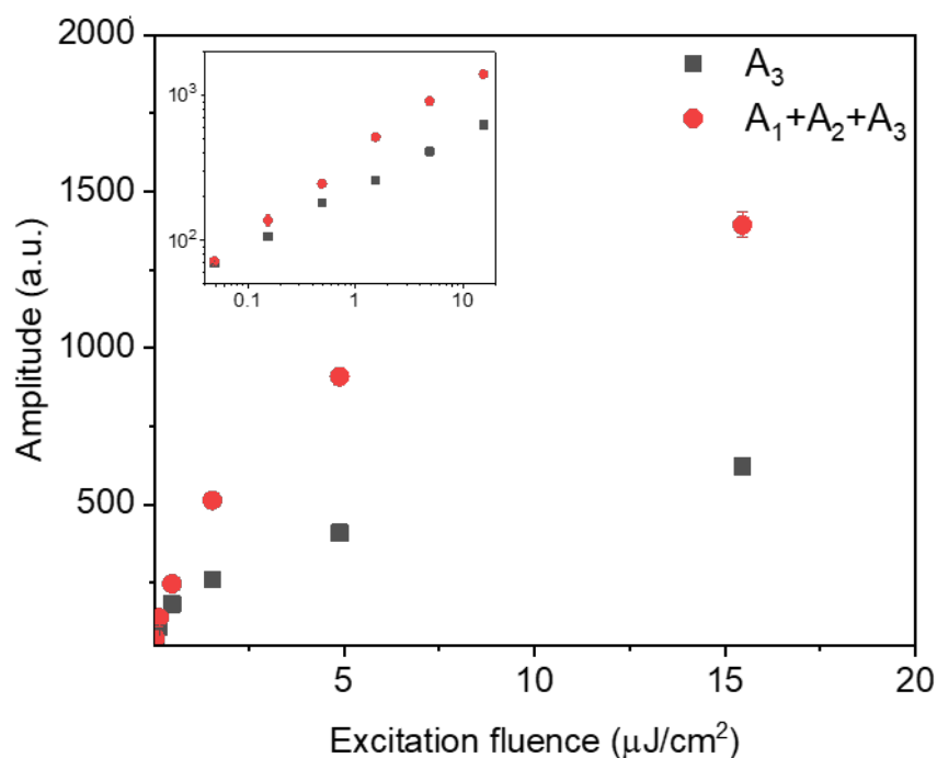
Figure 4.3. Evolution of the total ( A_1 + A_2 + A_3 , red dots) and single-exciton ( A_3 , black dots) amplitude of the time components used in the multi-exponential fit of the TR-PL decay traces of n=3 MAPI NPLs, for different excitation fluences. Inset: same graph in the log-log scale.
