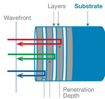
Figure 2.7. Principle of a chirped mirror (Optics Balzers).
