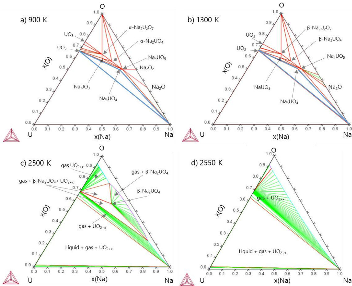
Figure 2.14: Calculated isothermal sections of the Na-O-U system at 900 K (a), 1300K (b), 2500K (c), 2550K (d) using the Calphad model of Smith et al. [6]. The stable ternary compounds at the temperature considered are reported on the sections. The UO 2 -Na 3 UO 4 -Na phase field is represented in blue on fig a) and b).
