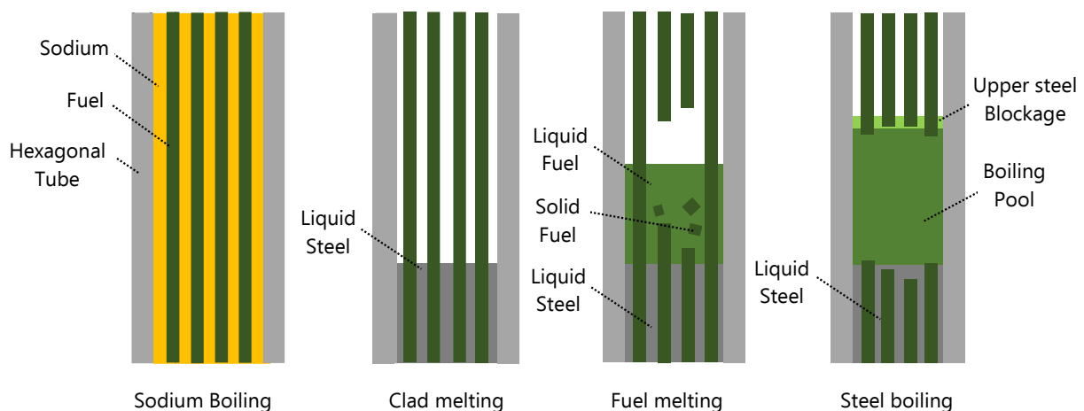
Figure 1.9: Evolution of a subassembly under a TIB scenario as described by Kayser et al. [34].
