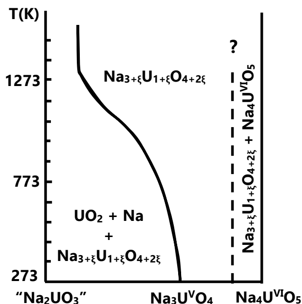
Figure 2.3: Na-O-U phase diagram section between the theoretical composition \text{Na}_2\text{UO}_3 and \text{Na}_4\text{U}^{\text{VI}}\text{O}_5 along the \text{O}/(\text{U}+\text{Na})=1 composition line [2]
