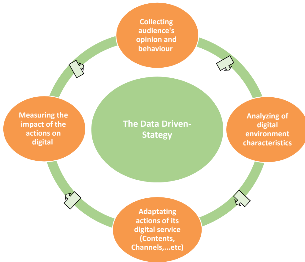
Figure 6. Data-Driven Algorithms
