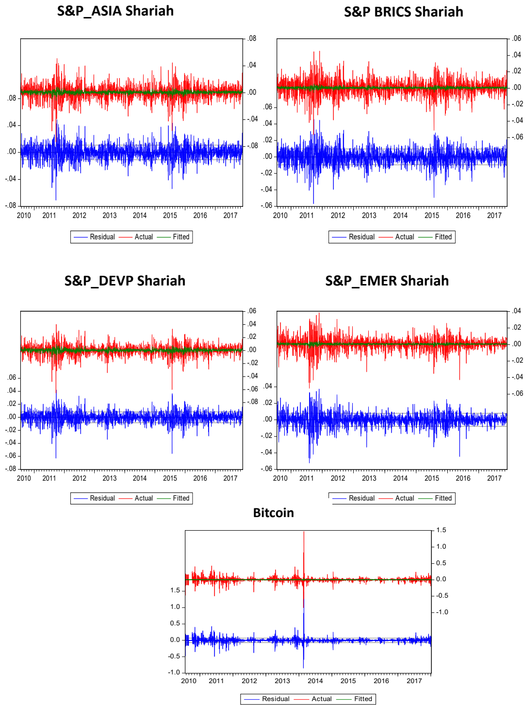
Figure 5. Residuals of Shariah indices and Bitcoin
