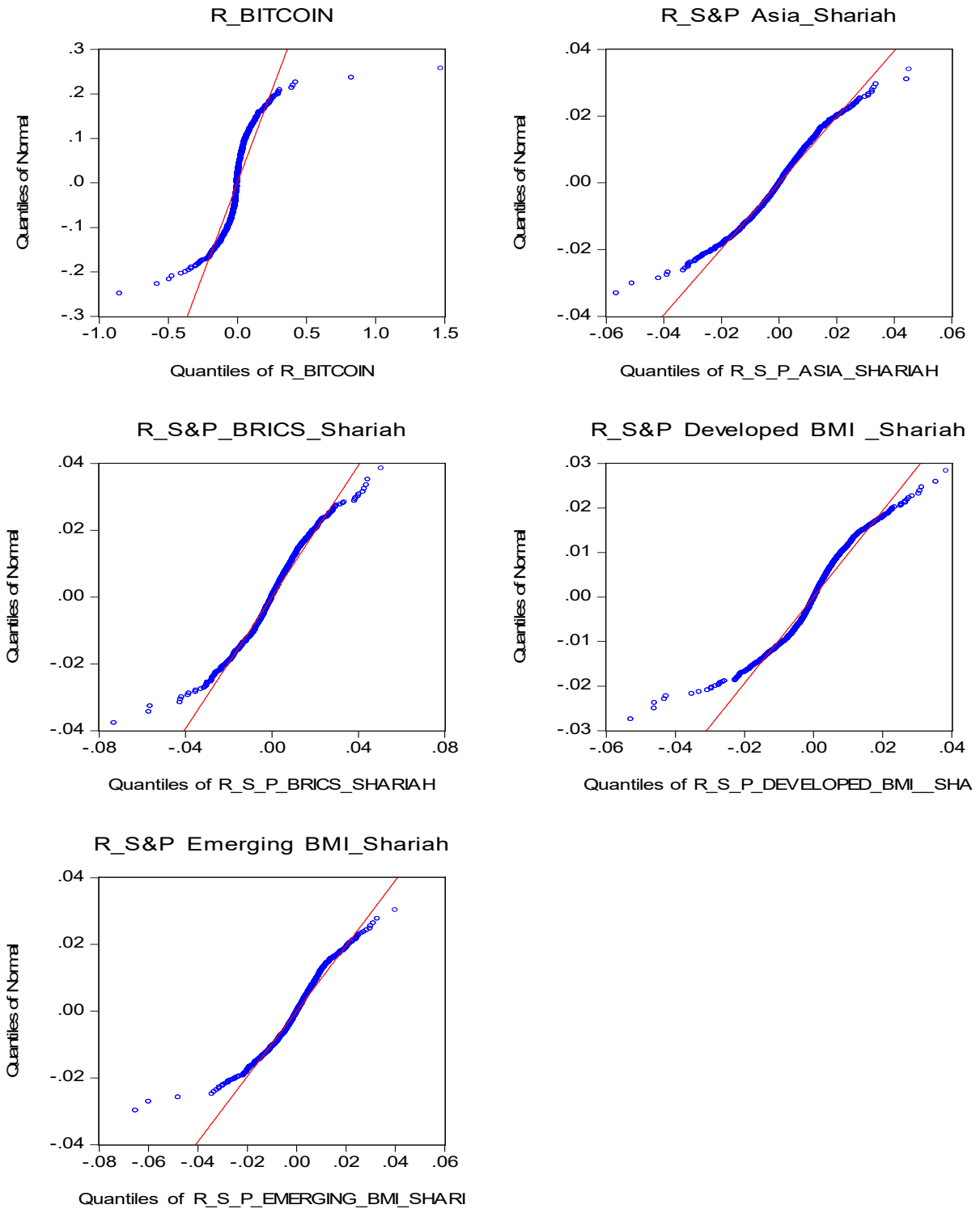
Figure 7. Q-Q plots of Index returns normally distributed for Islamic indices and Bitcoin
