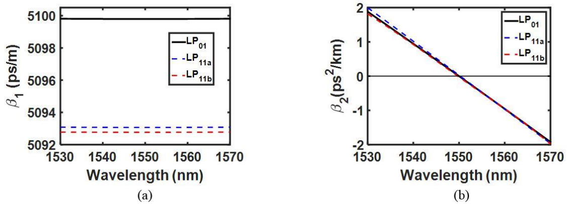
Figure 3.6: (a) Inverse group velocity of the three modes and (b) group velocity dispersion of the three modes.
