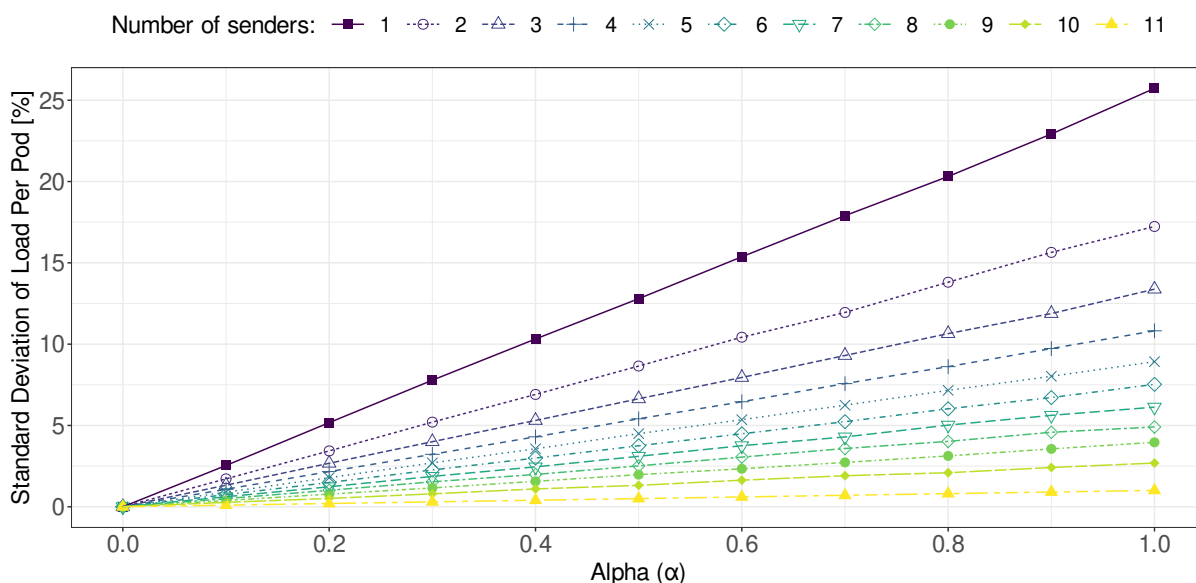
Figure 4.8 – Overall system load imbalance as a function of \alpha and the number of senders.
