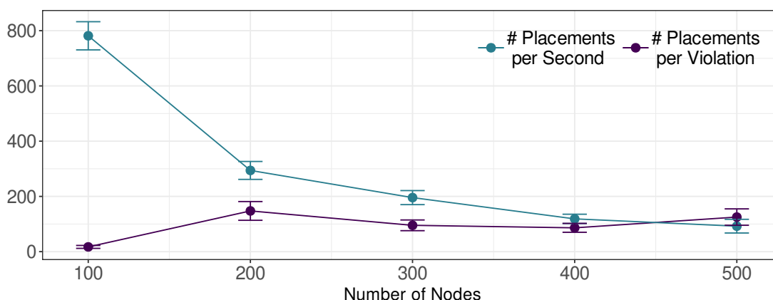
Figure 6.7 – Scalability (simulator).
