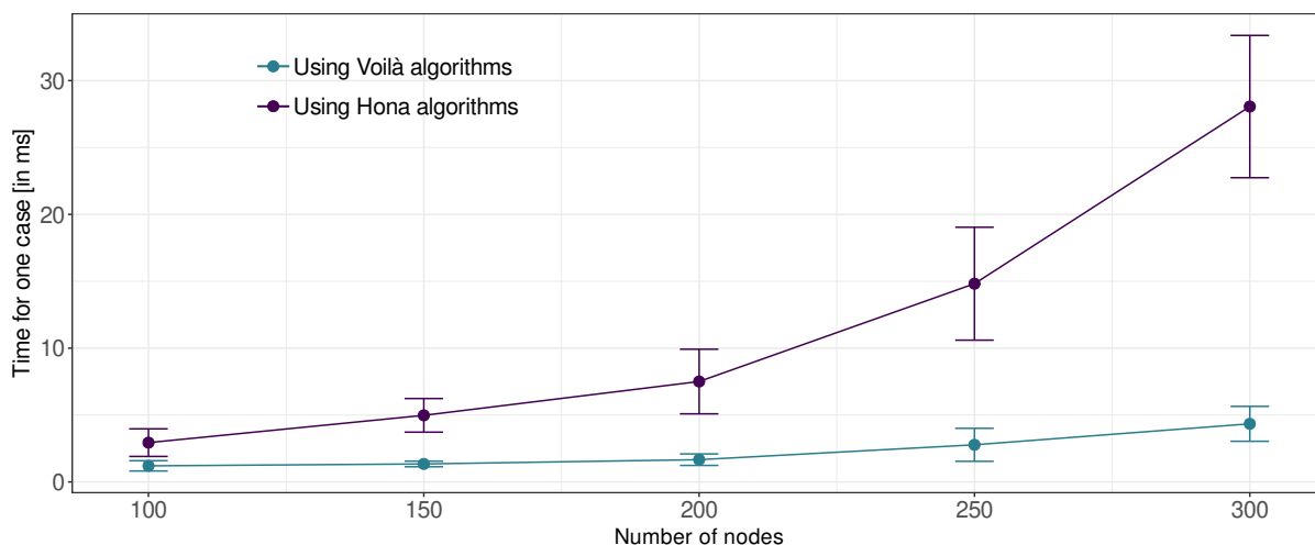
Figure 6.3 – Time needed to compute the objective function for both Hona and Voilà as a function of the number of nodes.
