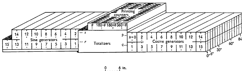
Fig. 4. Diagrammatic view of computer.
