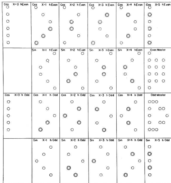
FIG. 4. Layout of stencils for N=20 . The ringed holes correspond to negative values. The same cards can be used for the sine and the cosine stencils, one side of each card serving for the cosine summation and the other side for the sine summation.
