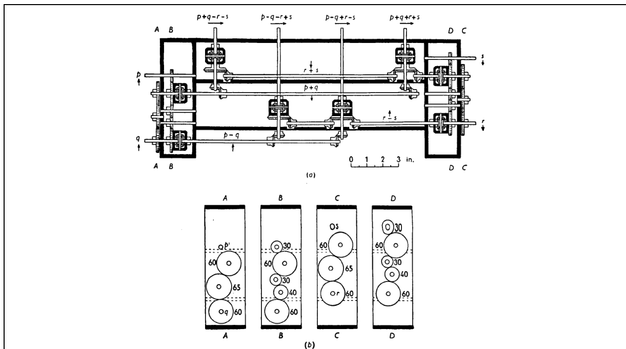
Fig. 3. (a) Totalizer unit for combining sub-totals. (b) End view of gearing in totalizer unit.
