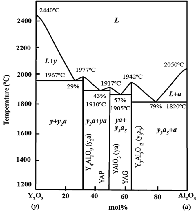
Figure I.15: Phase diagram for system Y_2O_3 - Al_2O_3 from [49].
