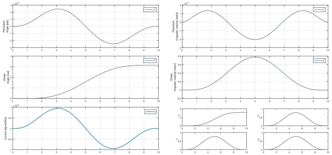
FIGURE 7.11: S4. Rest-to-rest trajectory tracking for Inertia Wheel Pendulum.
