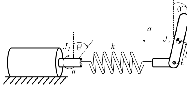
FIGURE 3.4: The single link manipulator with joint elasticity
