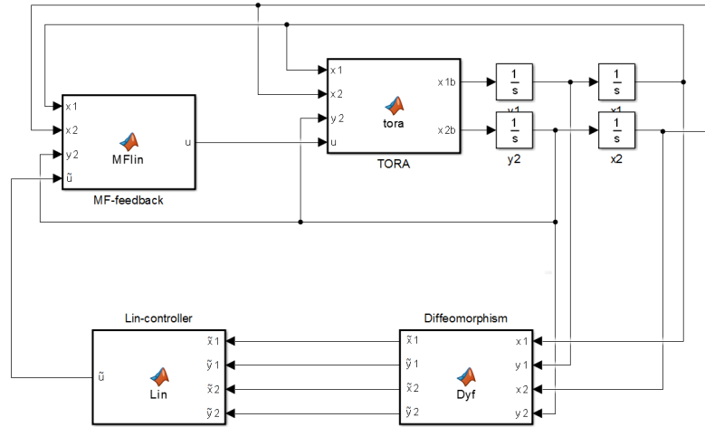
FIGURE 7.16: The simulation scheme for stabilization of the TORA system.
