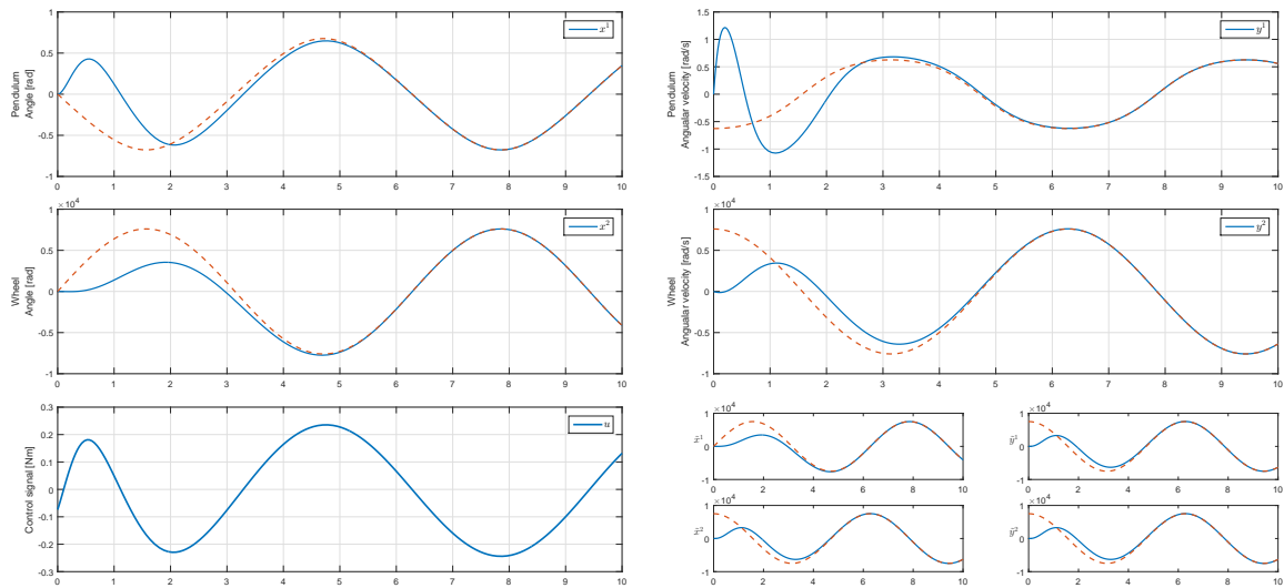
FIGURE 7.15: S7. Sinusoidal trajectory tracking of the Inertia Wheel Pendulum.
