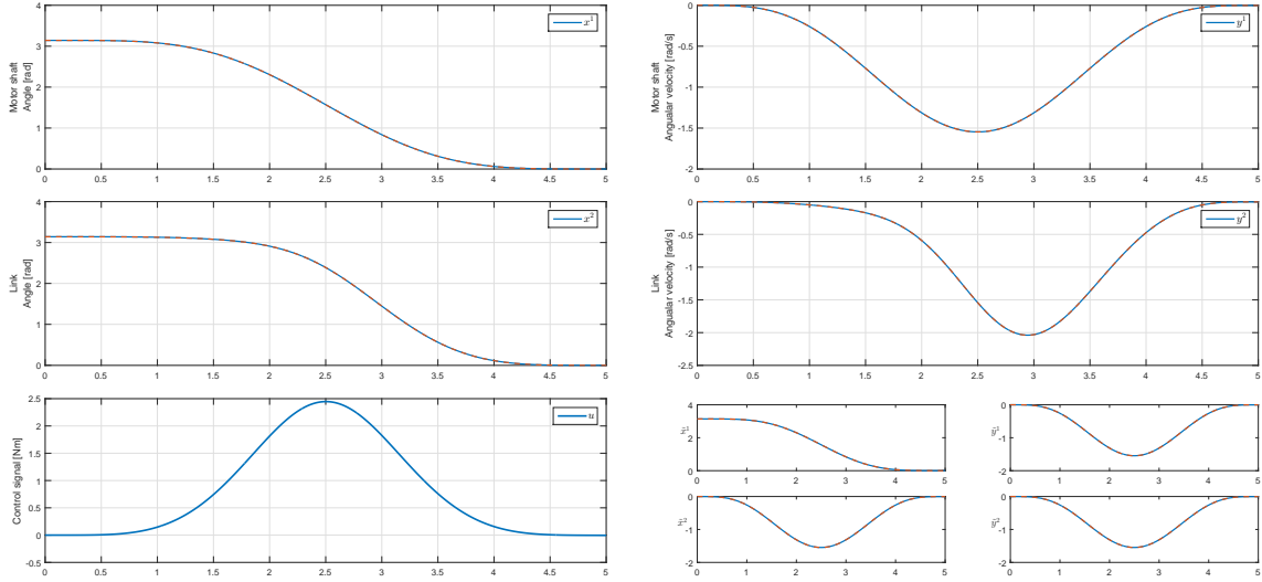
FIGURE 7.26: S12. Rest-to-rest trajectory tracking for the FLEX system.
