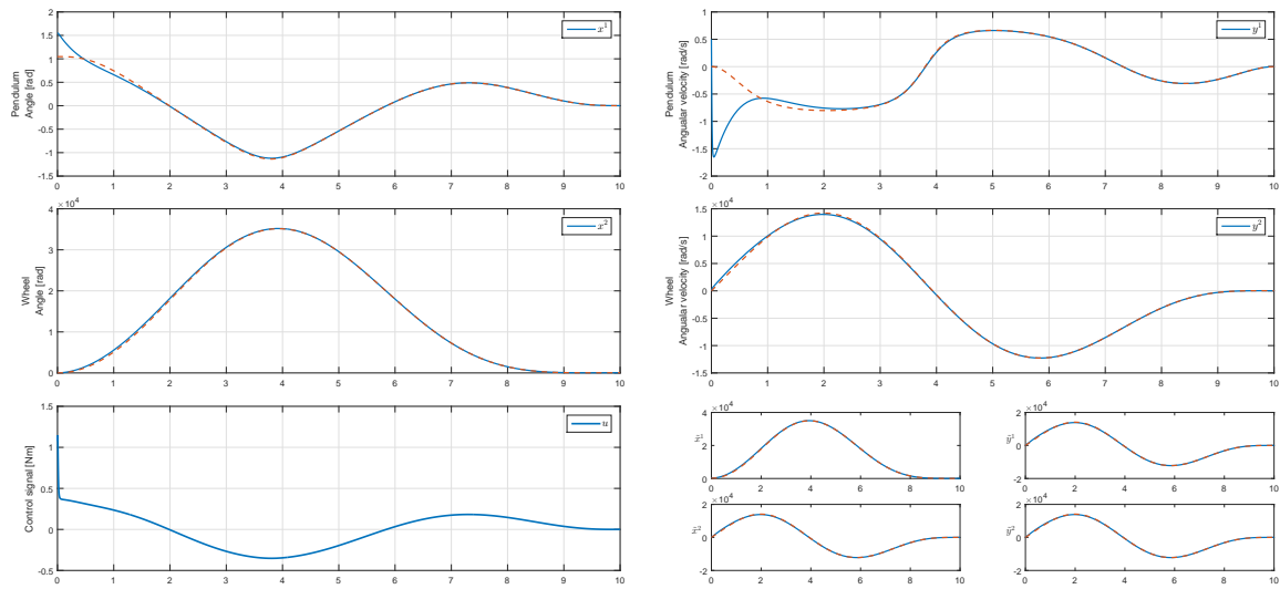
FIGURE 7.13: S5b. Trajectory tracking for mismatched initial conditions of the Inertia Wheel Pendulum.
