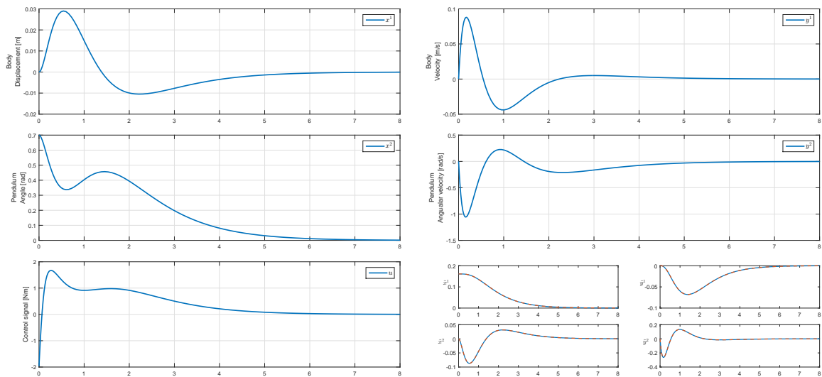
FIGURE 7.18: S8b. The simulation results for the TORA system with the pole placement tuning.
