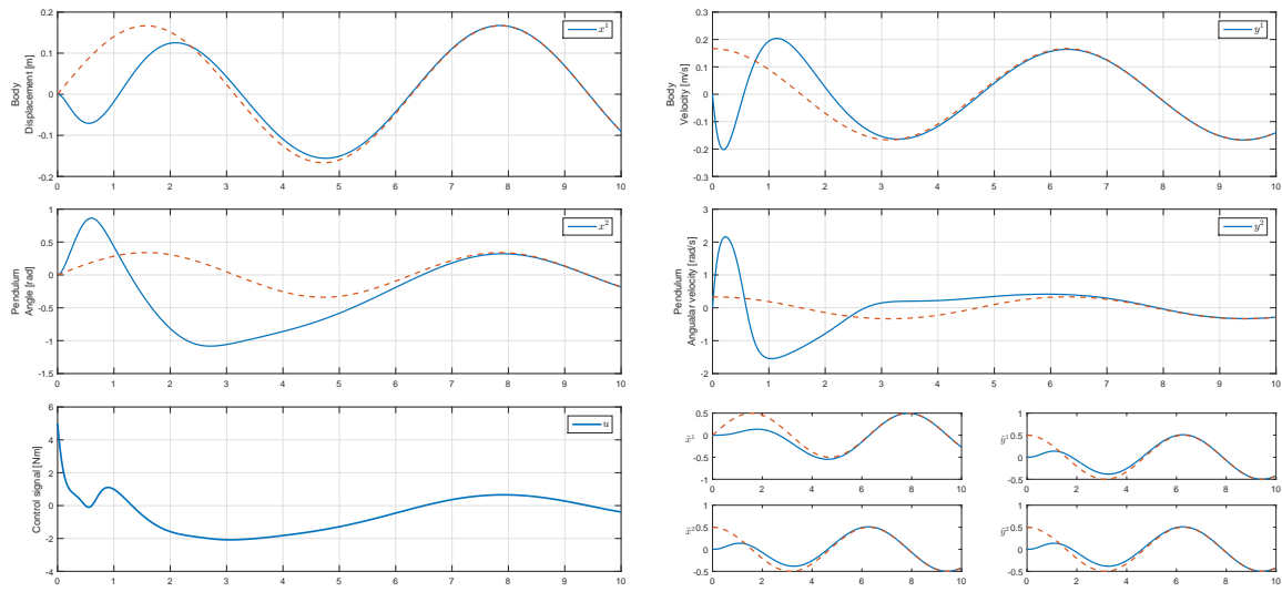
FIGURE 7.20: S9. Sinusoidal trajectory tracking of the TORA system.
