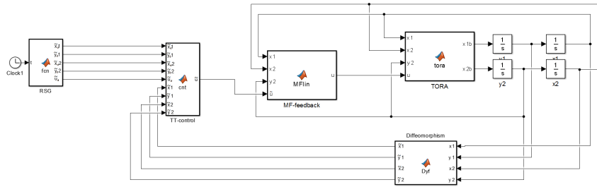
FIGURE 7.19: The simulation scheme for trajectory tracking of the TORA system.
