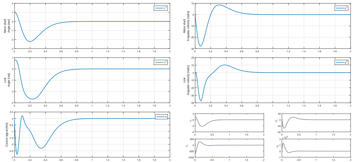
FIGURE 7.22: S10a. The simulation results for the FLEX system with the natural frequency tuning.
