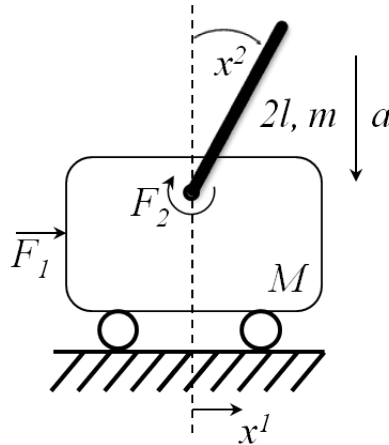
FIGURE 7.2: Cart-pole system.
