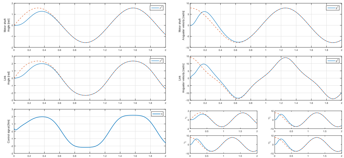
FIGURE 7.27: S13. Sinusoidal trajectory tracking of the FLEX system.
