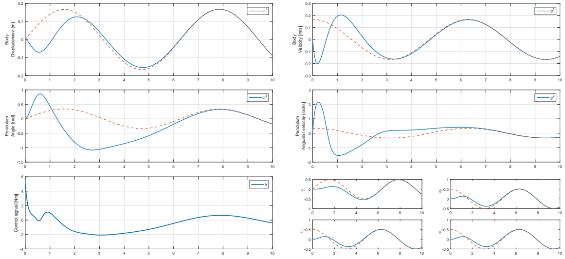
FIGURE 7.20: S9. Sinusoidal trajectory tracking of the TORA system.
