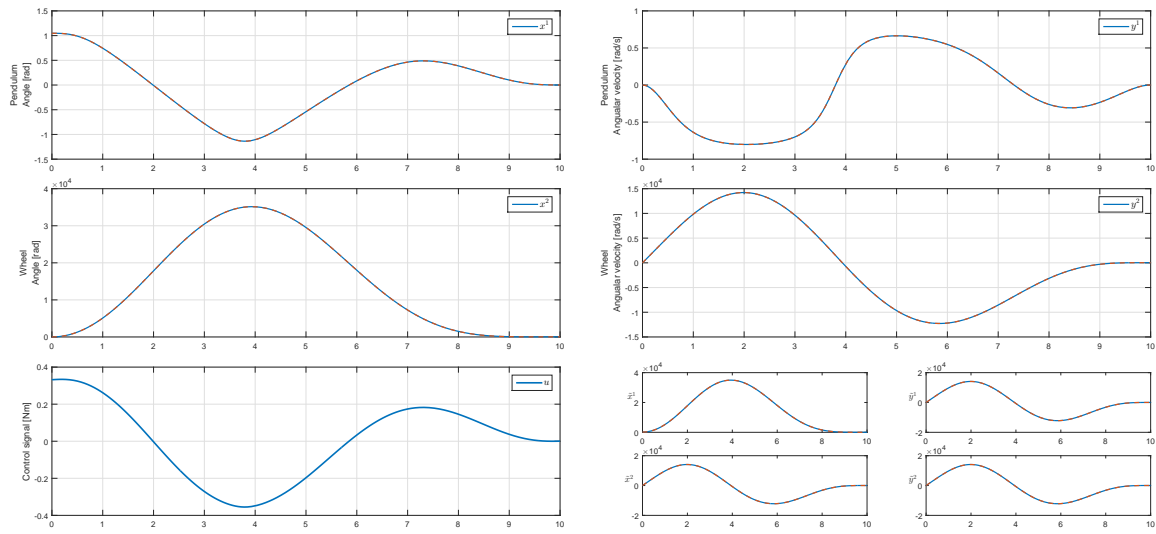
FIGURE 7.12: S5a. Trajectory tracking for matched initial conditions of the Inertia Wheel Pendulum.
