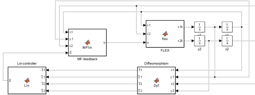
FIGURE 7.21: The simulation scheme for the FLEX system.
