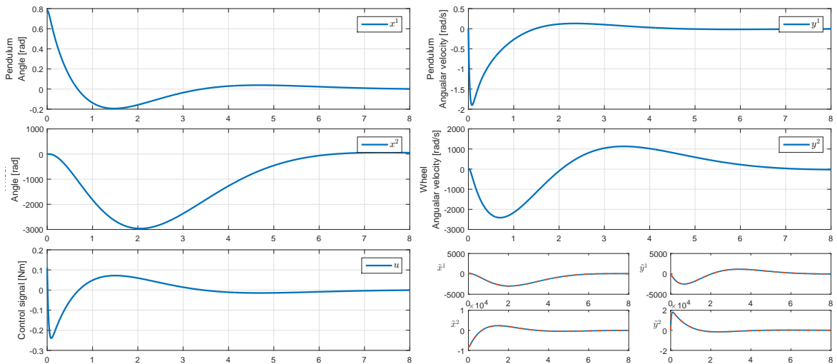
FIGURE 7.7: S1c. The simulation results for the Inertia Wheel Pendulum with LQR tuning.
