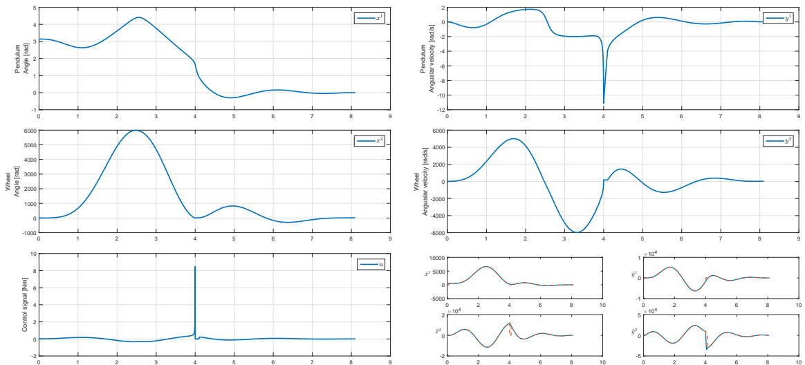
FIGURE 7.14: S6. Tracking the trajectory that passes through the singularity of the Inertia Wheel Pendulum.
