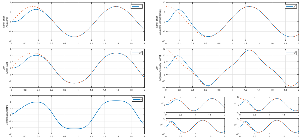
FIGURE 7.27: S13. Sinusoidal trajectory tracking of the FLEX system.
