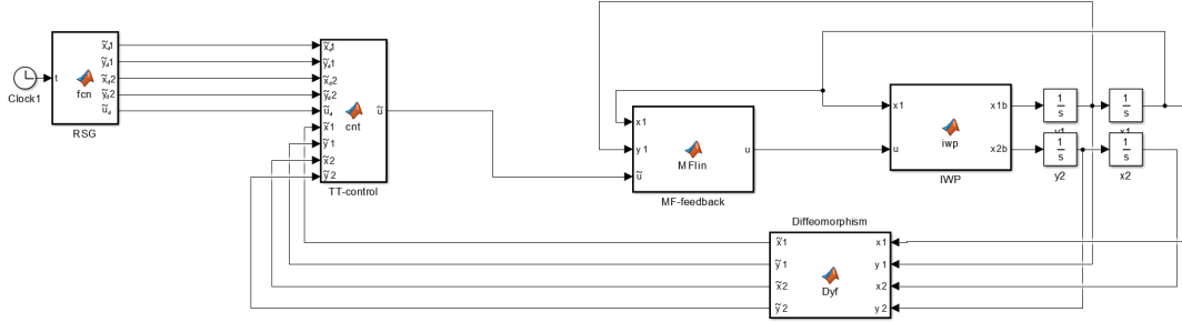
FIGURE 7.10: The simulation scheme for trajectory tracking of the Inertia Wheel Pendulum.
