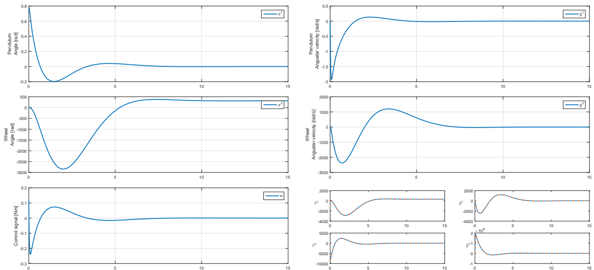
FIGURE 7.9: S3. The simulation results for the Inertia Wheel Pendulum outside the origin.
