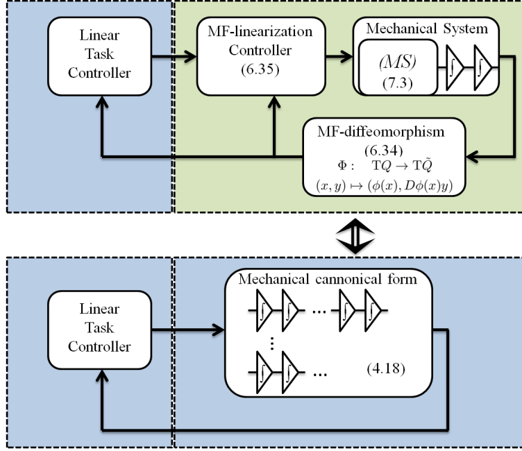
FIGURE 7.3: The cascade controller for MF-linearizable (\mathcal{MS}) .
