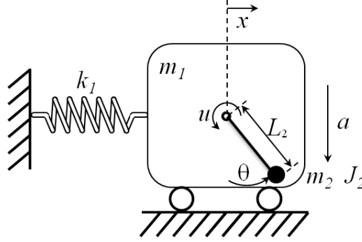
FIGURE 3.3: The TORA system
