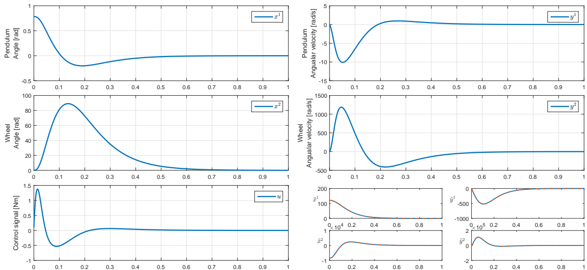
FIGURE 7.6: S1b. The simulation results for the Inertia Wheel Pendulum with pole placement tuning.
