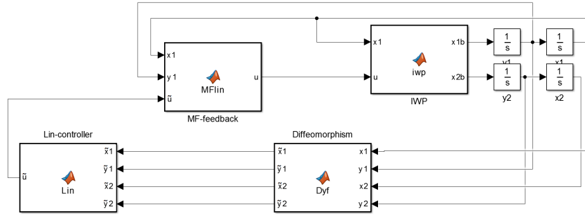
FIGURE 7.4: The simulation scheme for stabilization of the Inertia Wheel Pendulum.
