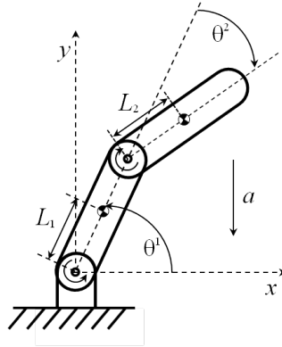
FIGURE 3.1: The two-link manipulator
