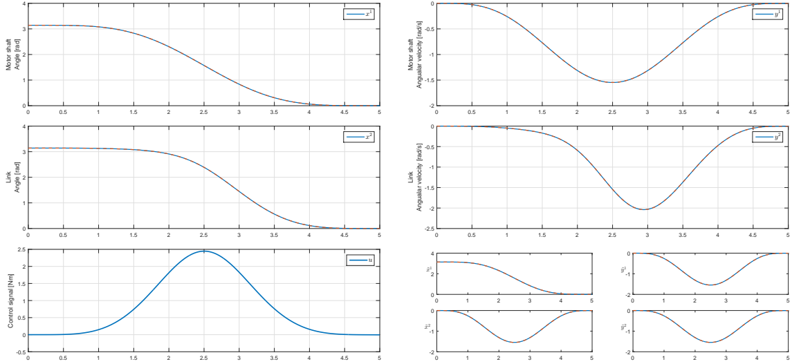
FIGURE 7.26: S12. Rest-to-rest trajectory tracking for the FLEX system.
