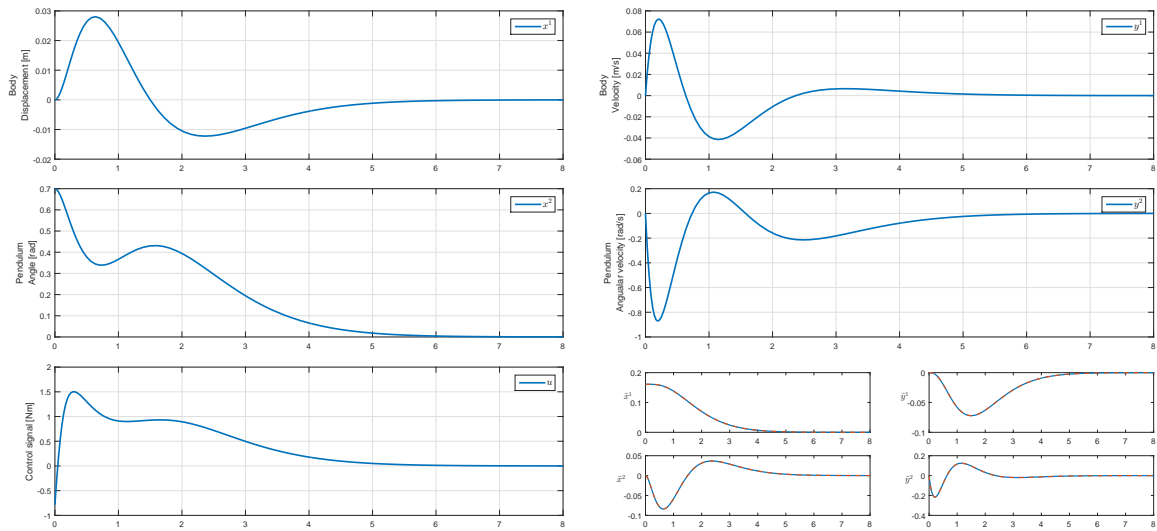
FIGURE 7.17: S8a. The simulation results for the TORA system with the natural frequency tuning.
