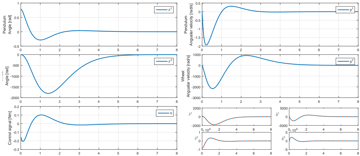
FIGURE 7.5: S1a. The simulation results for the Inertia Wheel Pendulum with the natural frequency tuning.
