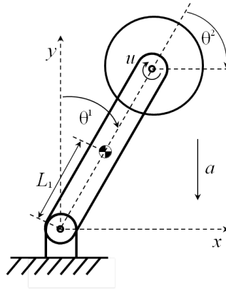
FIGURE 3.2: The inertia wheel pendulum
