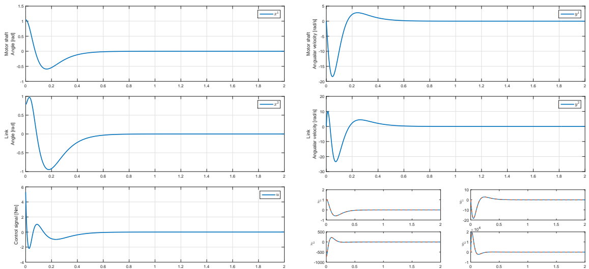
FIGURE 7.23: S10b. The simulation results for the FLEX system with pole placement tuning.
