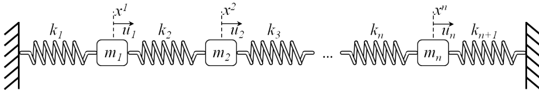
FIGURE 4.1: The n -coupled spring-mass system
