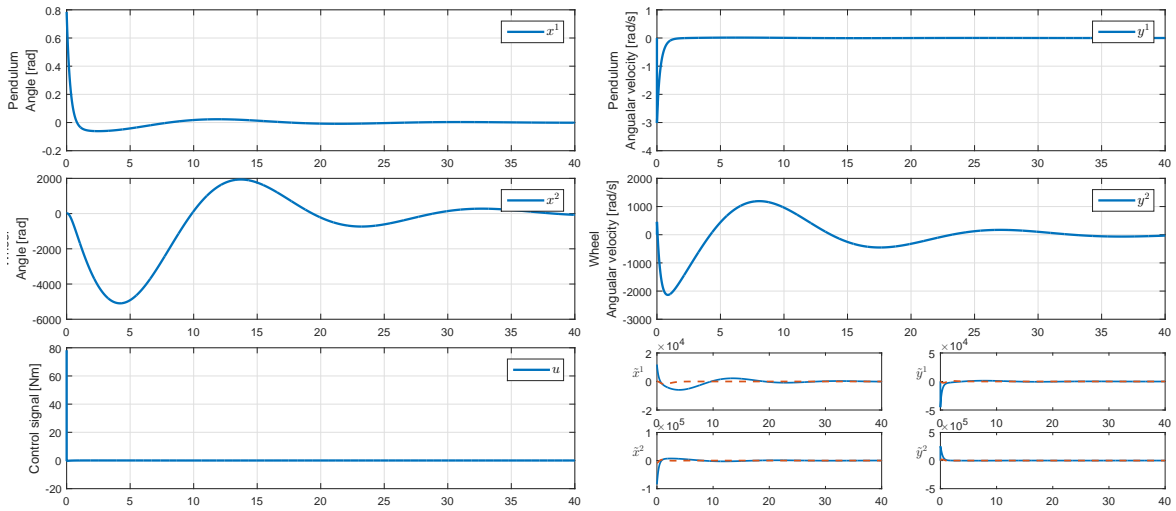
FIGURE 7.8: S2. The simulation results for the Inertia Wheel Pendulum with the parametric uncertainties of 1000%.
