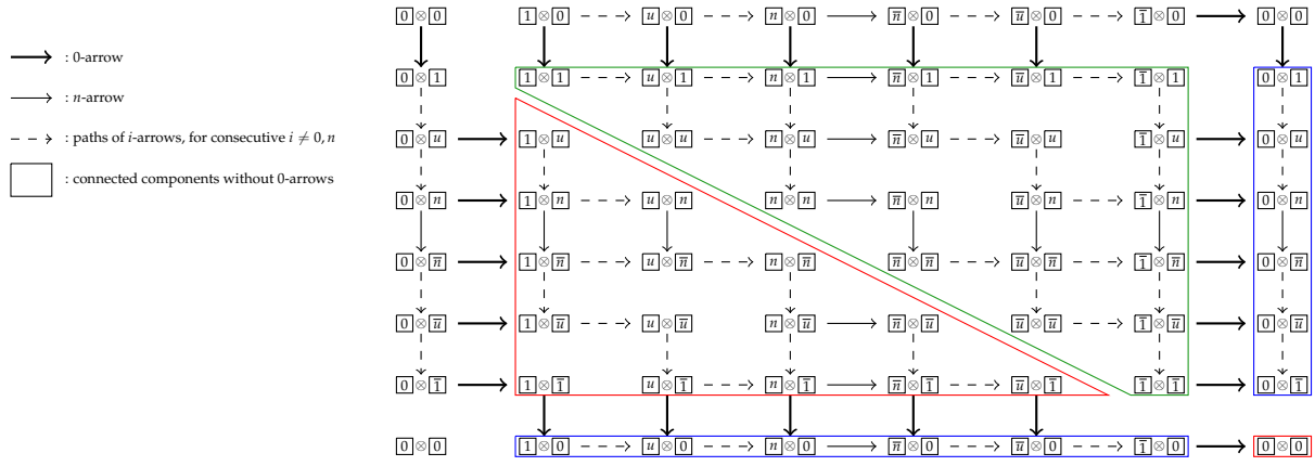
FIGURE 10.2: Crystal graph of \mathcal{B} \otimes \mathcal{B} for type A_{2n}^{(2)} ( n \geq 2 )
