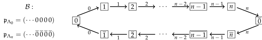
FIGURE 10.3: Crystal graph \mathcal{B} of the vector representation for type D_{n+1}^{(2)} ( n \geq 2 )
