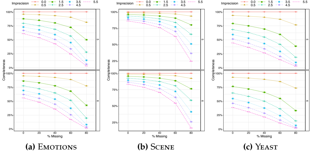
Figure 5.9: Missing labels. Evolution of the average completeness (%) for each level of imprecision (a curve for each one) and discretization z = 5 (top) and z = 6 (down), with respect the percentage of missing labels..
