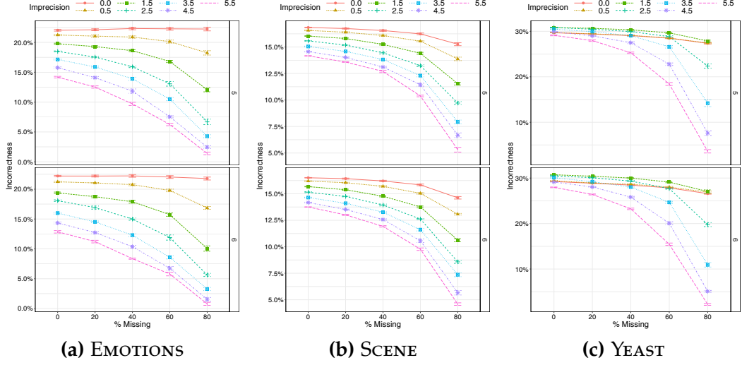
Figure 5.8: Missing labels. Evolution of the average incorrectness (%) for each level of imprecision (a curve for each one) and discretization z = 5 (top) and z = 6 (down), with respect the percentage of missing labels.
