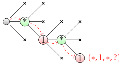
Figure 6.3: Marginalization strategy for four labels \{Y_1, Y_2, Y_3, Y_4\}
