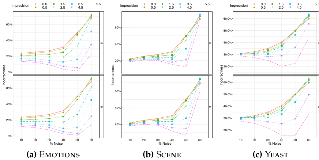
Figure 5.10: Noise-Reversing . Evolution of the average incorrectness (%) for each level of imprecision (a curve for each one) and two levels of discretization z=5 (top) and z=6 (down), with respect to the percentage of noise.
