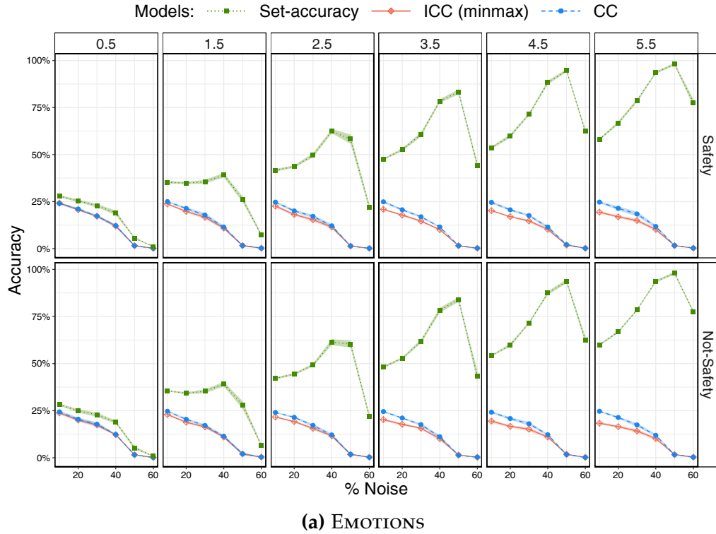
Figure B.9: Reversing - ICC versus CC - Marginalization . Figures show performance evolution (%) of the imprecise and precise classifier-chains approaches for all levels of imprecision and using the safety imprecise chaining (top) and not (down), with respect to the percentage of noiseness (x-axis).
