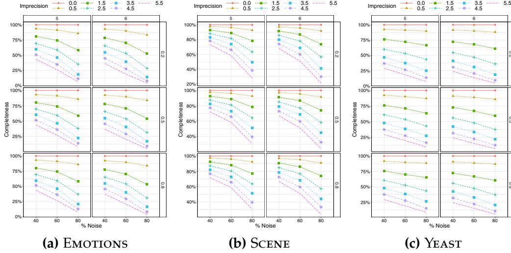
Figure 5.13: Noise-Flipping. Evolution of the average completeness (%) for each level of imprecision (a curve for each one), two levels of discretization z = 5 (left) and z = 6 (right), and three different probabilities \beta = 0.2 (top), \beta = 0.5 (middle) and \beta = 0.8 (down), with respect to the percentage of noise.
