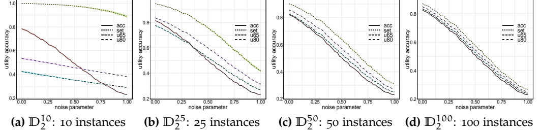
Figure 3.7: Utility accuracies (%) with confidence intervals of the (I)QDA model on corrupt test data sets \mathbb{T}_2^\epsilon using 50 training data sets with different number of instances, i.e. \{\mathbb{D}_2^{10}, \mathbb{D}_2^{25}, \mathbb{D}_2^{50}, \mathbb{D}_2^{100}\} .
