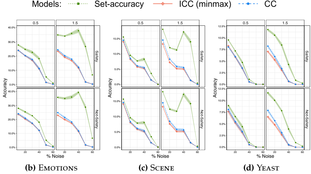
Figure 6.13: Reversing - ICC versus CC - Imprecise Branching Figures show performance evolution (%) of the imprecise and precise classifier-chains approaches for 0.5 (left) and 1.5 (right) levels of imprecisions, and using the safety imprecise chaining (top) and not (down), with respect to the percentage of noisy (x-axis).
