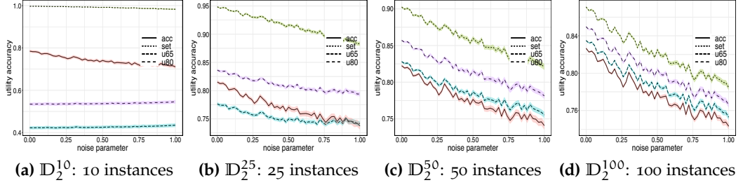
Figure 3.9: Utility accuracies (%) with confidence intervals of the (I)QDA model on corrupt test data sets \mathbb{T}_2^\psi using 50 training data sets with different number of instances, i.e. \{\mathcal{D}_2^{10}, \mathcal{D}_2^{25}, \mathcal{D}_2^{50}, \mathcal{D}_2^{100}\} .
