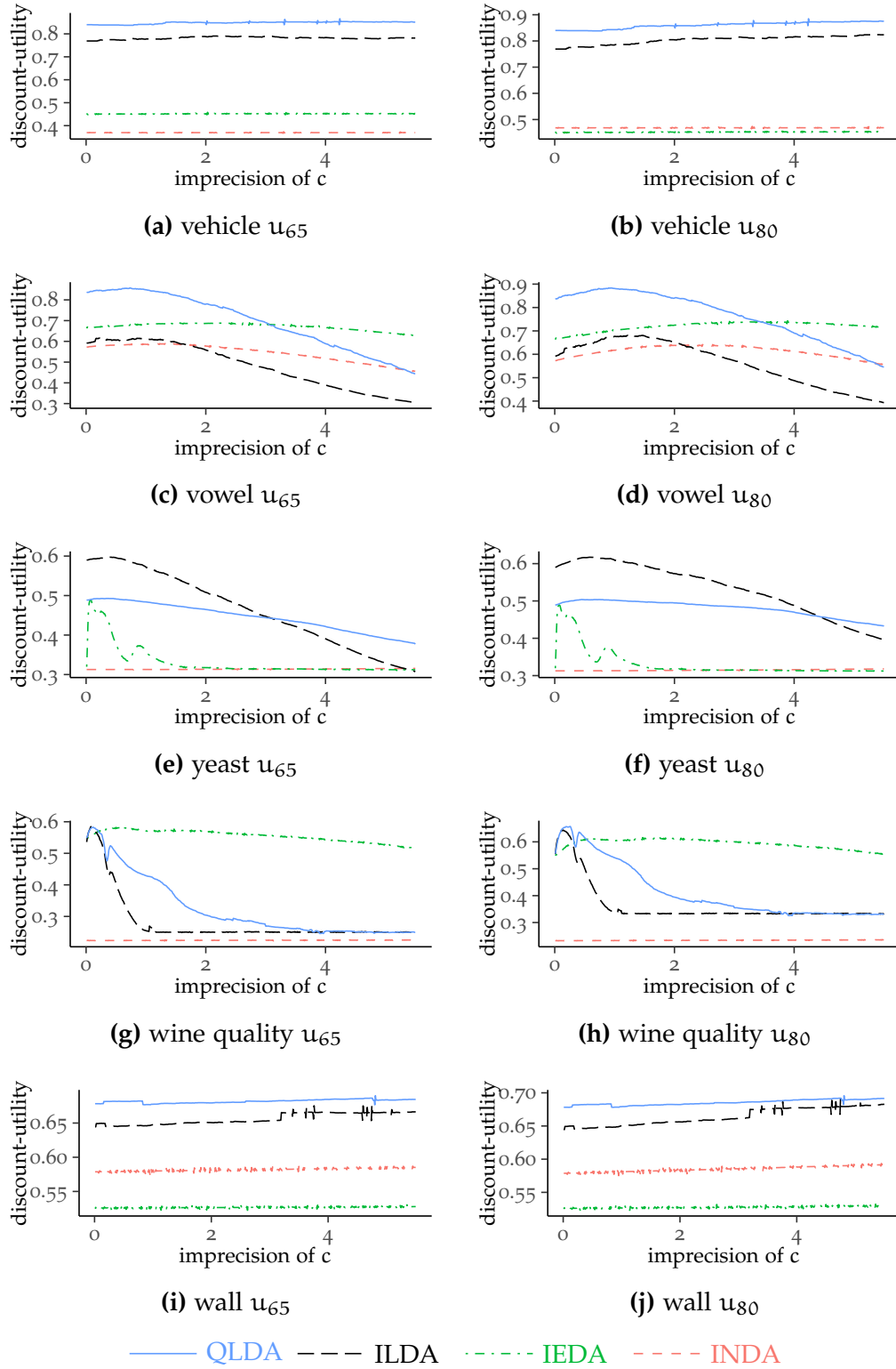
Figure A.3: Experiments for IGDA model (left:utility-discount u_{65} , right:utility-discount u_{80} )
