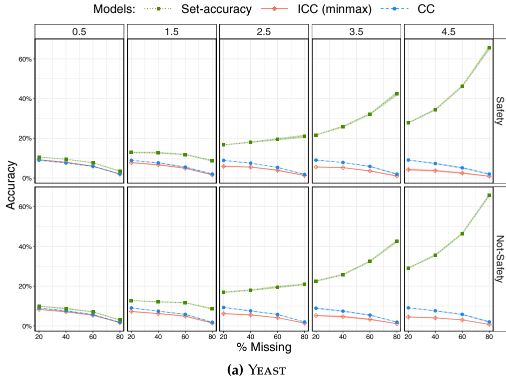
Figure B.14: Flipping - ICC versus CC - Marginalization. continuation of Figure B.13
