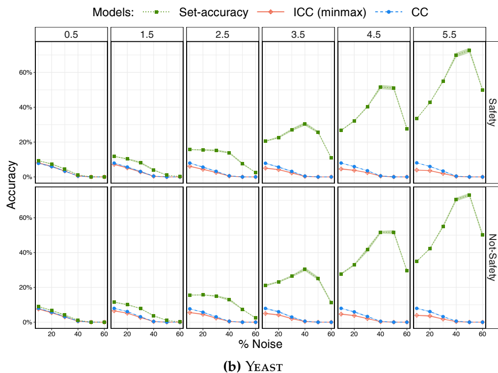
Figure B.10: Missing - ICC versus CC - Marginalization. continuation of Figure B.9
