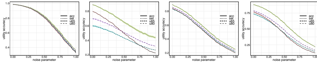
(c) (Imprecise) Naive discriminant analysis
