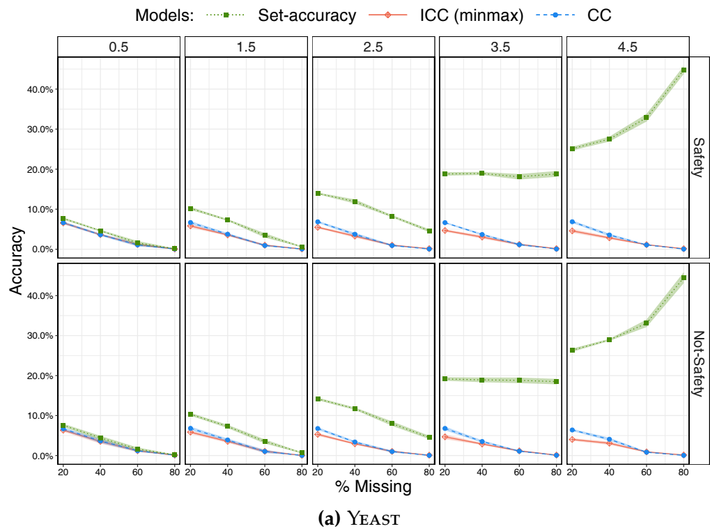
Figure B.18: Flipping - ICC versus CC - Marginalization. continuation of Figure B.17
