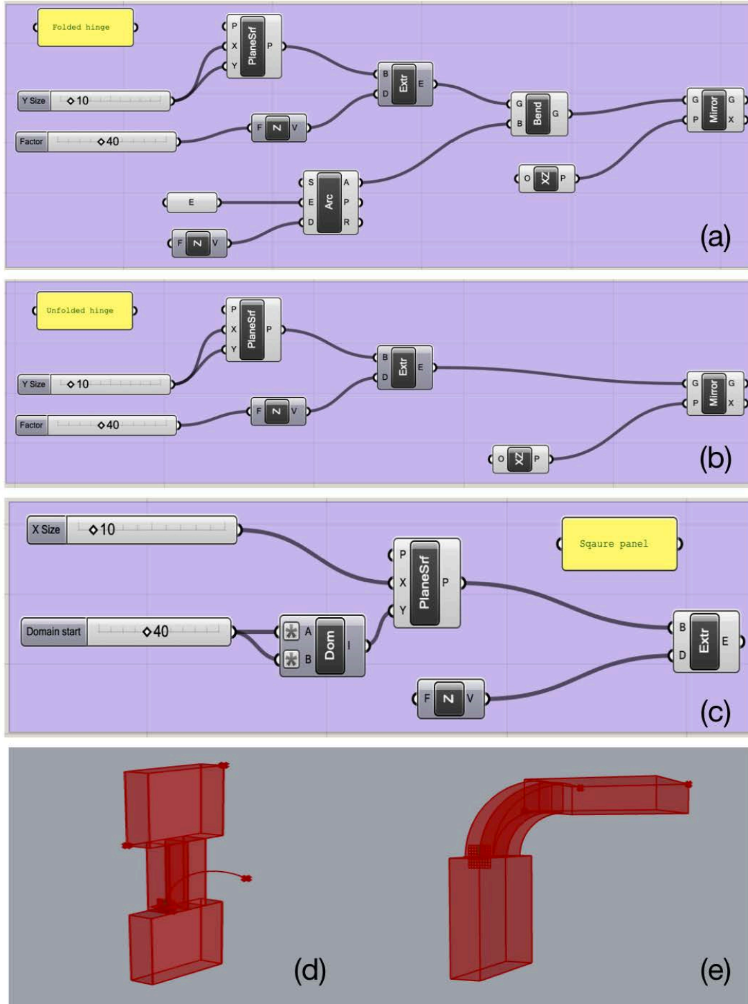
Figure. 58 Design flow and parameter setting in Grasshopper of (a) folded hinge, (b) unfolded hinge, (c) square panel. And the simulation result of (d) non-active and (e) active hinges
