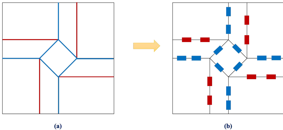
Figure. 53 (a) State A with crease pattern representation (b) State A with hinge layout representation
