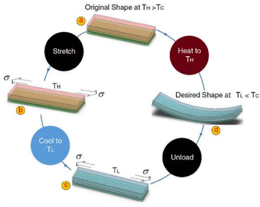
(a) Constrained-Thermo-Mechanics
