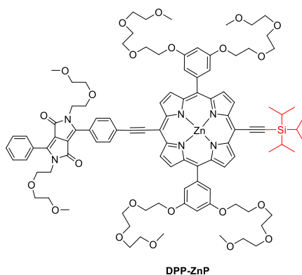
Figure 36. Structure du PS DPP-ZnP .
