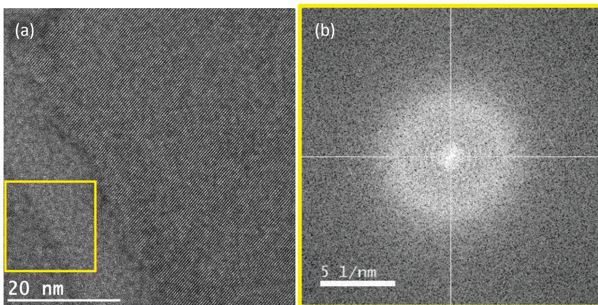
Figure 4.20: HRTEM image of a) matrix lattice fringes and amorphous silicon rich phase; b) Fast Fourier transformation (FFT) of the amorphous Si phase.
