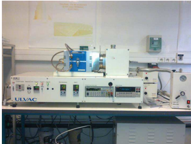
Figure 2.18: ZEM-3 machine.
