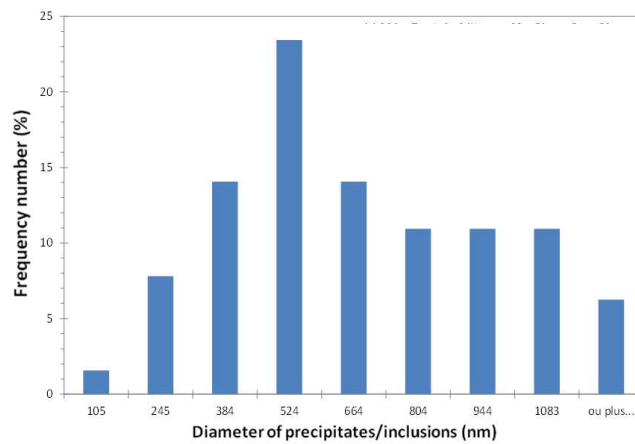
Figure 4.14: Grain size distribution of the optimized Mg_2Si_{0.3875}Sn_{0.6}Sb_{0.0125} material with 1.7 vol.% MgCuSn.
