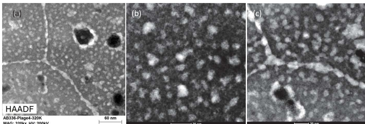
Figure 4.15: STEM/HAADF images of dark nodules and bright precipitates/inclusions concentrated in the grains and at the grain boundaries.
