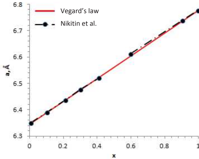
Figure 2.3: Curve of lattice constant vs. the mole fraction x for Mg_2Si_{1-x}Sn_x solid solution (adapted from Nikitin et al. [68] and Rowe [71]).
