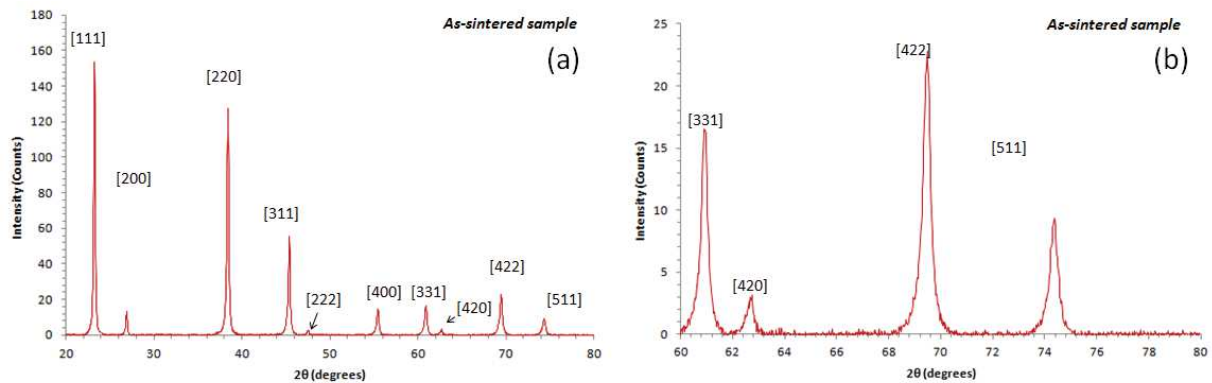
Figure 5.3: XRD spectrum on Mg_2Si_{0.38}Sn_{0.6}B_{0.02} as-sintered sample: (a) Complete spectrum; (b) Zoom on the high diffraction angle values.
