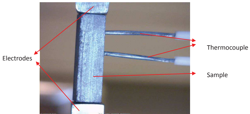
Figure 2.19: Placement of the specimen in the ZEM3 and important parts.
