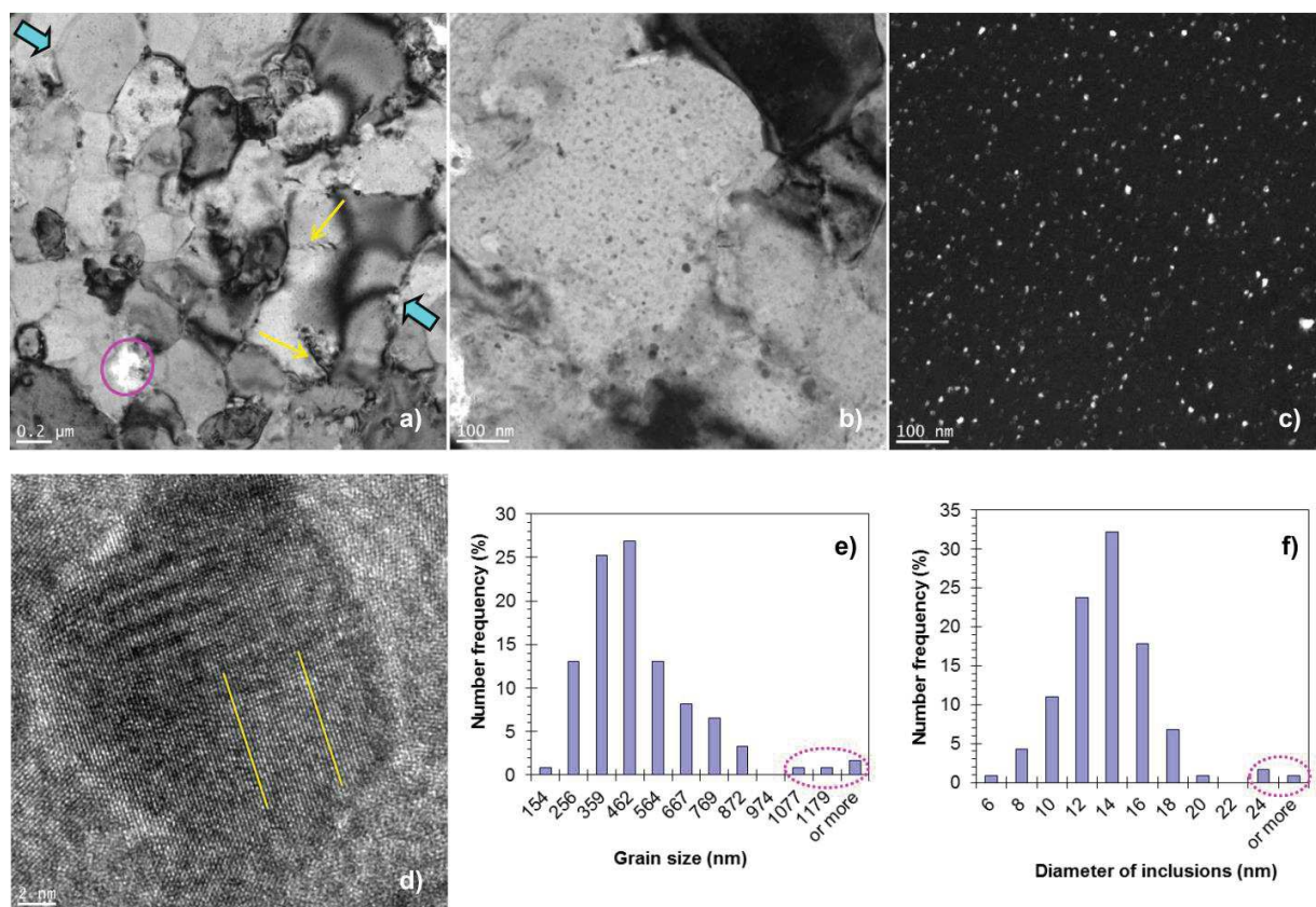
Figure 3.4: Typical microstructure of the as-sintered sample: (a) general view; (b) detailed view in bright field mode showing very small inclusions; (c) dark field image where most inclusions in the field are illuminated; (d) HRTEM image on an inclusion; (e) grain size distribution in the as-sintered material; (f) inclusions diameter distribution.
