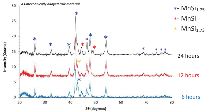
Figure 5.8: XRD patterns of as-mechanically alloyed MnSi_{1.75} alloy with milling times of: 6 hours (blue); 12 hours (red); 24 hours (black).
