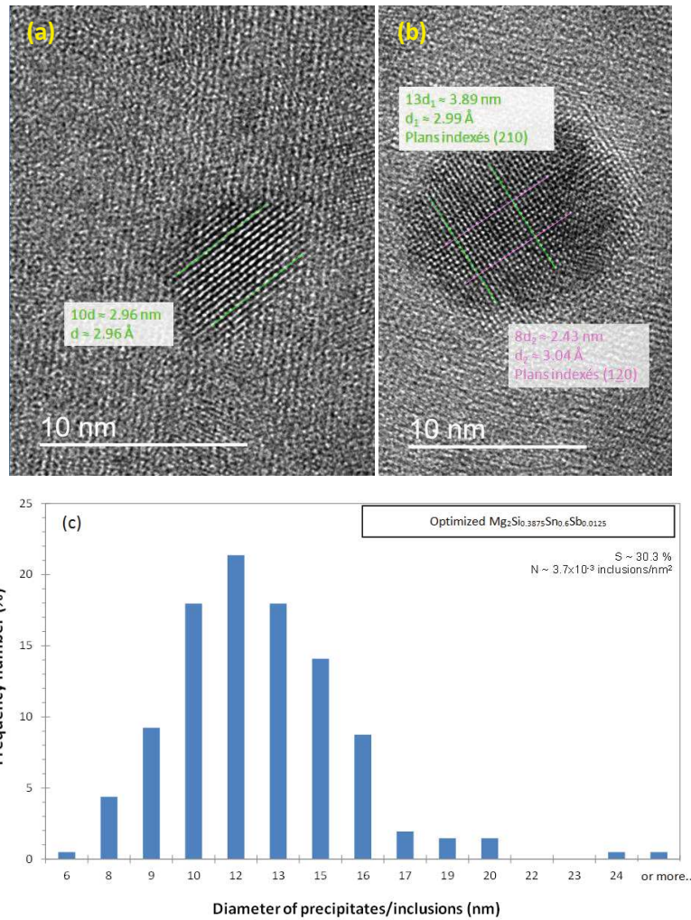
Figure 4.6: HRTEM pictures of precipitates/inclusion and their size distribution in optimized \text{Mg}_2\text{Si}_{0.3875}\text{Sn}_{0.6}\text{Sb}_{0.0125} .
