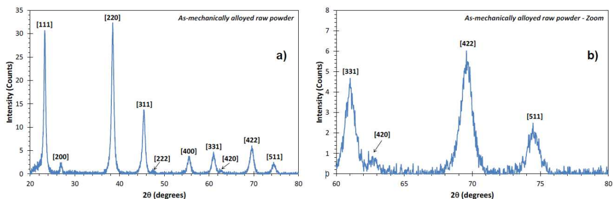
Figure 3.1: XRD spectra on the as-mechanically alloyed raw powder: (a) Complete spectrum; (b) Zoom on the high diffraction angle values for the as-mechanically alloyed powder.
