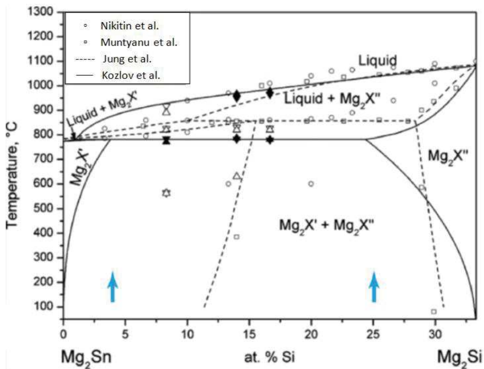
Figure 2.1: Binary Mg_2Si - Mg_2Sn phase diagram as it was reported by Muntyanu et al. [67], Nikitin et al. [68], Jung et al. [69], and Kozlov et al. [70] (figure adapted from [70]).
