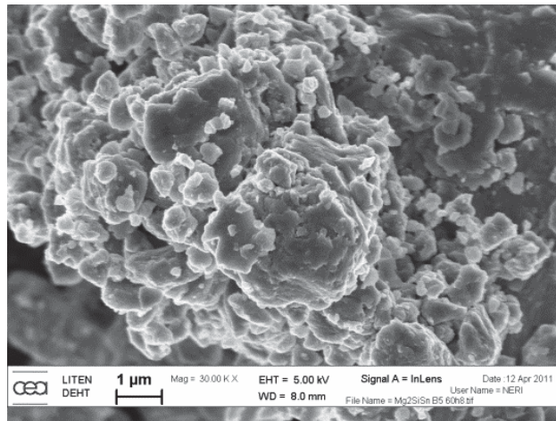
Figure 5.2: SEM image of the boron doped Mg-Si-Sn powder.
