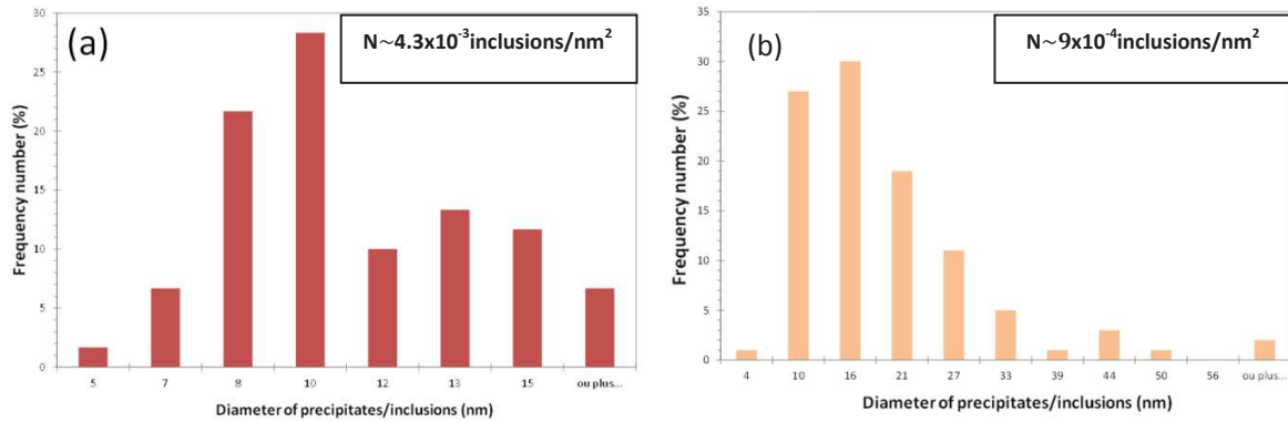
Figure 4.18: Optimized Mg_2Si_{0.3875}Sn_{0.6}Sb_{0.0125} material with 1.7 vol.% MgCuSn. Size distribution of: a) precipitates/inclusions; b) oxide-based nodules.
