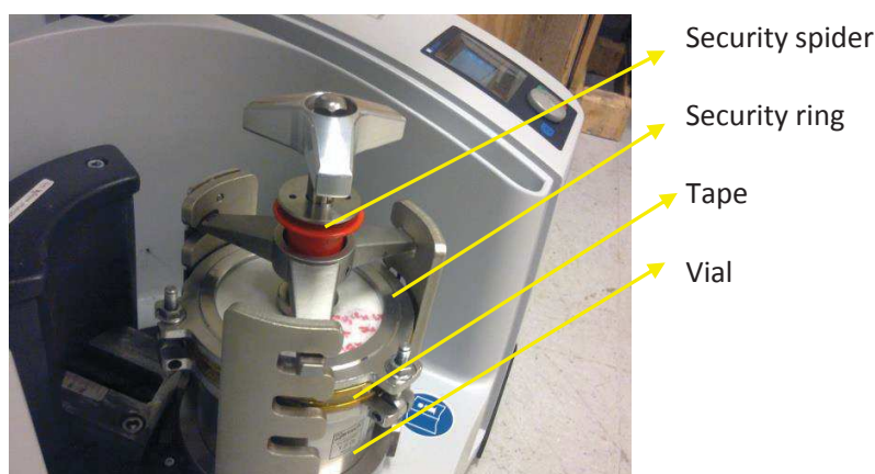
Figure 2.7: Planetary ball mill – RETSCH PM200.
