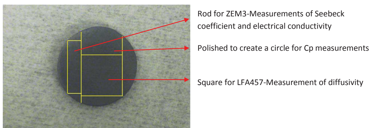
Figure 2.16: Cutting of the samples for measurements.
