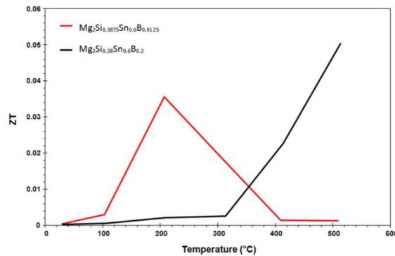
Figure 5.7: Thermoelectric figure of merit (ZT) in function of temperature.
