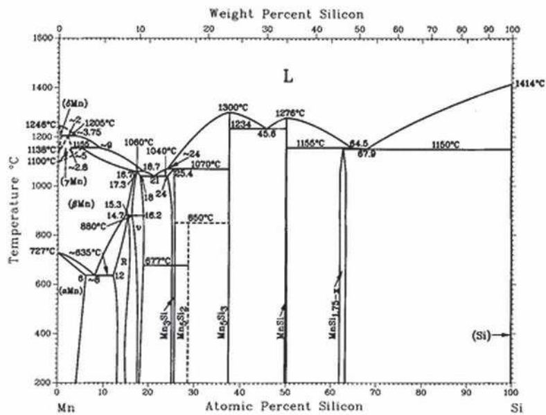
Figure 2.4: Assessed Mn-Si phase diagram (adopted from A.B. Gokhale [72]).
