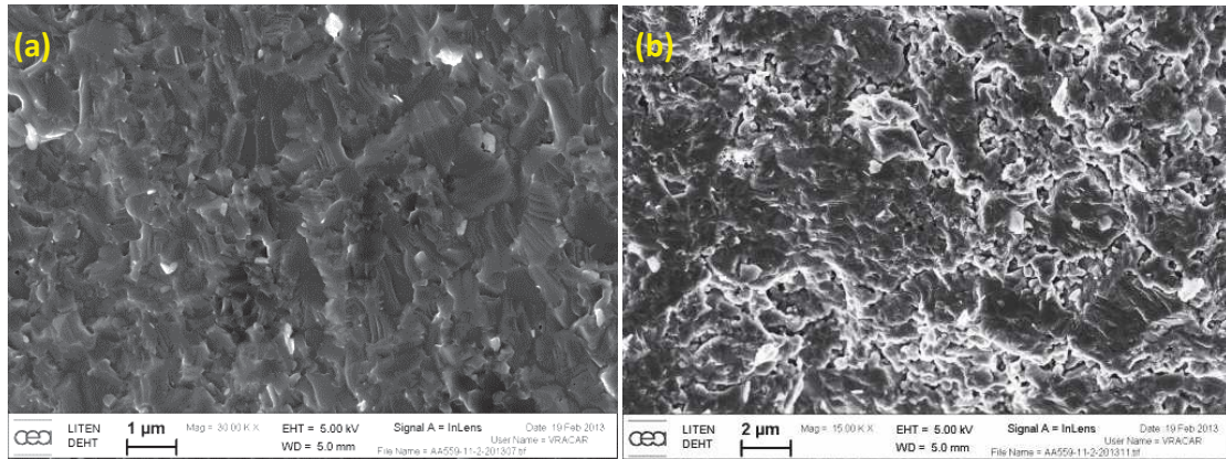
Figure 5.5: Fracture surface of both as-sintered samples: a) Mg_2Si_{0.38}Sn_{0.6}B_{0.02} ; b) Mg_2Si_{0.3875}Sn_{0.6}B_{0.0125} .
