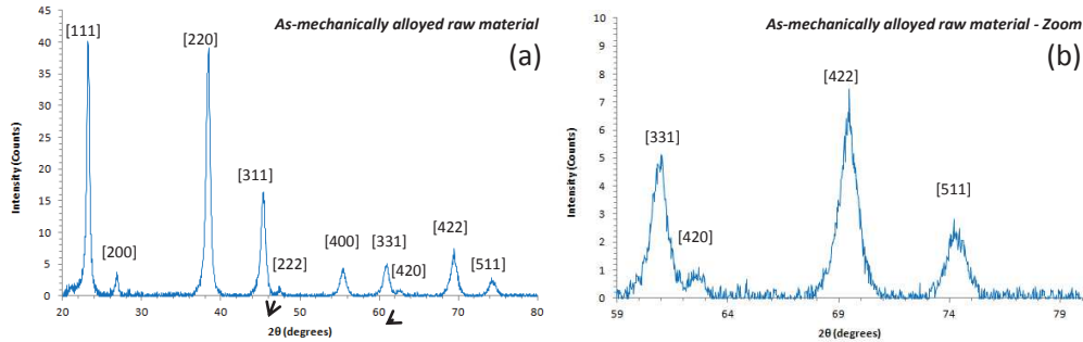
Figure 5.1: XRD spectrum on Mg_2Si_{0.38}Sn_{0.6}B_{0.02} as-mechanically alloyed raw powder: (a) Complete spectrum; (b) Zoom on the high diffraction angle values.
