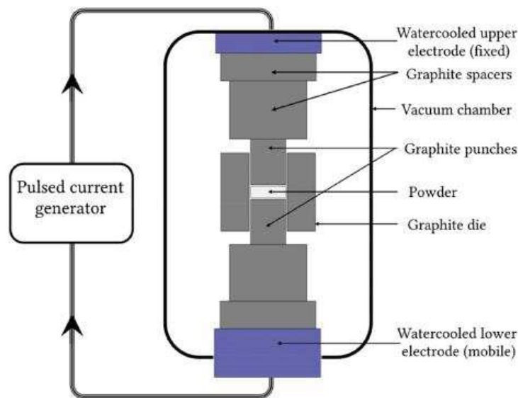
Figure 2.12: Scheme of SPS.
