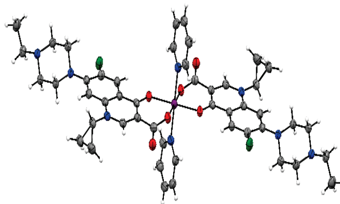
Figure I16: [Zn(ern)_2(py)_2].6H_2O^{57}
