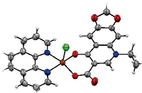
Figure I15: [Cu(oxo)(phen)Cl]^{56}
