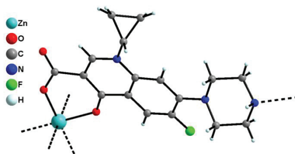
Figure III 24 : Structure du complexe [(Zn(Q2)(H_2O))].3H_2O
