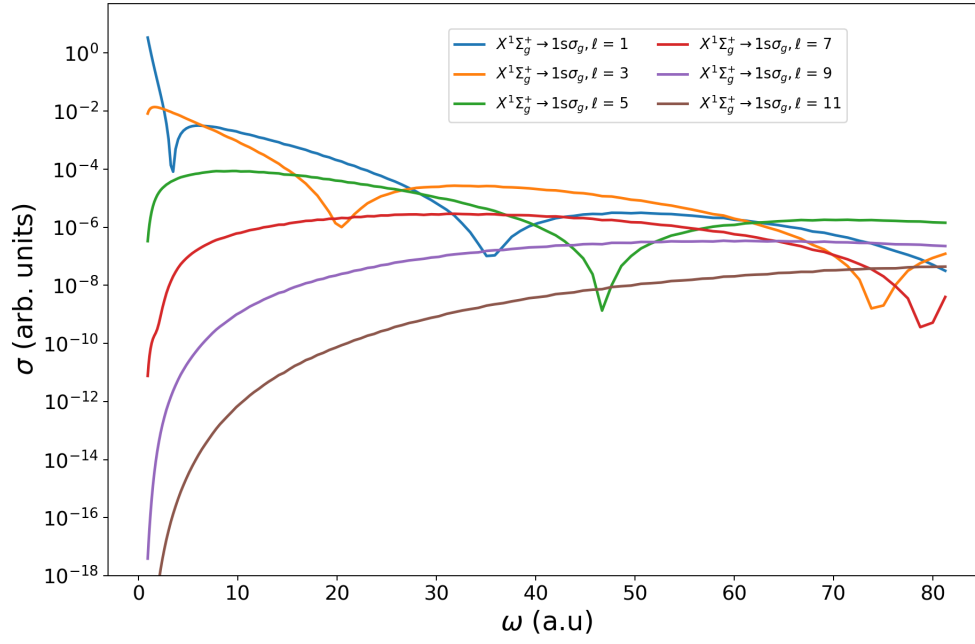
FIGURE 5.3 – Contribution from the first six partial waves to the partial photoionization cross-section to the 1\Sigma_u^+(1\sigma_g) continuum from the ground state of H_2 as a function of photon energy.
