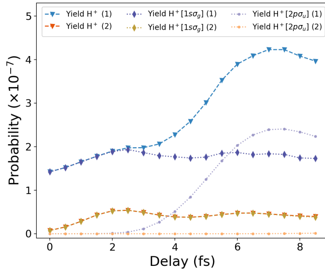
FIGURE 4.3 – Calculated H^+ yields as a function of the delay between the unfiltered (1) and filtered (2) APT, and the probe with their corresponding contributions from the ionic states 1\sigma_g and 2p\sigma_u .
