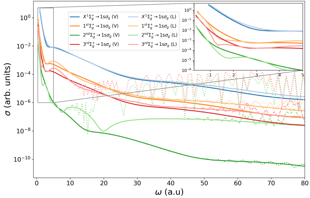
FIGURE 5.2 – Partial photoionization cross-section to the 1\Sigma_u^+(1s\sigma_g) continuum from the ground state and the first three excited states of symmetry 1\Sigma_g^+ of H_2 as a function of photon energy. The dark colors represent results from calculations in velocity gauge (labeled with V), while the corresponding light colors do so for calculations in length gauge (labeled with L). Results from calculations using 1001 (dotted line), 2002 (dashed line), and 3003 (solid line) points to solve the bi-electronic integrals from equation 1.25 are shown.
