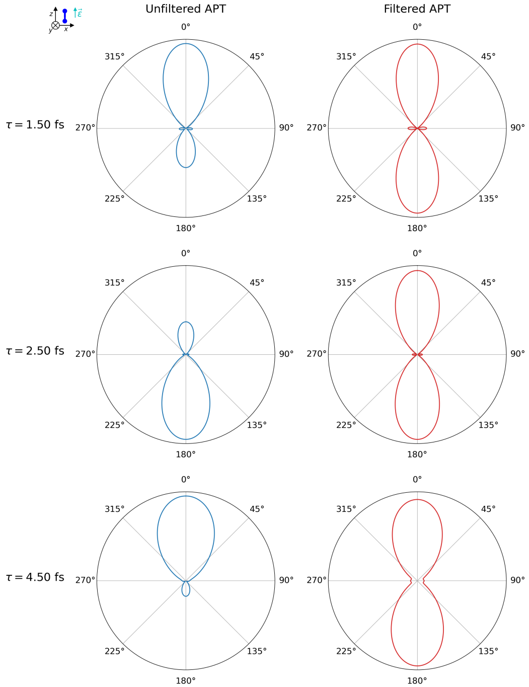
FIGURE 4.10 – 2D-projected MFPADs in the z-o-x plane for dosociative ionization of H_2 with EKE=0.5 eV and NKE=0.2 eV for a pump-probe scheme with an unfiltered (left panels) and filtered (right panels) APT. Each row corresponds to different delays of the probe with respect to the APT.
