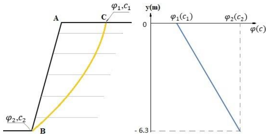
Figure 2-19 Variation of the friction angle with depth in the backfill
