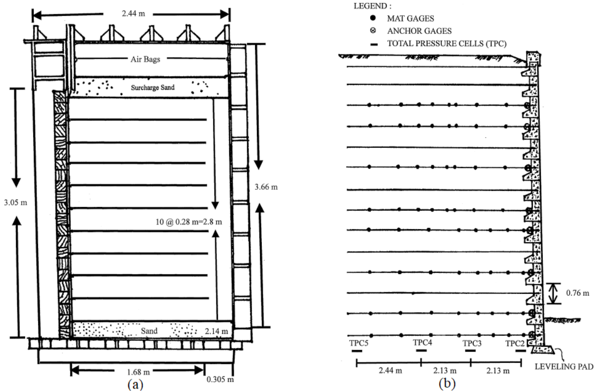
Figure 1-18 (a) University of Colorado wall (Wu, 1991); (b) Large-scale wall test conducted by Sampaco (1996)
