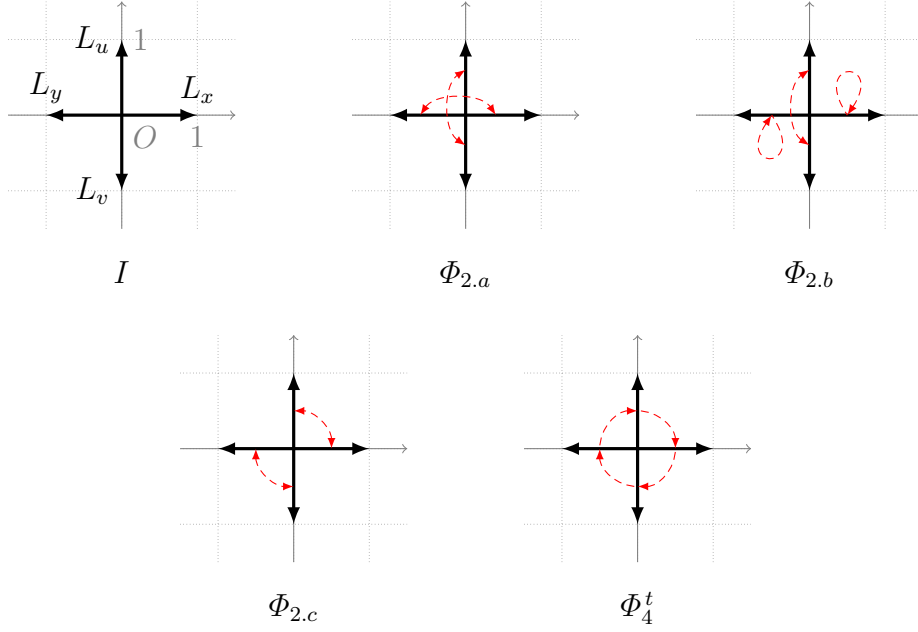
Figure 7.3: Actions on primitive vectors of the fan \Sigma_{\mathcal{H}}
