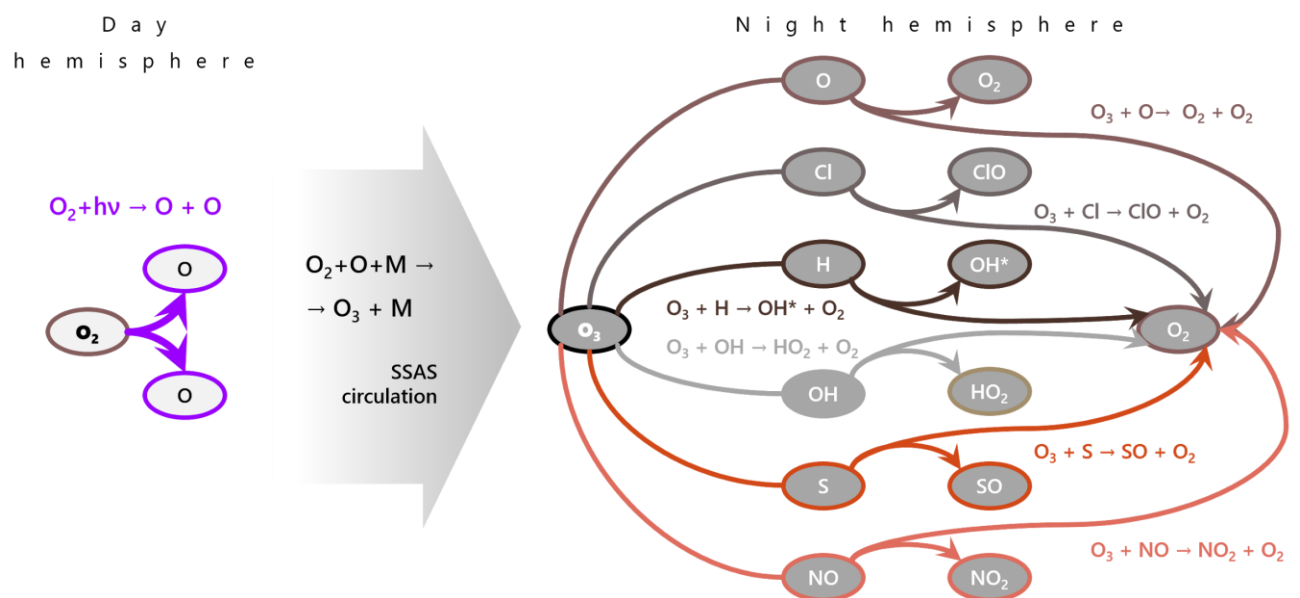
Figure 2.9. The main reactions of the ozone chemical cycle including its source and formation (left) and the main sinks (right).
