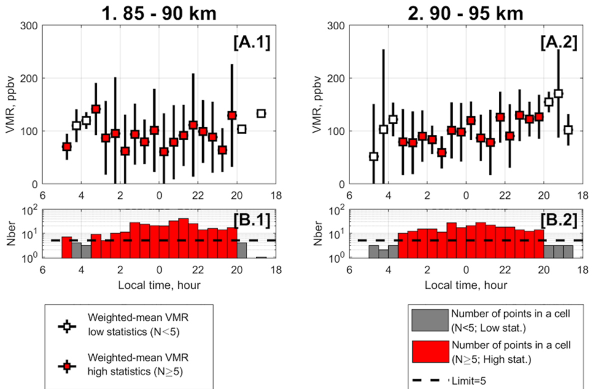
Figure 4.13. A1 and A2: Weighted-mean SO 2 VMR variations with local time for two altitude ranges of 85-90 km (1) and 90-95 km (2). The data are binned by 30 min of local time. Red and white square bins with statistical dispersions include \geq 5 and < 5 individual points respectively. The B panels represent the number of individual points for one bin. Black dashed lines in the histograms correspond to the level of 5 points.
