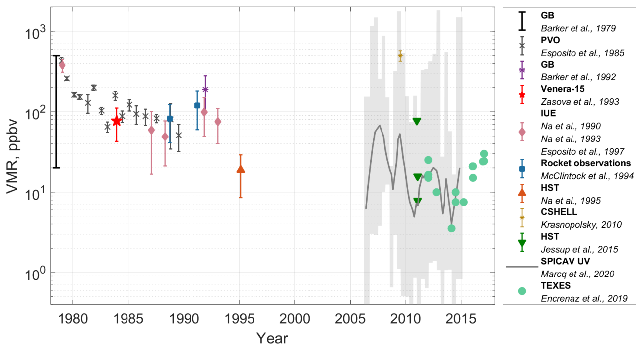
Figure 2.1. The timeline of sulphur dioxide observations at the cloud tops on the day side of Venus. The references are given in the legend. The SPICAV UV observations are presented with the corresponding variability of obtained values within 4-month intervals. The full range of obtained values is represented by the grey area which is accompanied by a median curve (grey solid line).
