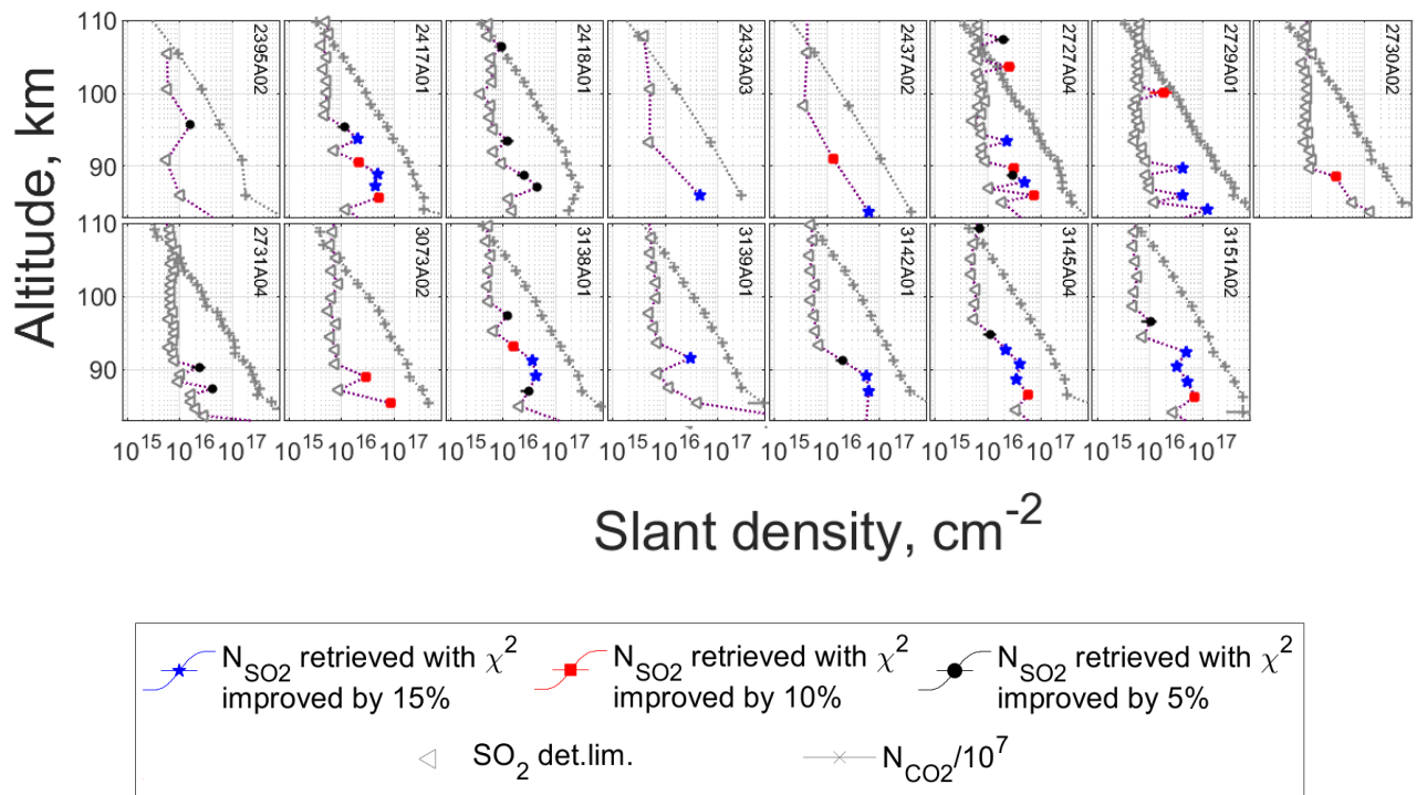
Figure A1.1. Individual slant density profiles of carbon and sulphur dioxides in 83-110 km and the SO 2 detection limit values corresponding to the SO 2 negative detections. The decrease of \chi^2 in cases of the SO 2 detection is marked by different colors.
