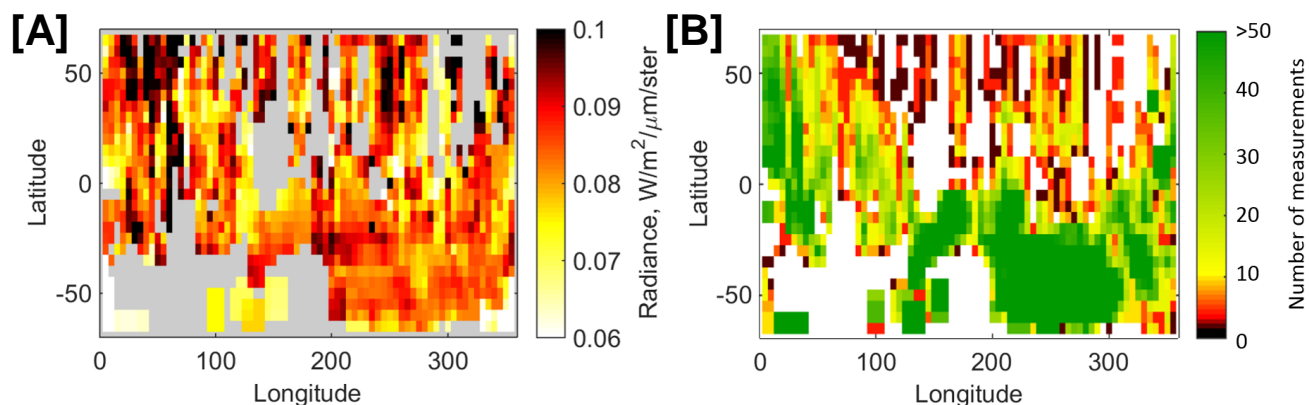
Figure 6.2. (A) Geographic distribution of radiation intensity in a transparency window of 1.28 \mu\text{m} obtained with emission angle \leq 10^\circ . The map is averaged within bins of 5^\circ \times 5^\circ . (B) The number of observations in each bin (Evdokimova et al., 2016).
