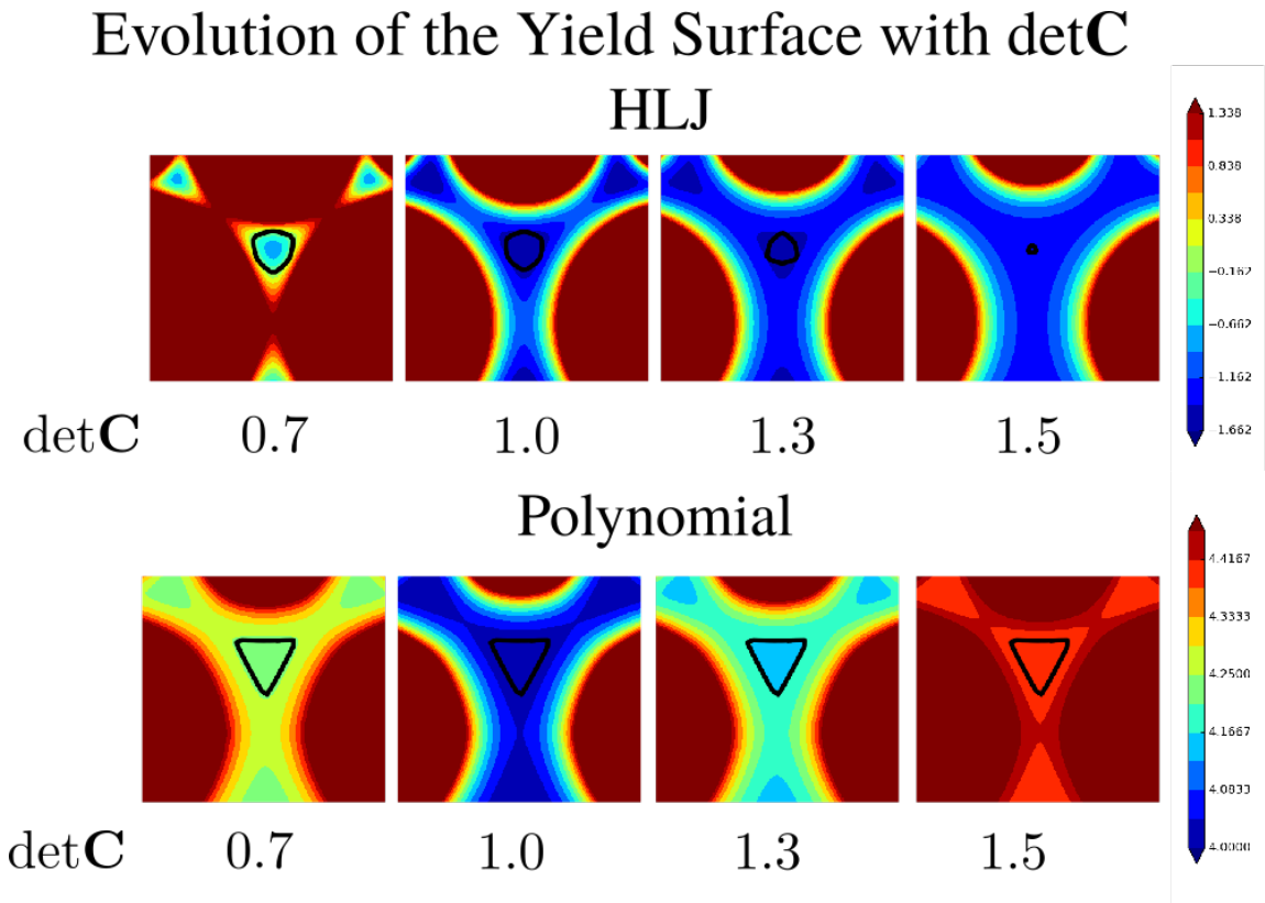
Figure 5.7: Dependence on \det \mathbf{C} of the Yield Surface: Evolution of the stability region, that we called yield-surface , is shown for the Polynomial and the HLJ energy. The peculiar response to tension in the HLJ energy causes the progressive shrinking of its stability region, up to a complete disappearance.
