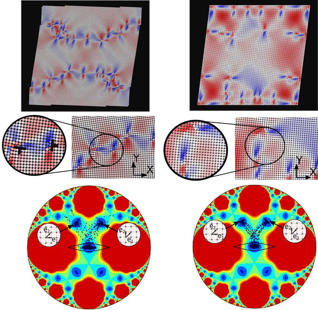
Figure 4.8: Post-Instability Pattern for the Rhombic Pure Shear: Results are shown for a N = 10^4 domain with both periodic (left) and fixed (right) boundaries. On top: the Cauchy stress \sigma_{xy} is shown in the full domain with evidence on two edge dislocations. On bottom: The element points in the configurational space. Wells \mathbf{S} , \mathbf{S}_1^{0^\circ} , and \mathbf{S}_{-1}^{90^\circ} are simultaneously activated. The points on the valleys connecting these wells correspond to the elements in the dislocation core.
