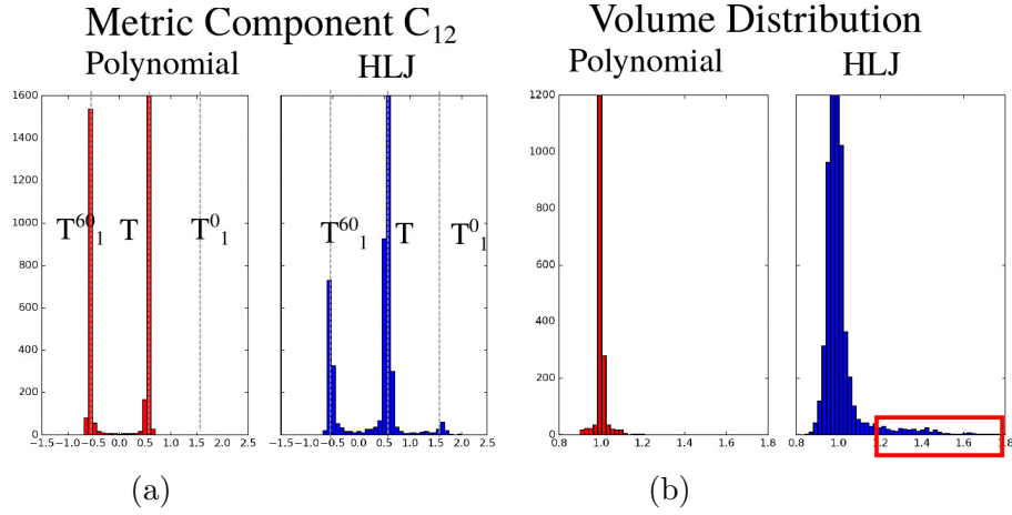
Figure 5.4: Histograms of Metric Component C_{12} and of Elements Volume: (a) Distribution of metric component C_{12} show that T_1^{60} , of metric C_{12} = -0.5774 , is the most active well (other than reference well T , with metric component C_{12} = 0.5774 ) for both polynomial and HLJ energies. (b) Distribution of elements volume, the great majority of elements preserve their volume (unitary), but HLJ shows the presence of few elements whose volume is very high. Histogram y-axis has been cut to better visualize the distribution.
