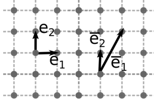
Figure 2.3: Bravais Lattice: Schematic representation of a simple, Bravais, lattice. It is fully described by an integer basis \{\mathbf{e}_I\} which, periodically translated in space, defines the lattice. Choices for the integer basis \{\mathbf{e}_I\} are infinite, but all these basis are in relation by the action of the global symmetry group GL(2, \mathbb{Z}) .
