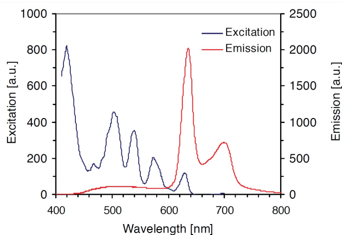
Figure 1.5 – Excitation and emission spectra of PpIX [52].
