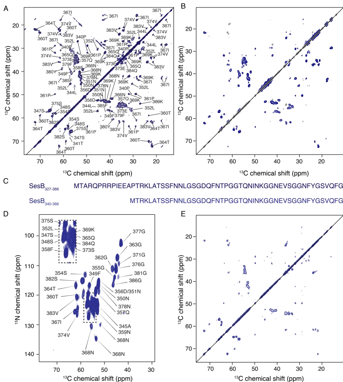
Figure 2-4: SesB 328-386 and SesB 340-386 share a similar rigid amyloid fold comprising ~50 residues. (A) 2D ^{13}\text{C} - ^{13}\text{C} PDSD with a 50 ms-mixing time displaying intra-residual correlations of SesB 328-386 (peak assignments are shown). (B) 2D ^{13}\text{C} - ^{13}\text{C} DREAM spectrum recorded on SesB 328-386 fibrils and exhibiting the most rigid amino acids. (C) Primary sequences of SesB 328-386 and SesB 340-386 . (D) 2D ^{13}\text{C} - ^{15}\text{N} projection of a 3D ^1\text{H} - ^{13}\text{C} - ^{15}\text{N} hCANH of perdeuterated and ^1\text{H} -back-exchanged SesB 340-386 fibrils (peak assignments are shown). (E) 2D ^{13}\text{C} - ^{13}\text{C} PDSD with a 50 ms-mixing time displaying intra-residual correlations of SesB 340-386 which shows a spectral fingerprint very similar to that of SesB 328-386 . The 2D spectra were recorded on an 800 MHz (proton frequency) using a 11 ( i.e. , PDSD) or 18 ( i.e. , DREAM) kHz MAS and a 3.2 mm probe (3-day experiments), and the 3D spectrum was recorded on a 900 MHz spectrometer (proton frequency) using a 60 kHz MAS and a 1.3 mm probe (1-day experiment)
