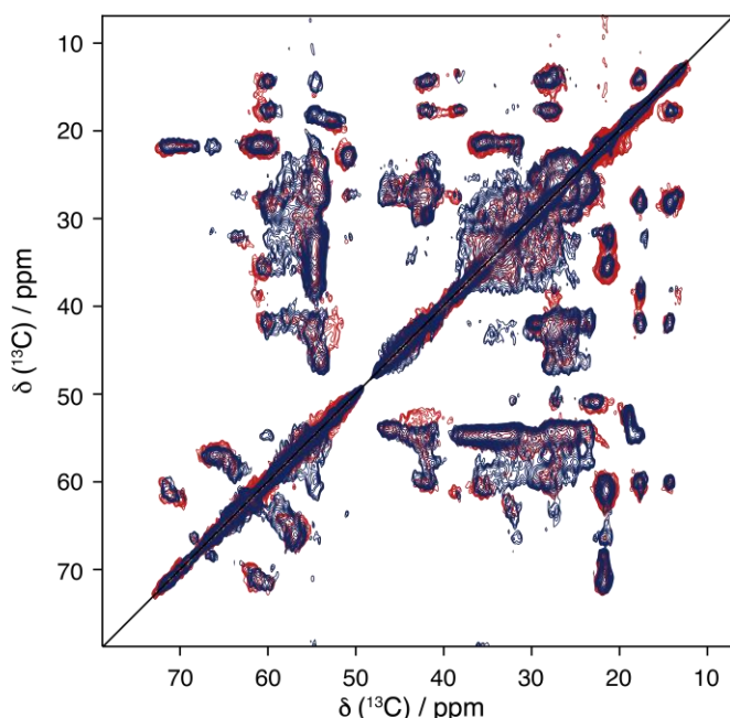
Figure 5-8: Superposition of 2D ^{13}\text{C} - ^{13}\text{C} PDSD spectra with a 50 ms mixing time using a 600 MHz spectrometer (proton frequency) of PrgJ(1-101) in dark red and PscI(1-112) in dark blue.
