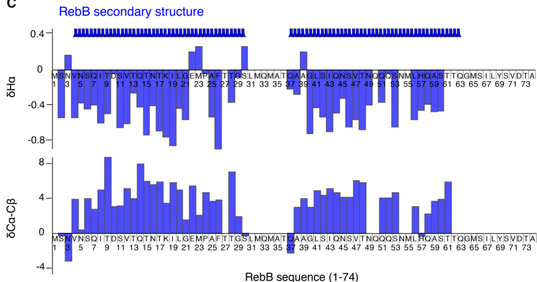
Figure 6-3: (A) Sequence alignment of RebA, RebB (generated with Clustal, and represented with Jalview). For clarity purposes, the assigned residues shown in the Figure 2A are highlighted in bold characters. (B) \delta(C\alpha-C\beta) , \delta H\alpha and secondary structure of assigned residue in RebA (142). (C) \delta(C\alpha-C\beta) , \delta H\alpha and secondary structure of assigned residue in RebB (142).
