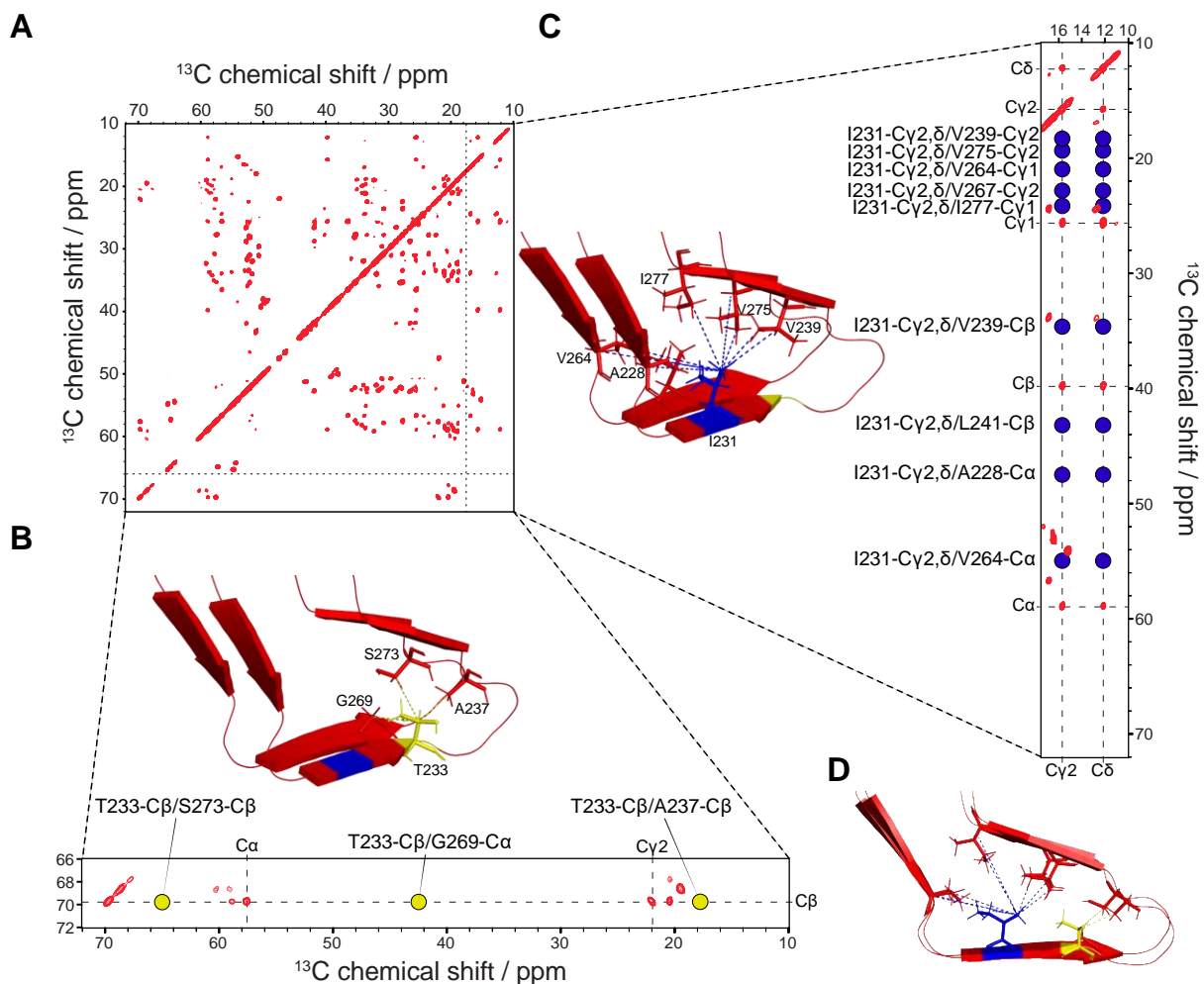
Figure 0-4: Illustration of long range through-space distance determination, based on HET-s(218-289) amyloid core (55). (A) 2D- ^{13}\text{C} - ^{13}\text{C} PDS spectrum (50ms mixing time) of HET-s(218-289) uniformly labelled ( ^{13}\text{C}/^{15}\text{N} ) recorded on a 800MHz spectrometer (proton frequency). (B) Excerpts of the PDS spectrum shown in A, displaying only threonine correlations. T233 resonances are highlighted with dashes (C \alpha , C \beta , C \gamma 2). Reported distances regarding T233 are displayed with yellow dots and illustrated on the HET-s(218-289) structure (PDB ID: 2RNM). (C) Excerpts of the PDS spectrum shown in A, (ppm window: 10-17.5). I231 resonances are highlighted with dashes (C \alpha , C \beta , C \gamma 1, C \gamma 2, C \delta ). Reported distances regarding I231 are displayed with blue dots and illustrated in HET-s(218-389) structure (PDB ID: 2RNM). For clarity purposes, overlapping peaks were disregarded. (D) HET-s structure (55), as shown in B-C, from a lateral point of view. All mentioned distances were determined based on either PDS long-mixing time experiments (with [2-^{13}\text{C}] - or [1,3-^{13}\text{C}_2] -glycerol labelling schemes), or CHHC spectra (with a fully labelled HET-s amyloid core sample).
