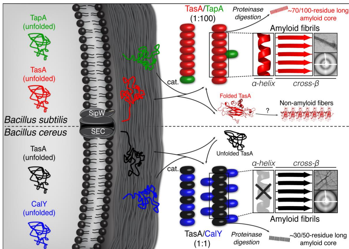
Figure 3-10: The current understanding of the mechanisms involved in TasA/CaIY/TapA secretion and Bacillus biofilm formation in both B. subtilis and B. cereus .
