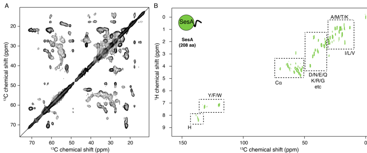
Figure 2-7: The partner protein SesA displays a similar 13 C- 13 C spectral fingerprint in its assemble form suggesting a common structural arrangement. (A) 2D 13 C- 13 C PDSD with a 50 ms-mixing time displaying short-range 13 C- 13 C correlations of SesA 1-208 fibrils' rigid core. (B) 2D 1 H- 13 C J-based INEPT displaying flexible segments of SesA 1-208 fibrils, probably accounting for the globular unstructured part.
