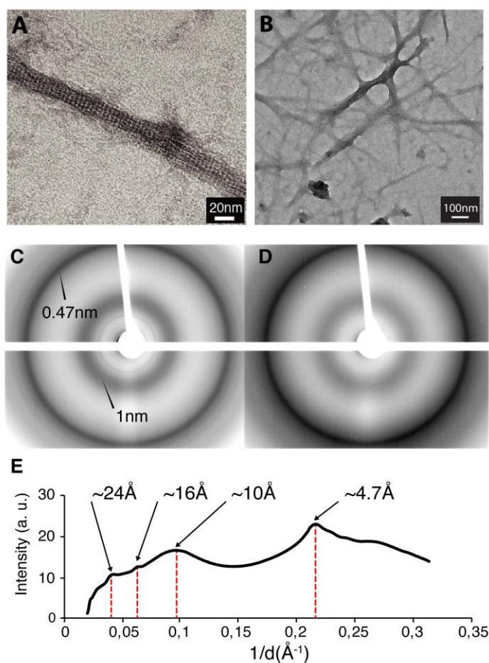
Figure 3-4: Transmission electron micrographs of negatively stained B. subtilis TasA (A) and B. cereus TasA amyloids (B). The average TasA-bs filament width was ~5 nm. X-ray diffraction patterns of TasA-bc functional amyloids (C) (reflections at ~4.7 Å and ~10 Å are highlighted) and TasA-bs functional amyloids (D). (E) Diffraction intensity plot of TasA-bc filaments, diffraction signals at 24, 16, 10 and 4.7 Å are highlighted.
