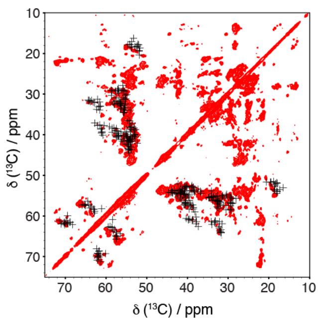
Supplemental Figure 3-4: Comparison of SSNMR 2D ^{13}\text{C} - ^{13}\text{C} correlation experiment (PDSD, 50 ms mixing time) of TasA-bs to chemical shift predictions.
