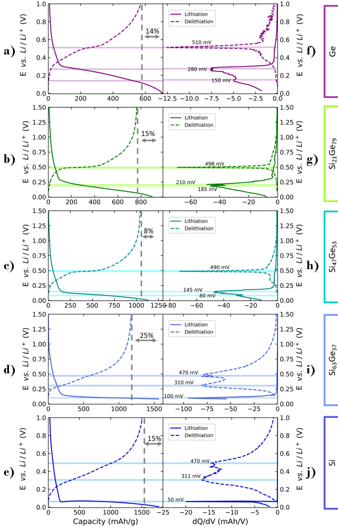
Figure 4.7 a-e) potential vs. \text{Li}/\text{Li}^+ against capacity f-j) voltage vs. \text{Li}/\text{Li}^+ as a function of dQ/dV for crystalline Ge, and the Ge-rich ( \text{Si}_{21}\text{Ge}_{79} ), Si \approx Ge ( \text{Si}_{47}\text{Ge}_{53} ), Si-rich alloys ( \text{Si}_{63}\text{Ge}_{37} ), and Si Nps in a coin-cell at C/20 against Li metal.
