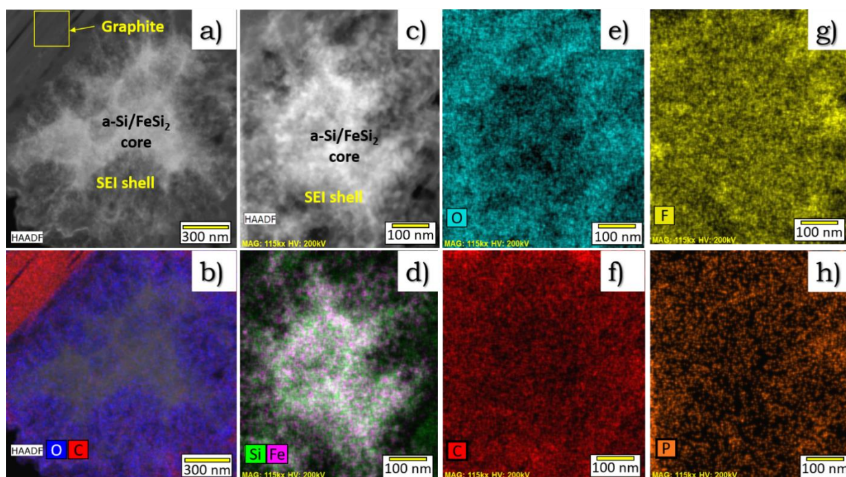
Figure 6.10 a) and c) HAADF image of the alloy particle and corresponding b) and d-h) chemical mapping of Si, Fe, F, O, C, and P elements for the 300 cycles a-Si/c-FeSi 2 /graphite electrode.
