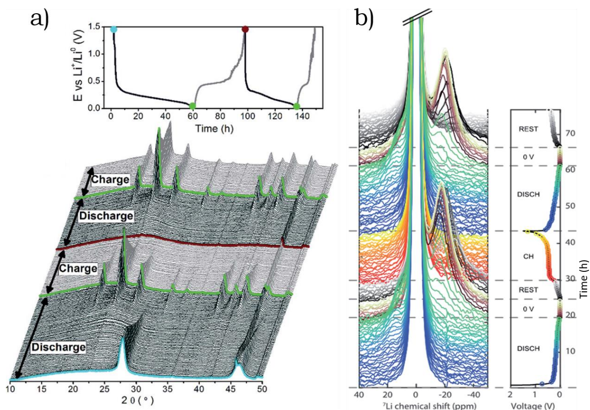
Figure 1.9 the electrochemical cycling of a c- \text{Si}_{0.5}\text{Ge}_{0.5} self-supported film vs. Li metal by a) Operando XRD. b) in-situ ^7\text{Li} NMR. Adapted from [70].
