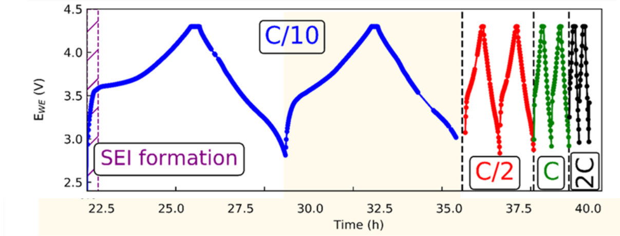
Figure 5.4 Electrochemical sequence applied to the fresh pouch cell at BM02. Evolution of the potential vs. time. The cell was cycled at several C-rates: C/10 (blue), C/2 (red), C (green), and 2C (black).
