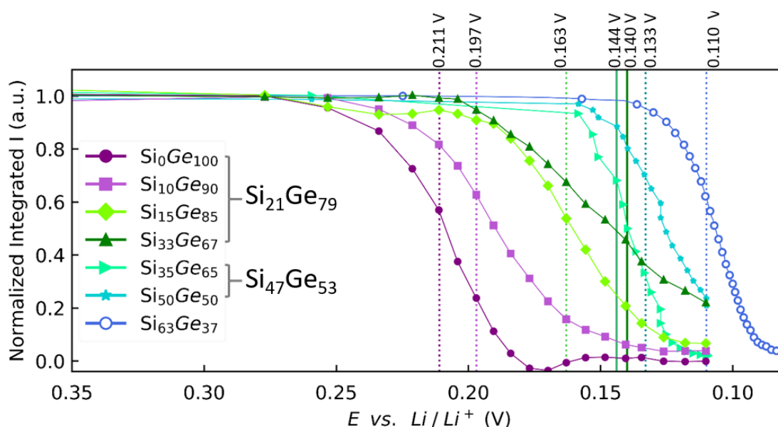
Figure 4.11 Normalized integrated intensity against voltage vs. \text{Li}/\text{Li}^+ during a complete lithiation for the distinct phases found in the three synthesized alloys.
