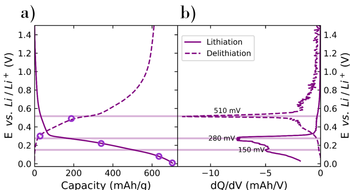
Figure 3.2 a) voltage vs. \text{Li}/\text{Li}^+ against the capacity of c-Ge Nps in a coin-cell. b) voltage vs. \text{Li}/\text{Li}^+ as a function of dQ/dV (the number of measured points for every voltage step) at C/10 during the first cycle. The points indicate the samples measure by post-mortem ^7\text{Li} -NMR.
