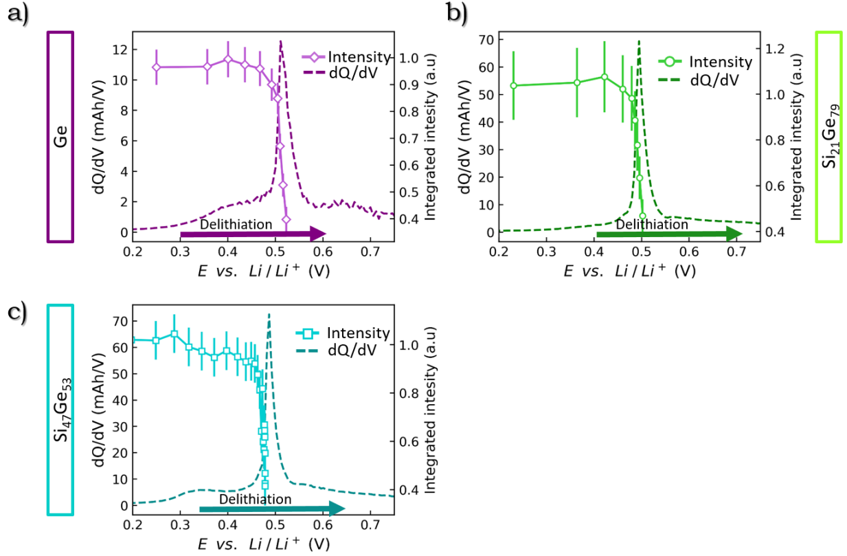
Figure 4.17 The dQ/dV graphs overlap the normalized integrated intensity for the (220) Bragg reflection of a) Li 15 Ge 4 obtained from pure Ge b) Li 15 (Si 100-x Ge x ) 4 obtained for Si 21 Ge 79 , and c) Si 47 Ge 53 .
