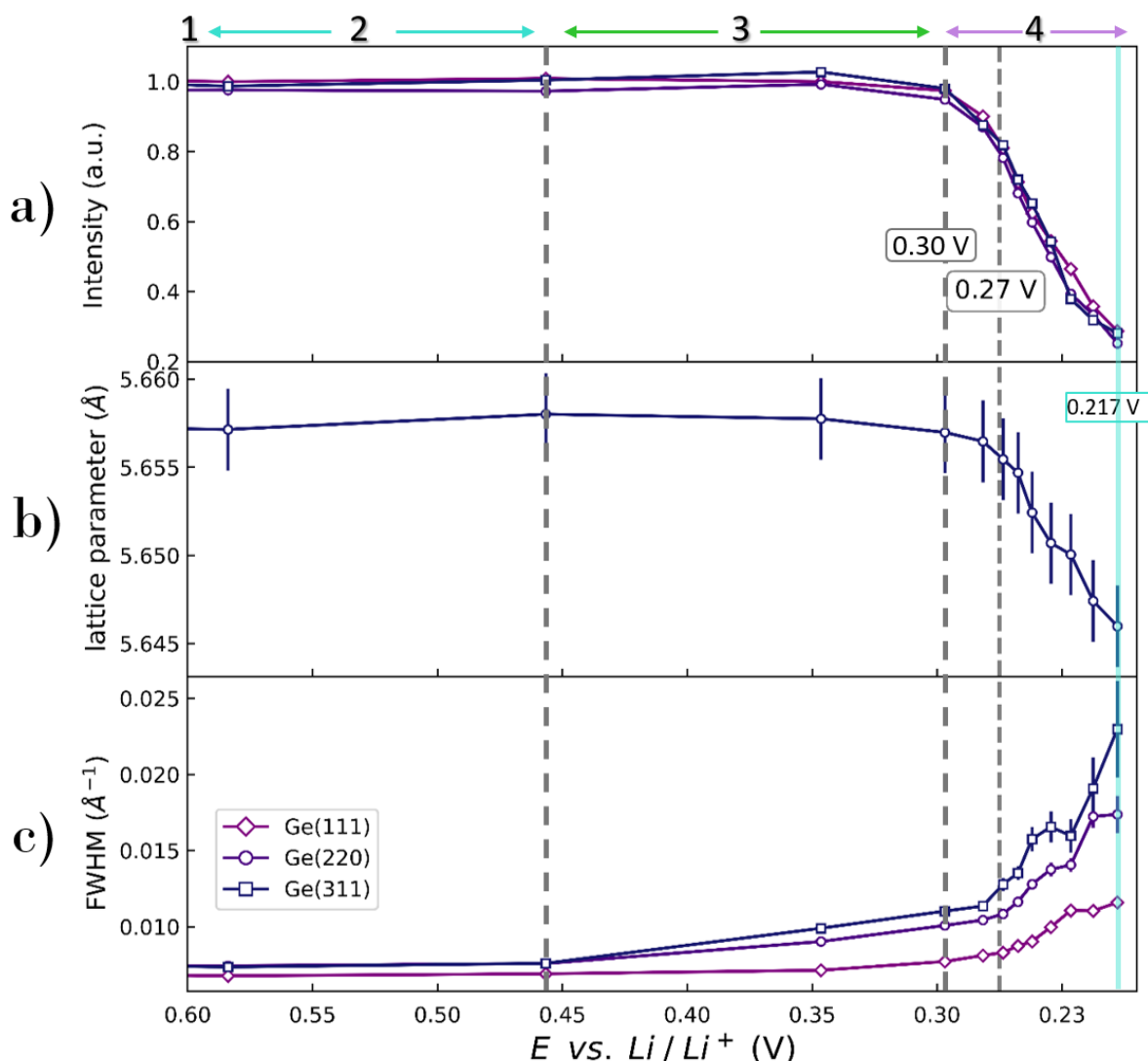
Figure 3.6 a) intensity, b) lattice parameter of Ge, and c) full widths at half maximum of the Ge(111), Ge(220), and Ge(311) reflections as a function of voltage vs. \text{Li}/\text{Li}^+ upon lithiation.
