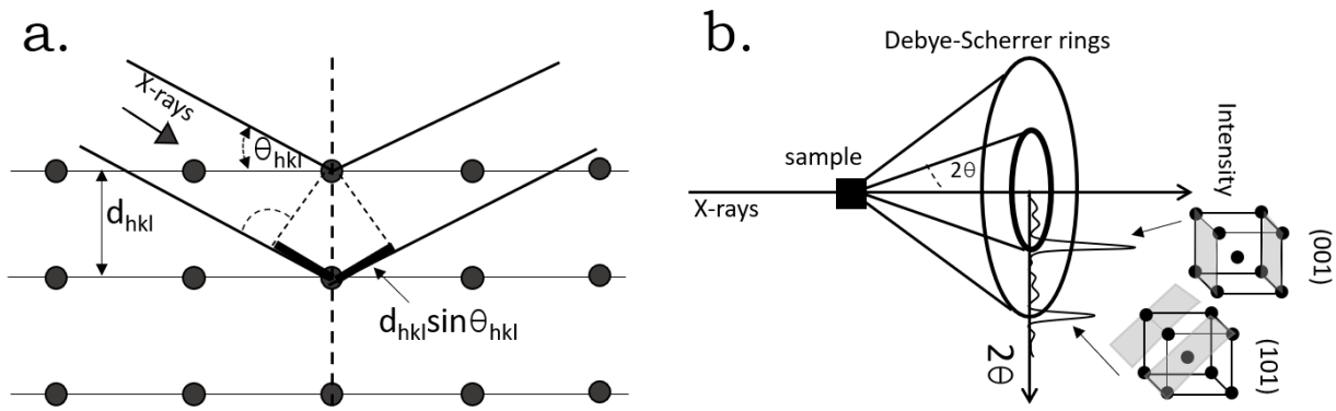
Figure 2.2. a. Illustration of the diffraction of X-rays by a crystal. b. Illustration of formation of a diffracted cone in the Debye-Scherrer geometry.
