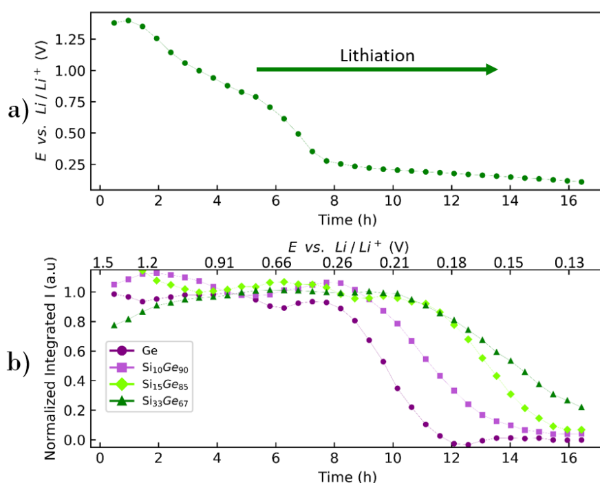
Figure 4.10 a) voltage vs. \text{Li}/\text{Li}^+ against time for the complete lithiation of the alloy with an average composition \text{Si}_{21}\text{Ge}_{79} . b) Normalized integrated intensity obtained from the fit of the distinct phases in \text{Si}_{21}\text{Ge}_{79} vs. time during a complete lithiation. Note that the secondary x-axis indicates the corresponding voltage.
