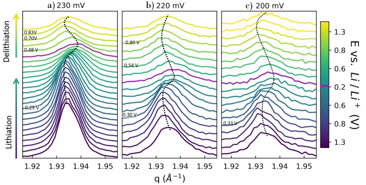
Figure 3.7 Evolution of the Ge(111) peak during the three partial lithiation down to a) 230, b) 220, and c) 200 mV.
