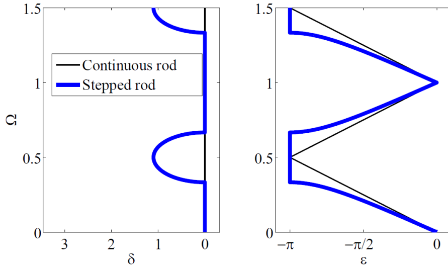
Figure 2.5 Dispersion diagram for a continuous rod and for a stepped rod.
