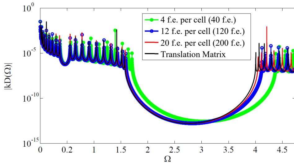
Figure 3.4 FRF convergence of finite element mesh to Translation Matrix model for a periodic beam with 10 cells.
