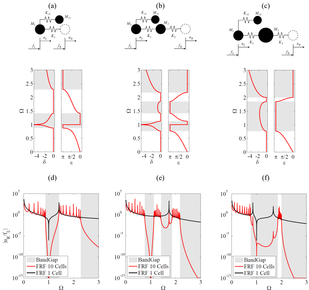
Figure 2.3 Dispersion diagrams for different unit cells: (a) case 4, (b) case 5, (c) case 6 and FRF amplitudes computed for 1 and 10 cells: (d) case 4; (e) case 5; (f) case 6.
