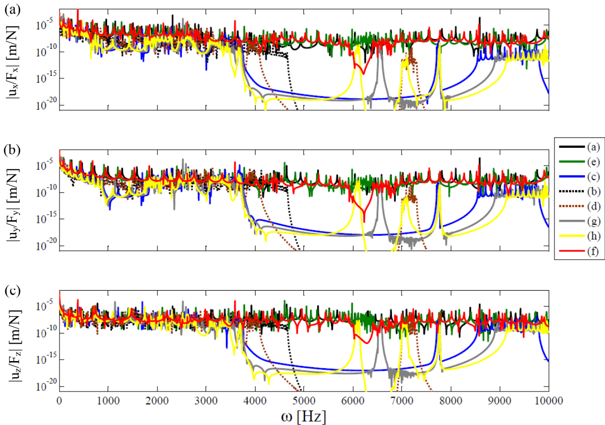
Figure 5.6 (a), (b) and (c) frequency responses of 8 scenarios periodic finite structures with 10 cells by exciting the first node on direction x, y and z and observing the corresponding dofs on the last unit cell.
