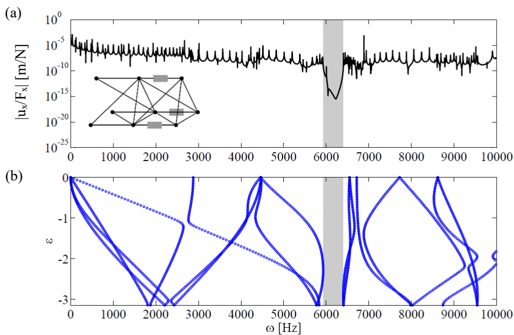
Figure 5.10 Band gap for (a) finite and (b) infinite structures considering the local resonance effect.
