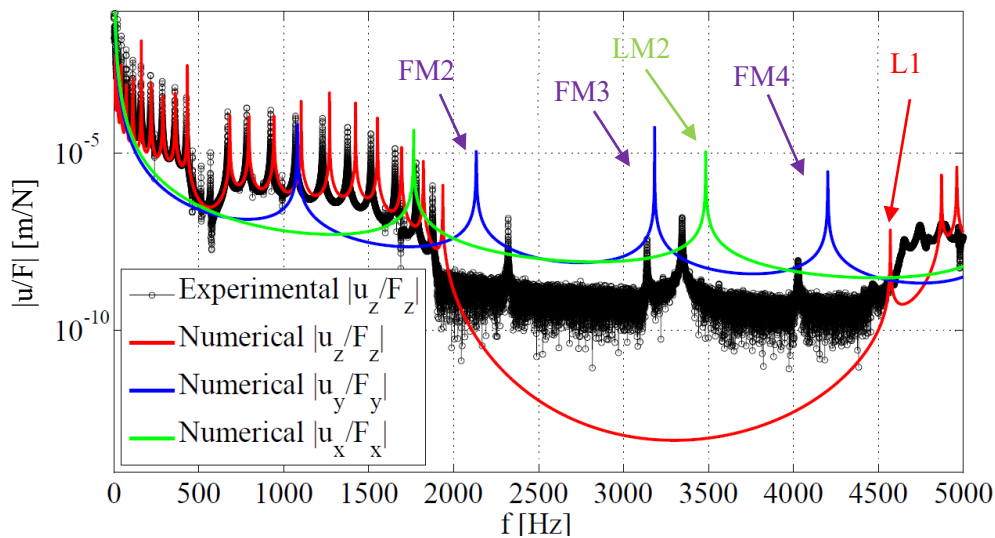
Figure 4.6 FRF with non-predicted resonance frequencies inside the attenuation zone.
