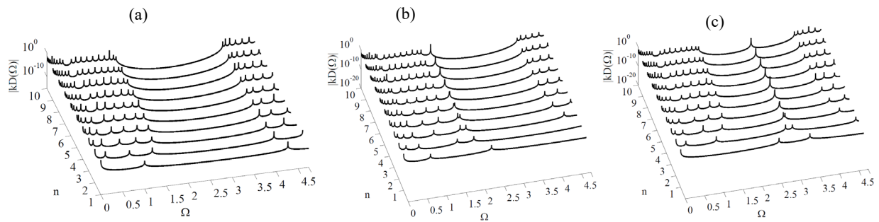
Figure 3.15 FRFs for convergence of cell number for: symmetric cases (a) and (b) and asymmetric case (c).
