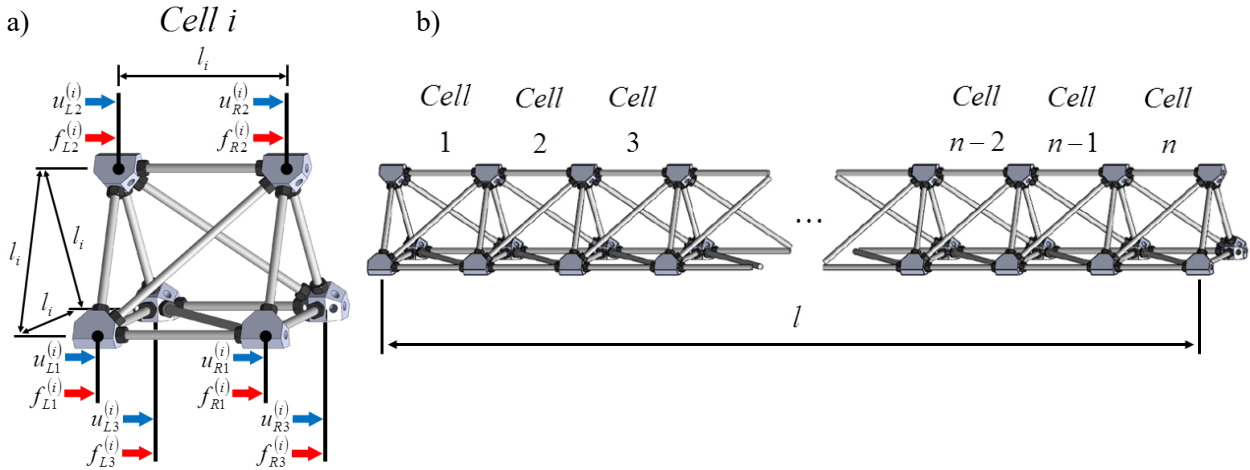
Figure 5.1 (a) 3D truss unit cell and (b) its finite model.
