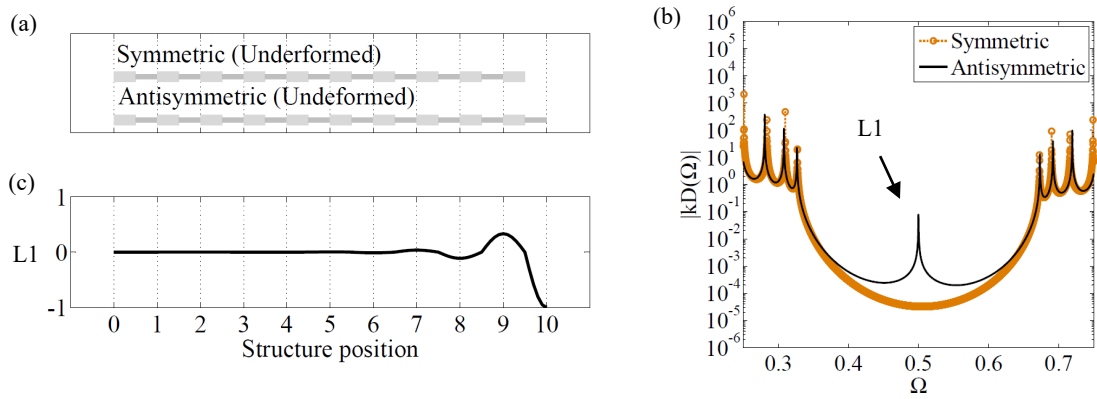
Figure 2.14 Comparison between (a) symmetrical and antisymmetrical structures, their (b) FRFs and (c) the shape of localized mode L1 for antisymmetrical one.
