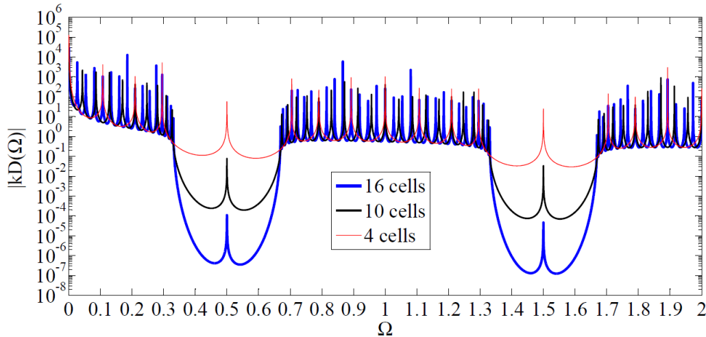
Figure 2.7 Frequency response functions for finite structures with various cell number.
