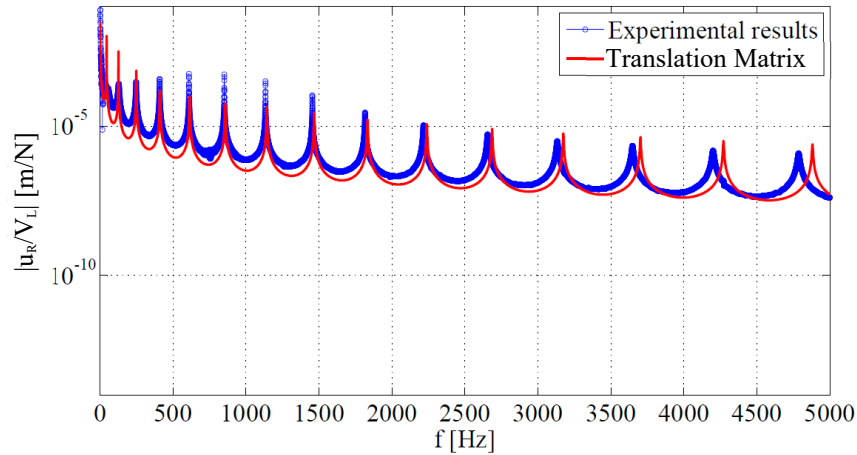
Figure 4.4 Frequency response function obtained experimentally for a free-free continuous beam.
