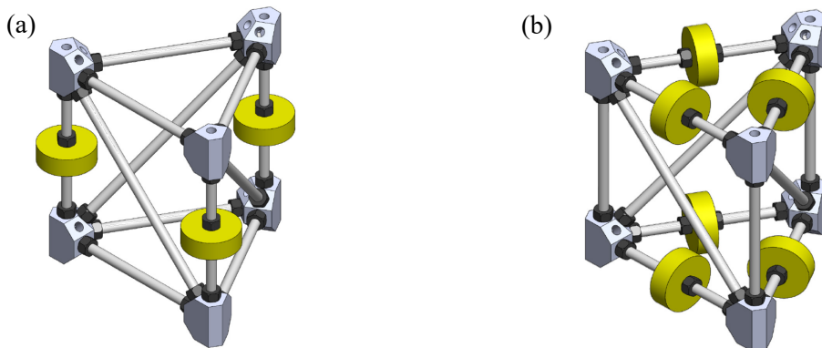
Figure 5.11 Example of truss unit cell with concentrated mass in the middle of (a) vertical and (b) horizontal bars to reduce frequency of inner resonances.
