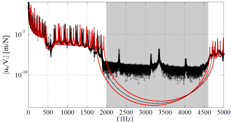
Figure 4.8 FRF with envelope confidence interval, experimental results and robust bandgap for calculated standard deviation.
