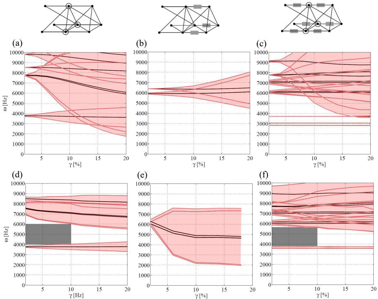
Figure 5.8 Bandgap bounds envelopes relatives to scenarios on Figures 5.3(c), 5.3(f) and 5.3(h), with: (a) mass as RV, (b) and (c) inductance as RV considering an infinite model (1 RV) with their corresponding (d), (e) and (f) for finite results with 10 RV.
