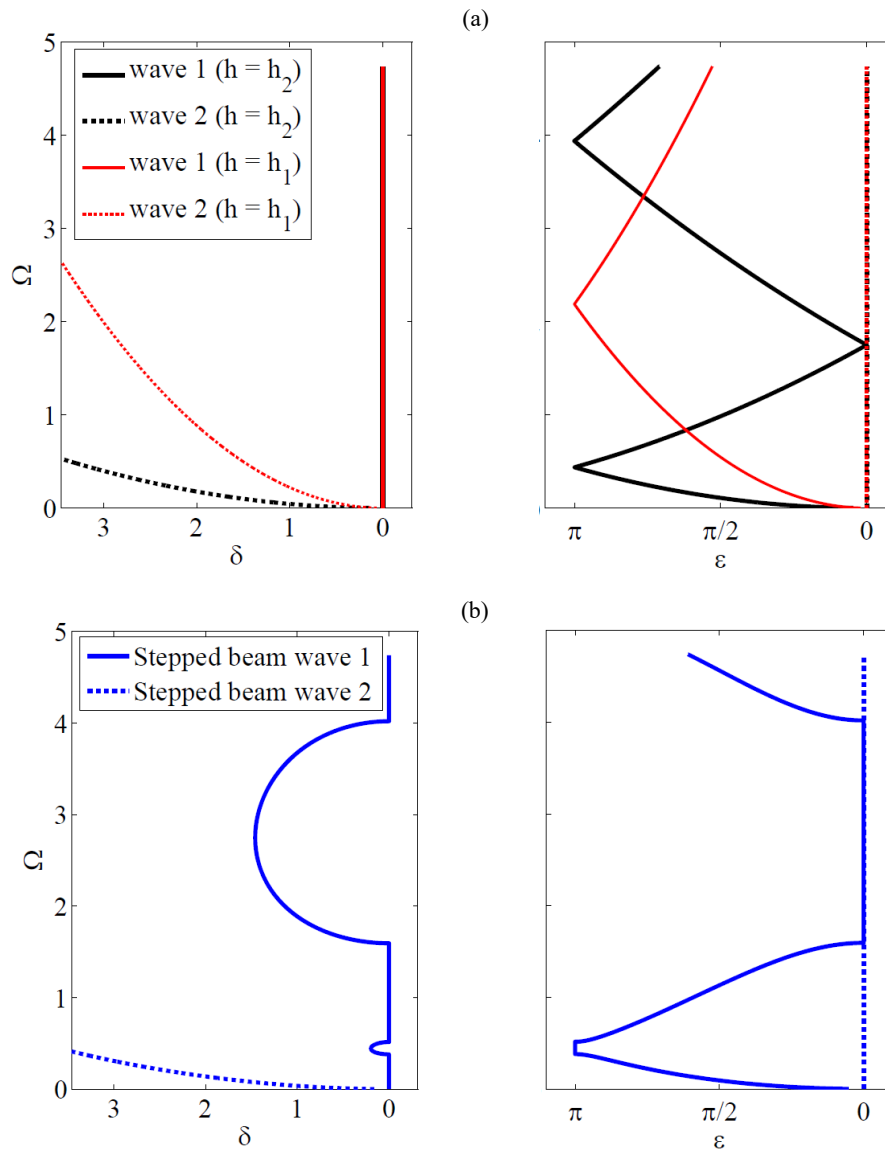
Figure 3.2 Dispersion constants considering flexural waves for (a) continuous beam and (b) stepped periodic beam.
