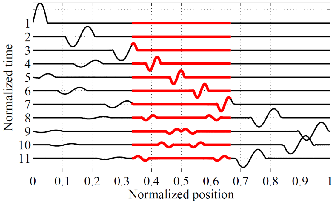
Figure 1.1 Wave propagating in a string with two density mismatches, in normalized positions 0.333 and 0.666, and fixed-fixed boundary conditions.
