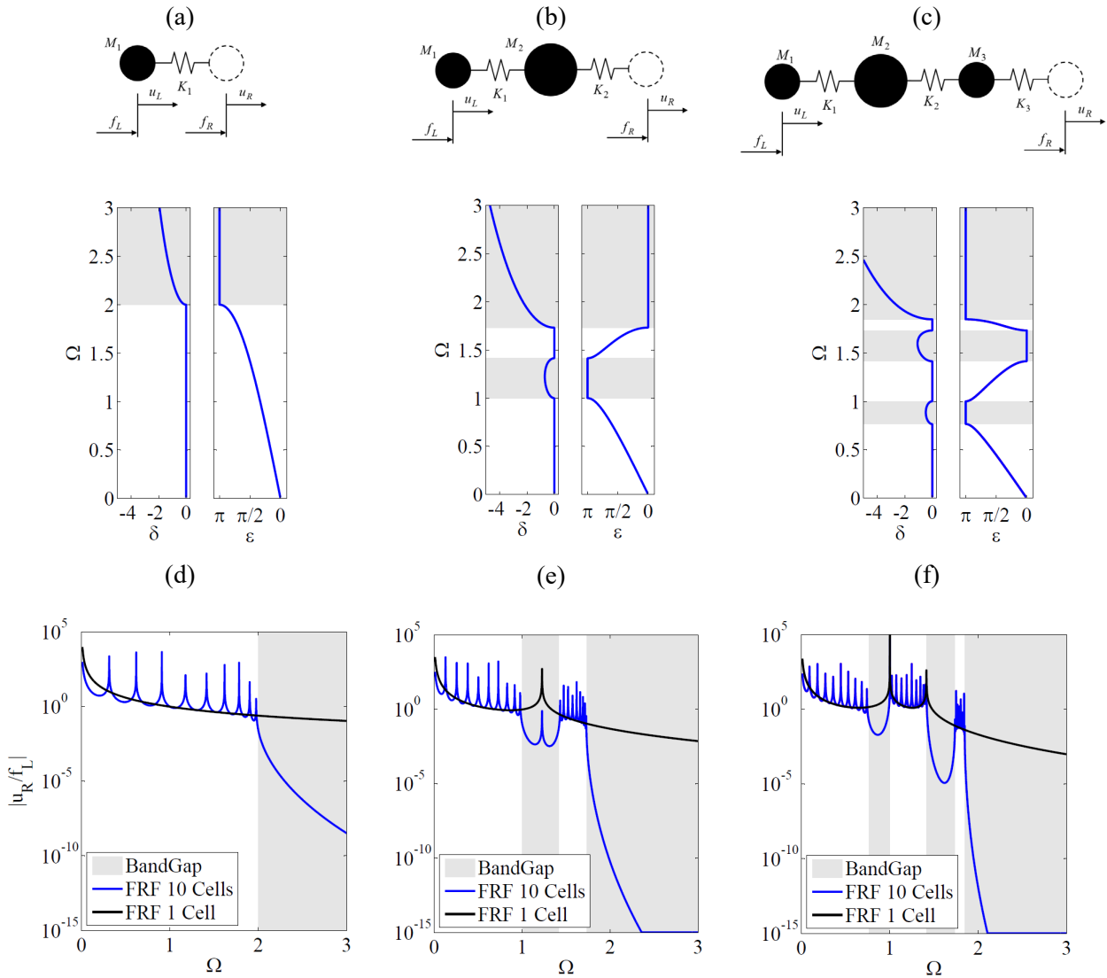
Figure 2.2 Dispersion diagrams for different unit cells: (a) case 1, (b) case 2 and (c) case 3, and FRF amplitudes computed for 1 and 10 cells: (d) case 1; (e) case 2; (f) case 3.
