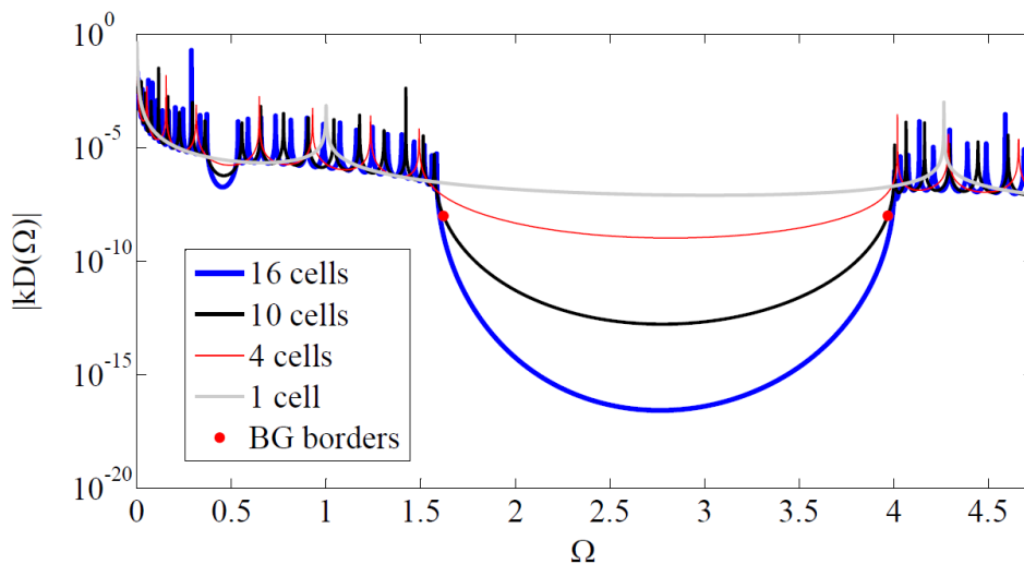
Figure 3.9 Number of cells for a stepped unit cell finite structure for an observable attenuation zone.
