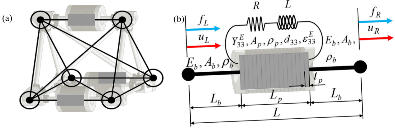
Figure 5.4 (a) Smart unit cell and (b) its piezoelectric stack actuator described as a finite element model.
