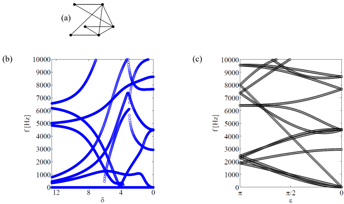
Figure 5.2 (b) Attenuation and (c) phase constants of truss unit cell (a) without concentrated mass on nodes.
