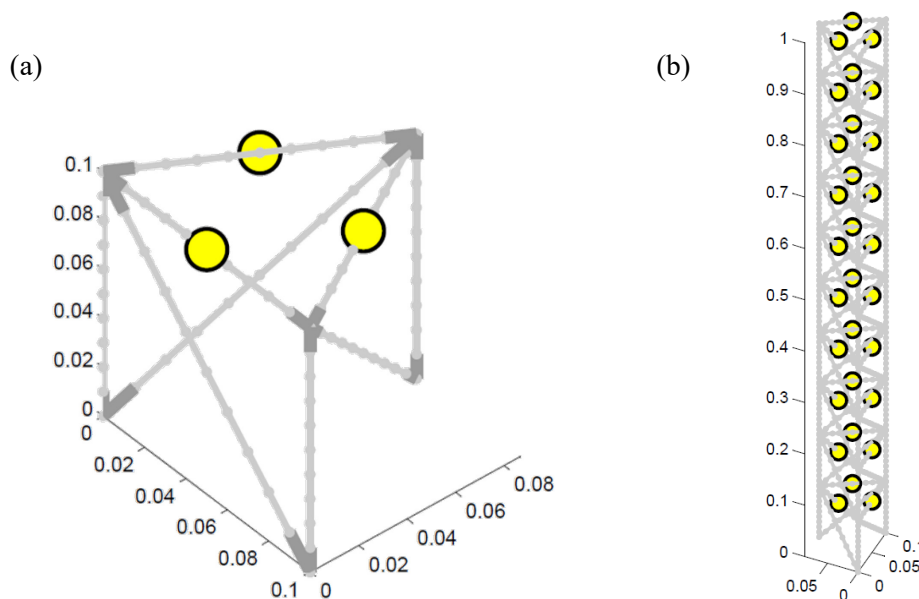
Figure 5.12 (a) Truss unit cell modeled with Euler-Bernoulli beams with concentrated mass on yellow circles dofs and (b) corresponding finite structure.
