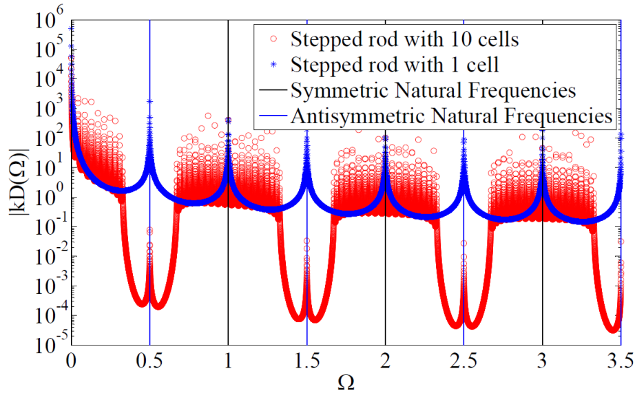
Figure 2.6 Frequency response functions for a free-free periodic stepped rod finite structure with 10 cells, one cell and its exact natural frequencies for symmetric and antisymmetric modes.
