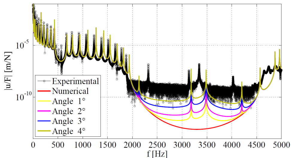
Figure 4.7 FRF with variation on exciting force angle and direction of measured displacement.
