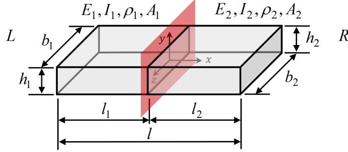
Figure 3.1 Representation of two continuous parts unit cell for a periodic beam structure.
