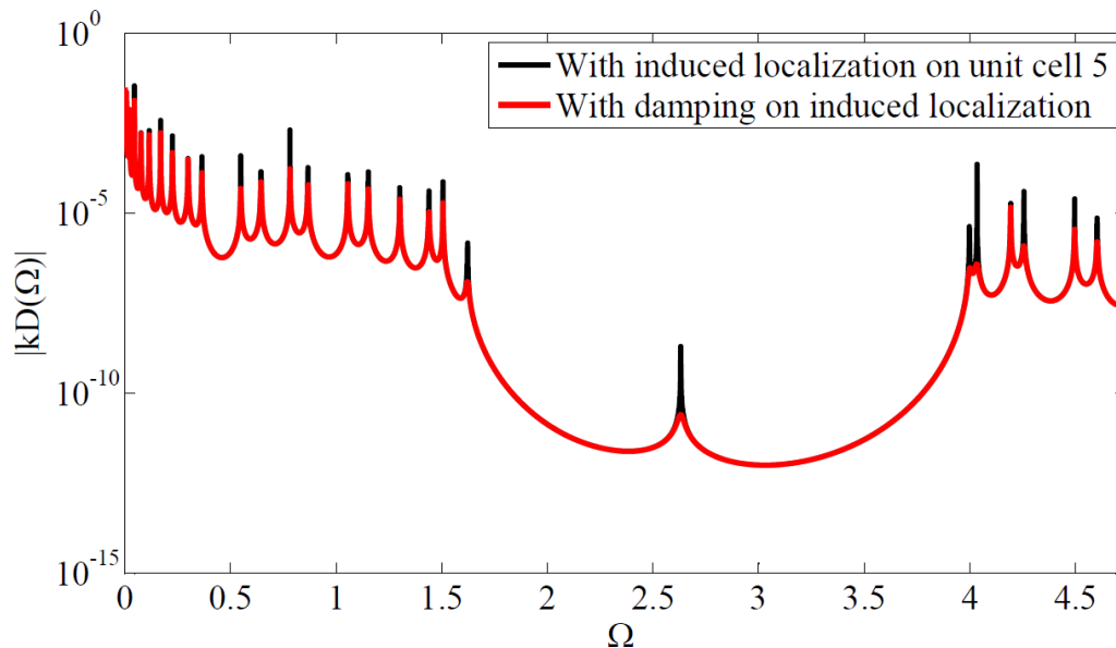
Figure 3.17 FRF of a beam periodic structure with localization phenomena and damping on cell 6.
