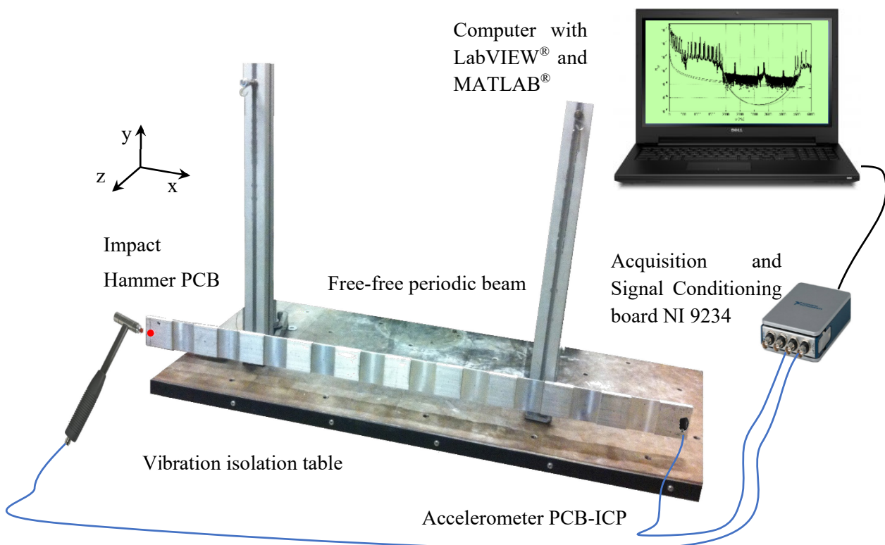
Figure 4.3 Experimental set up for a periodic free-free beam.
