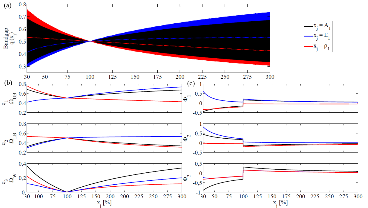
Figure 2.10 (a) Bandgap envelopes, (b) bandgap borders and width; (c) their respective numerical derivatives.
