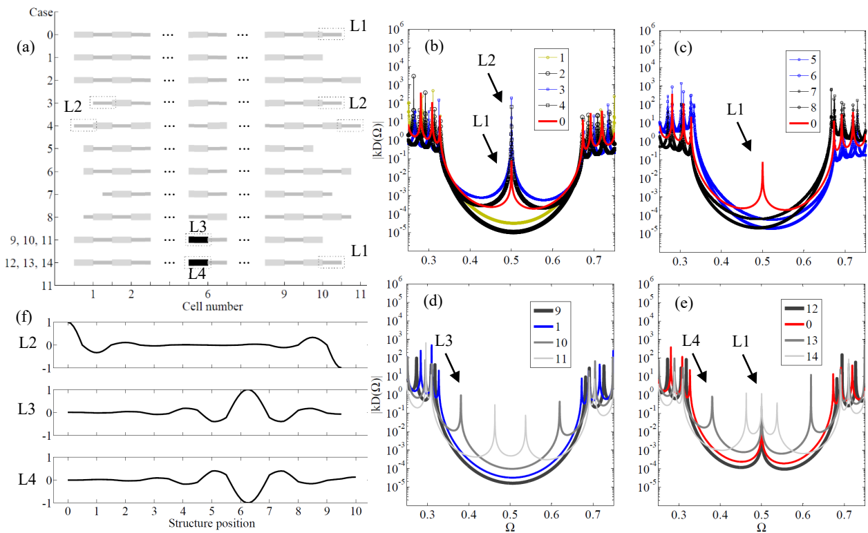
Figure 2.15 (a) 14 different structures cases and their corresponding FRFs for (b) cases 0, 1, 2, 3 and 4; (c) 0, 5, 6, 7 and 8; (d) 1, 9, 10 and 11; (e) 0, 12, 13 and 14; and (f) the shape of localized modes L2, L3 and L4.
