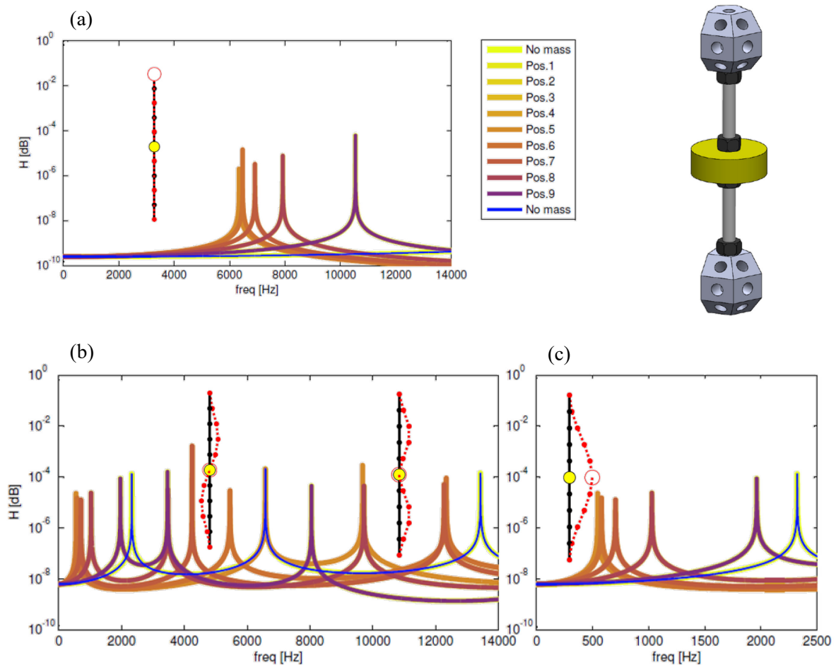
Figure 5.13 Resonant beam with concentrated mass and its (a) first longitudinal mode, (b) first three flexural modes and (c) a zoom of (b) in low frequency.
