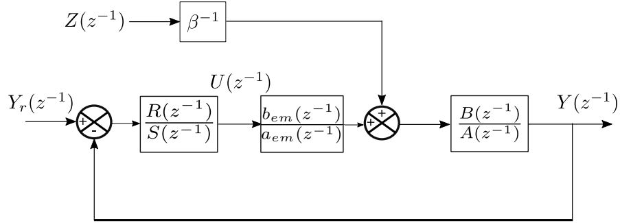
FIGURE 3.6: RST controller structure.
