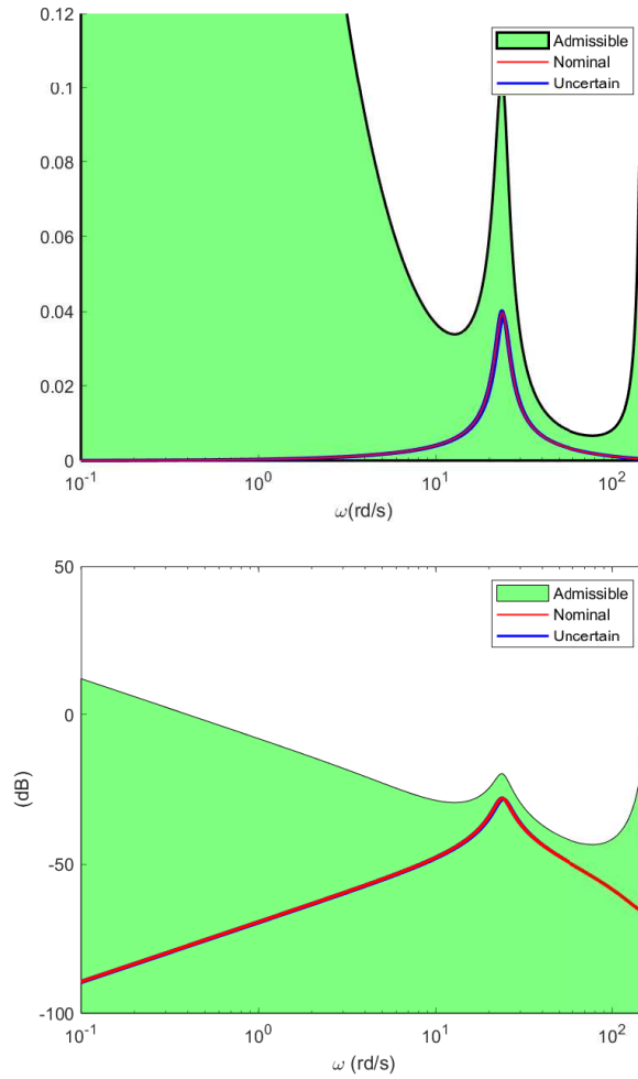
FIGURE 3.11: Nominal system gain |G(z^{-1})| (solid red line), set of open-loop system variations with m' \in [0.5 m, 1.5 m] (blue area), and admissible region for |G'(z^{-1})| to be stabilizable (green area) when in closed-loop with (3.27) in natural scale (top) and dB scale (bottom).
