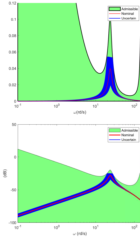
FIGURE 3.14: Nominal system gain |G(z^{-1})| (solid red line), set of open-loop system variations with m' \in [0.5m, 1.5m] , c' \in [0.75c, 1.25c] , and k' \in [0.75k, 1.25k] (blue area), and admissible region for |G'(z^{-1})| to be stabilizable (green area) when in closed-loop with (3.27) in natural scale (top) and dB scale (bottom).
