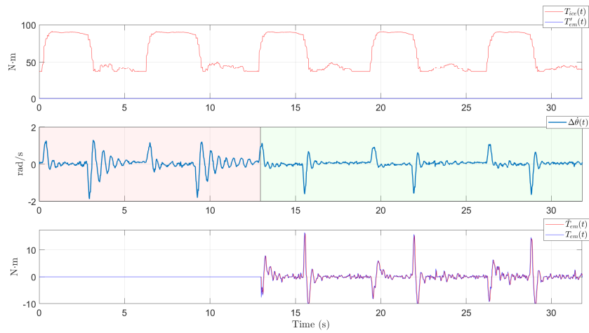
FIGURE 3.22: Top: ICE and EM torque setpoints. Middle: measured torsional speed \Delta\dot{\theta} . Bottom: total EM torque setpoint, T_{em} , and the measured torque, \tilde{T}_{em} . The RMS values, (3.26), are 0.296 and 0.418 with and without the damping controller: a 29.33% reduction. The experiment was carried out with the first gear engaged: R(i) = 16.45 . The red and green backgrounds at the middle of the figure indicate when the damping controller remained off and on, respectively.
