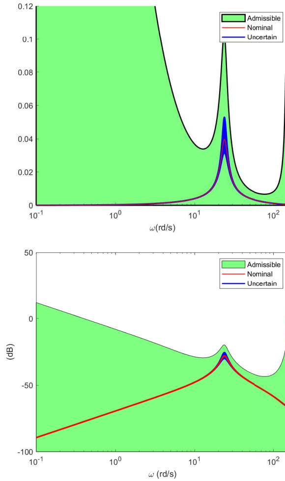
FIGURE 3.12: Nominal system gain |G(z^{-1})| (solid red line), set of open-loop system variations with c' \in [0.75c, 1.25c] (blue area), and admissible region for |G'(z^{-1})| to be stabilizable (green area) when in closed-loop with (3.27) in natural scale (top) and dB scale (bottom).
