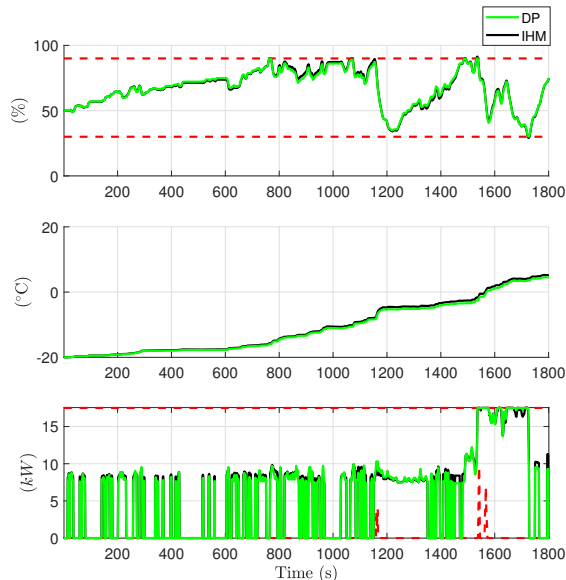
FIGURE 2.11: Solution to (2.52) for the low-temperature operation and the WLTC-C3 driving cycle with DP (green solid line) and the proposed implicit Hamiltonian minimization (black solid line). The red dashed lines at the top and bottom subfigures represent the bounds on the state-of-energy and the control input, (2.52e) and (2.52d), respectively.
