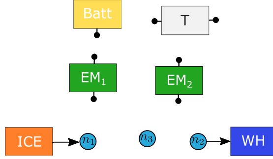
FIGURE 4.17: Topology design corresponding to simultaneous MILP (4.46).
