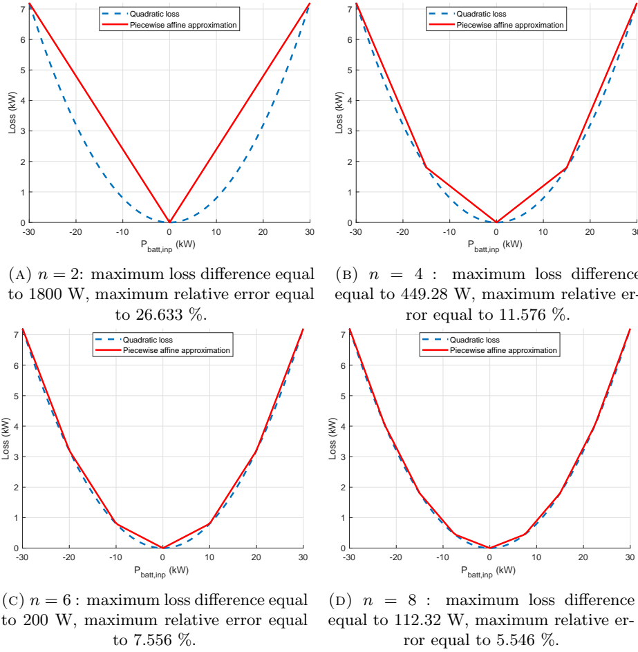
FIGURE 4.11: Piecewise approximations for the battery loss model.
