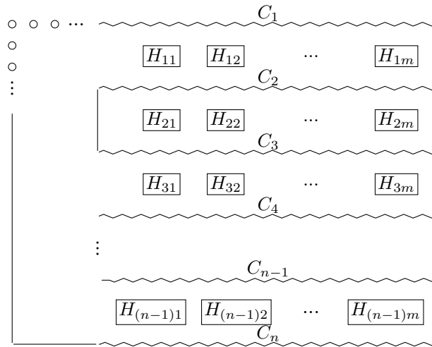
Figure 4.6: Papadimitriou's high-level construction
