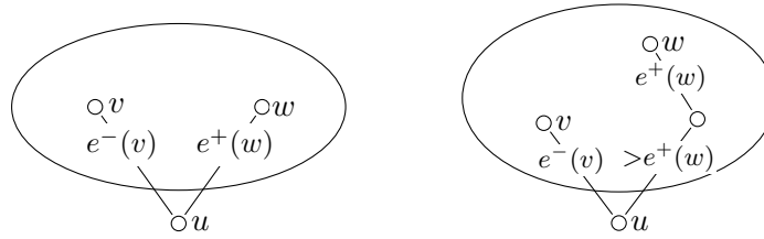
(a) Dismountability principle. (b) Example of 2-hop dismantlability.
