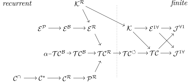
Figure 5.1: Hierarchy surrounding temporal connectivity (figure from [18]). (Same Figure as used in Chapter 2.)
