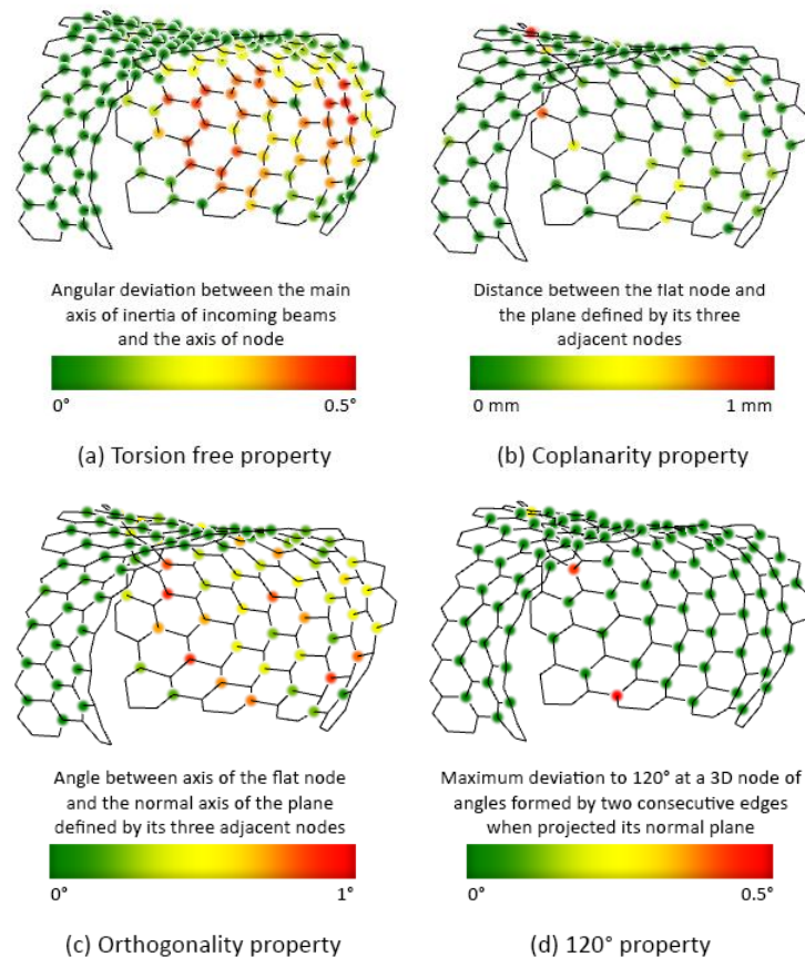
Figure 4.33: Fulfillment of Caravel properties for the heX-mesh Pavilion (image courtesy of Mathieu Lerouge)
