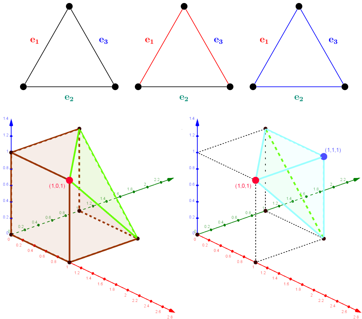
Figure 4.2: A graph G , a tree, and a 1-connected spanning subgraph. Below, the forest polytope, the tree polytope, and the connector polytope of G . Note that the tree polytope is a face of both the forest and the connector polytopes.
