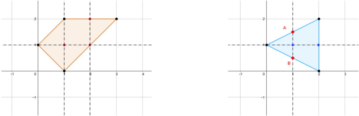
Figure 1.2: A box-integer polytope (left) and a non box-integer polytope (right): A and B are non integer points given by the intersection with an integer box-constraint.
