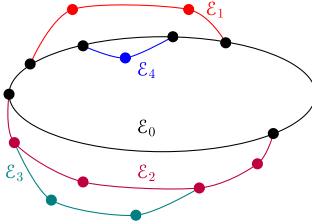
Figure 1.9: An open nested ear decomposition.
