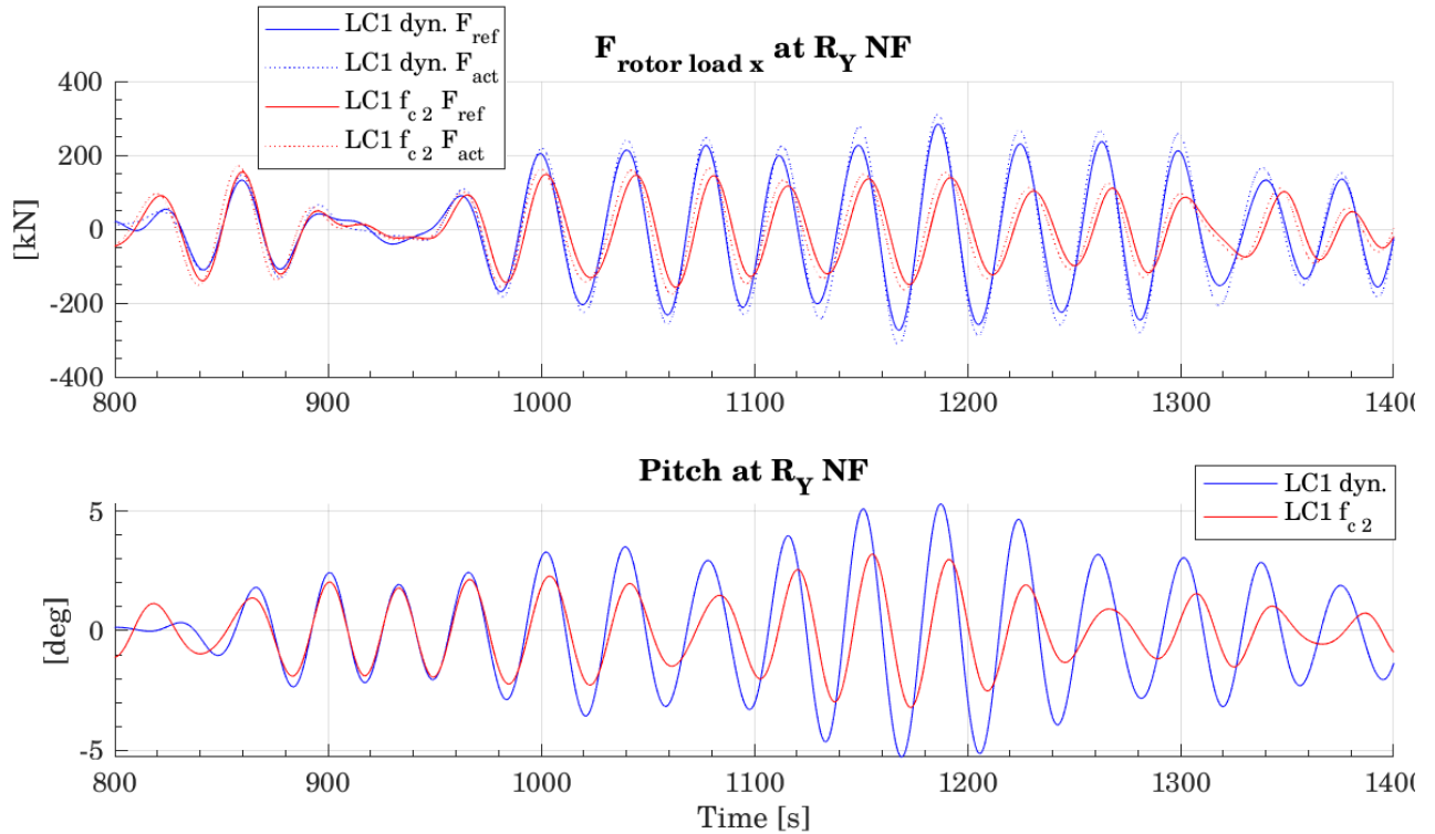
Figure 96: Actuator force (a) and platform pitch (b)
