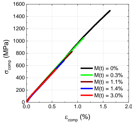
Figure 68 : Apparent compression stress-strain plots for C/PA6 specimens tested with the pin-ended buckling test fixture under several saturated aging conditions
