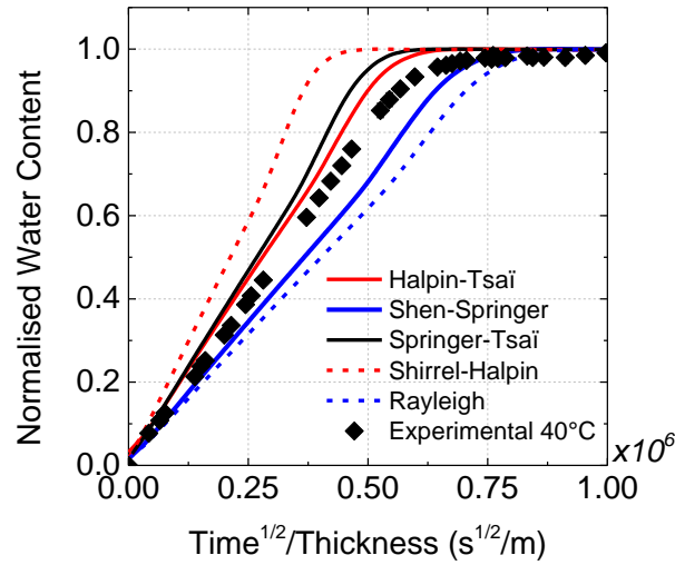
Figure 53: Comparison of the transverse coefficient of diffusion obtained using the equations described in Table 6
