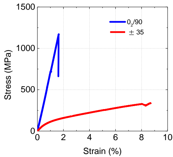
Figure 124 : Stress-strain plots of specimens which sequences at [\pm 35] and [0_2/90]
