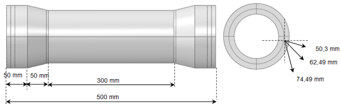
Figure II-A: Dimensions of the [0/\pm 88] cylinder
