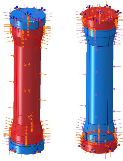
Figure II-D: Pressure conditions
