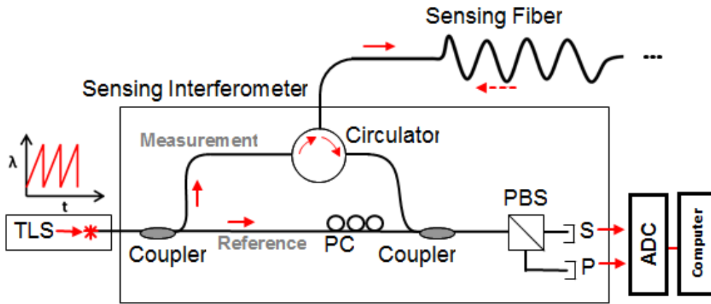
Figure 28 : Basic OFDR optical network
