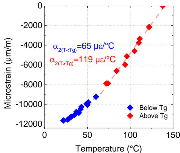
Figure 104 : Residual strain relaxation with temperature and measurement of the transverse CTE
