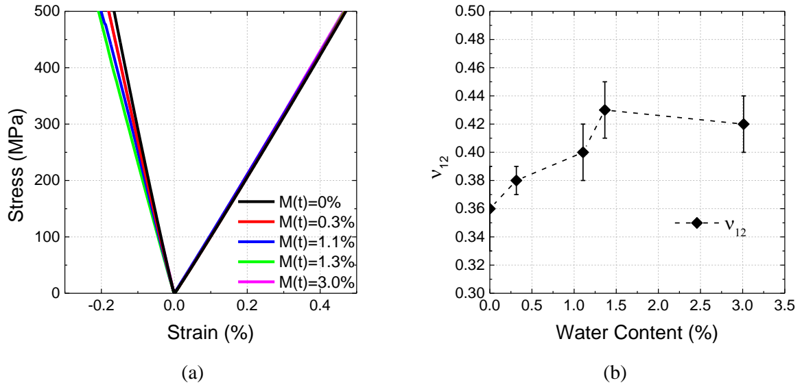
Figure 60 : Effect of water on (a) the longitudinal and transverse strains under tensile loading (b) Poisson's ratio \nu_{12} for C/PA6 specimens
