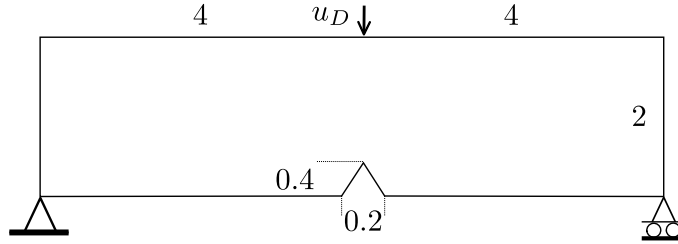
Figure 3.13 – 3-PB geometry and boundary conditions.
