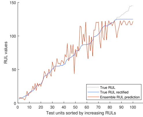
(b) sorted RUL of test units in FD003
