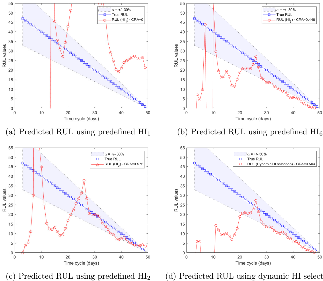
Figure 3-9: RUL prediction comparison when using predefined HI and dynamic HI selection
