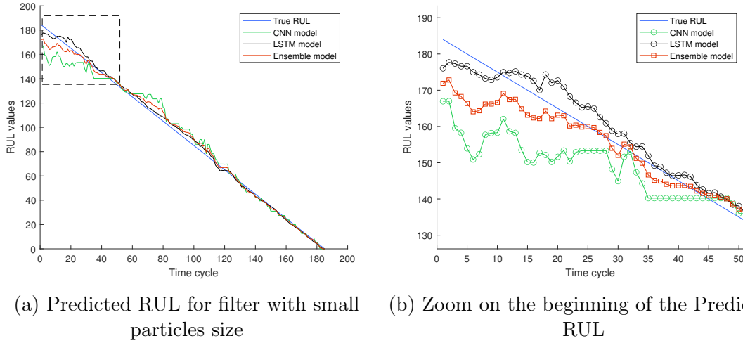
Figure 4-21: Predicted RUL for filter with small particles size in the test set
