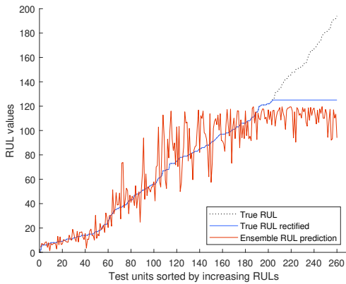
(c) sorted RUL of test units in FD002
