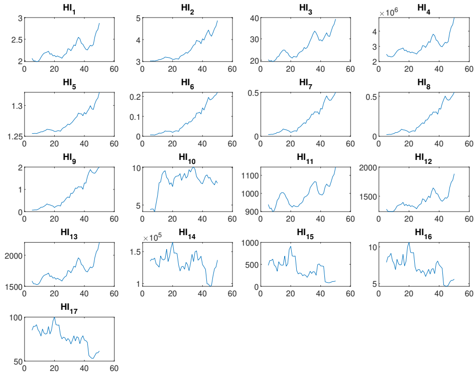
Figure 3-7: Computed indicators using HIs of Table 3.1
