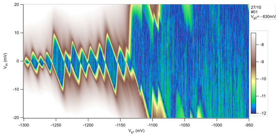
(a) Coulomb diamonds related to the dot 1 in the few holes regime taken along the V_{g2} = -630 mV line. Going rightward, the height of the diamonds, hence the addition energy, gets bigger and bigger. This is a strong indication that effectively we are reaching the few hole regime. Unfortunately, the actual setup did not allow us to go beyond V_{dc} = 20 mV. The many hole regime is presented in the other figure 5.6b.
