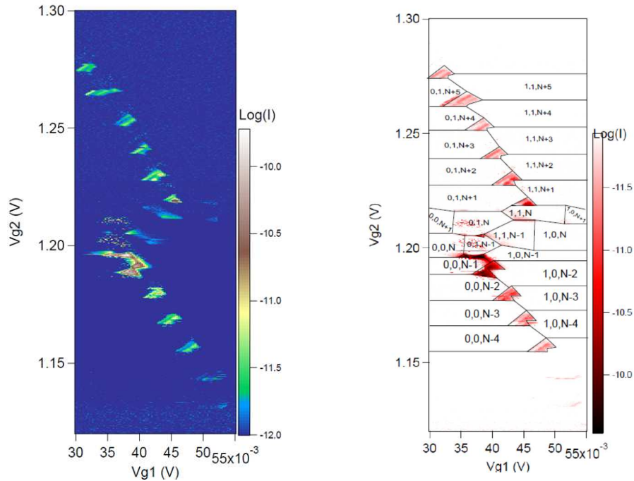
Figure 4.9 Left panel: A stability diagram recorded in log scale at base temperature in the configuration where only the outer dot 2 carries many electrons. The backgate voltage is +30 V and the bias voltage is +1.35 mV. In this region the topgate 1 voltage is close to 0 V ensuring the dot 1 to carry a low numbers of electrons. Moreover the break in the line of triangles indicates a change of the number of electrons of the central dot. Finally the big bias voltage eventually opens big bias triangles. Right panel: Same area but with a different color scale. We make here an attempt to index the stability diagram. Inside the bias triangles we also see lines parallel to the base of the triangles indicatind excited states.
