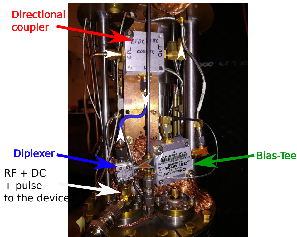
Figure 3.18 Close picture of one full channel consisting of a bias tee cascading a diplexer. On top of the picture is the directional coupler (red) for the RF tone (white arrow) connected to the high frequency port diplexer (blue) with the blue wire. Close to the diplexer is the bias tee (green), summing the DC bias (grey arrow) and the pulsed signal (brown arrow). The output is sent to the low frequency port of the diplexer. The final signal coming from the diplexer is sent to one of the two gates of the device. The other gate has its own full channel.
