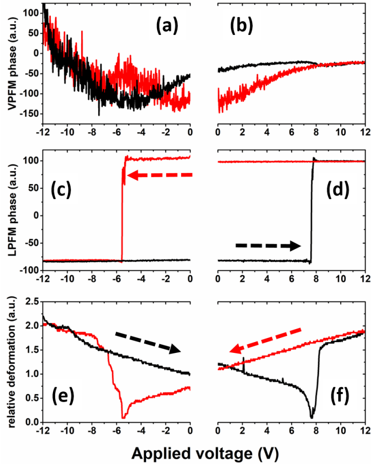
Figure 4.18: Discontinuous writing procedure on a domain in mica//Au/Co/CA(50 nm) film. Upper ((a) and (b)) and middle panels ((c) and (d)) show the VPFM and LPFM phase variation respectively with respect to the applied voltage during spectroscopy. Lower panel ((e) and (f)) shows the grain deformation or tip deflection. Dashed arrows show the direction of voltage increment.
