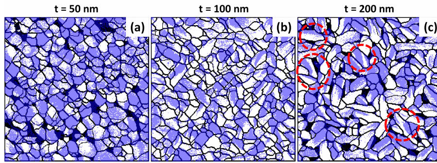
Figure 4.10: Topography contours superimposed on LPM phase maps. Black lines represent the grain boundaries and the white (minimum)-purple (maximum) shades represent the contrast of LPM phase response of mica//Au/CA films of thickness, t (a) 50 nm, (b) 100 nm and (c) 200 nm in a region of area 2 \times 2 \mu\text{m}^2 . Red dashed circles in panel (c) show some multi-domain grains. Black regions represent morphological voids.
