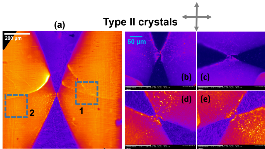
Figure 6.13: Optical polarimetry on a type-II crystal. (a) shows a large scale image and (b)-(e) show images of the same crystal at different rotation angles of the crystal. Dashed boxes represent regions of interest for expanded views shown in upcoming figures.
