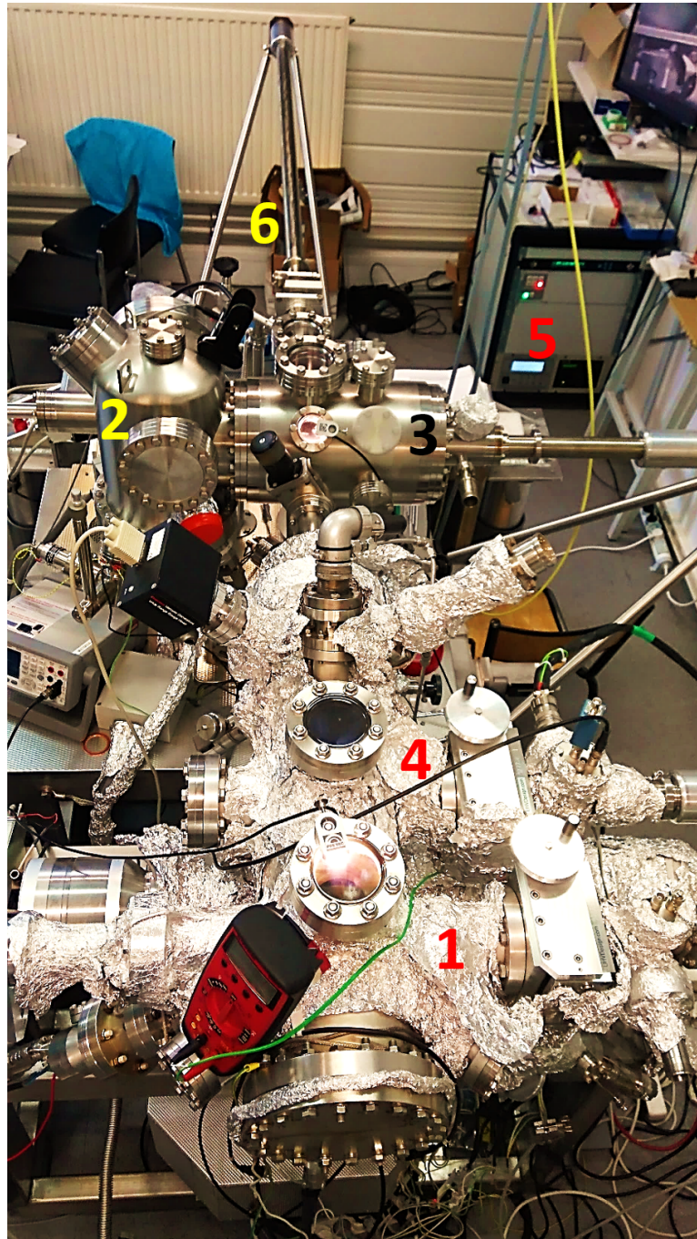
Figure 3.5: Top view of the multi-probe system. 1- thin film growth section, 2- surface characterization section, 3- sample storage region, 4- surface preparation region, 5- system operation control system, 6- magnetic transfer arm
