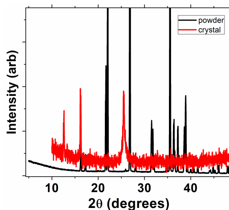
Figure 6.7: Comparison of XRD peaks of type-I crystal to that of the source powder. Wavelength of X-ray used is 1.5406 \text{ \AA} .
