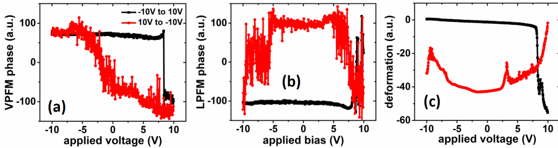
Figure 4.12: Results of a typical switching attempt on mica//Au/CA(50 nm) sample. (a) and (b) show the variation VPFM and LPFM phase with respect to applied voltage during the spectroscopy. (c) shows the tip deflection or grain deformation. Although no robust or clear switching can be observed, (a) seems to have a switching features appearing only on the positive bias side.
