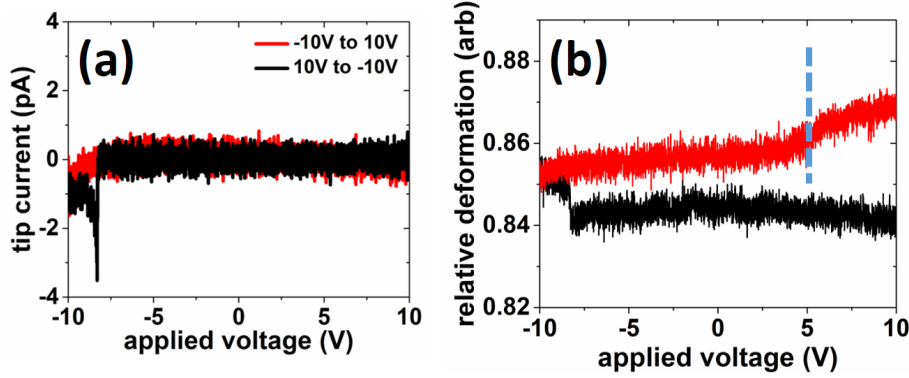
Figure 5.12: Switching current spectroscopy results on the concerned nanoscopic region. No AC excitation signal is applied during the measurement. Gradual reversal kinetics results in the disappearance of switching current peak on the positive voltage side. Dashed line in (b) indicates the approximate voltage position from where the grain deformation starts to take place as visible on the red curve.
