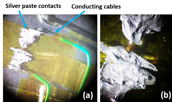
Figure 6.17: Arrangements to electrically pole along the length of the crystal of type-I.
