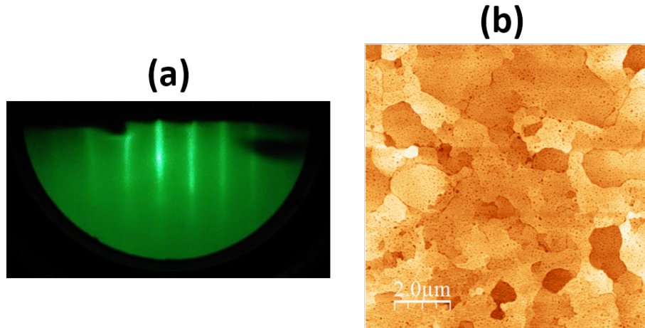
Figure 4.2: Characterization of mica//Au substrate surface. (a) shows the in-situ RHEED patterns obtained after the growth. (b) shows the surface topography as obtained from AFM imaging. Sections of different contrast in (b) represent atomically flat isolated planes of Au surface.
