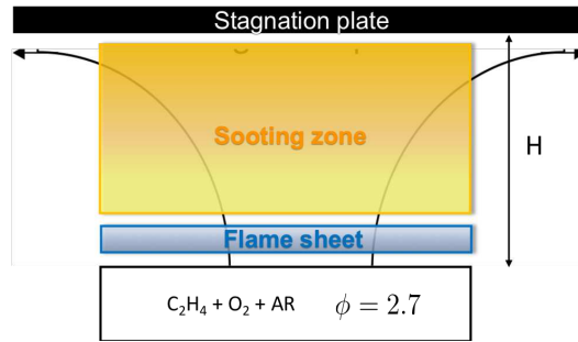
Figure 2.1: Schematic representation of the laminar burner-stabilized stagnation premixed flame ( H is the position of the stagnation plane above the burner where soot particles are collected by scanning mobility particle size (SMPS)).
