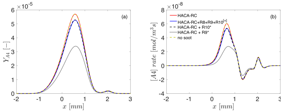
Figure 3.3: Impact of the surface kinetics on PAH prediction for the non-premixed flame. (a) Pyrene ( A_4 ) mass fraction with the reference HACA-RC (red line), with the three proposed radicals (blue line) without modification ( k_{react}^{[+]} in Table 3.1), with only C_3H_3 (dashed black lines) with modified reaction constants ( k_{react}^* in Table 3.1), with only CH_3 using k_{react}^* (dotted black line) and not considering soot production (yellow dashed line); (b) the corresponding A_4 chemical production rate.
