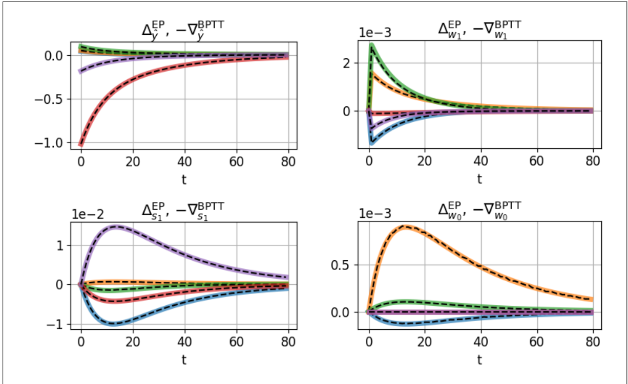
Figure 4.3: Real-time RNN with symmetric weights with one hidden layer. Left: \Delta_s^{\text{EP}}(t) neural updates and -\nabla_s^{\text{BPPT}}(t) gradients. Right: \Delta_\theta^{\text{EP}}(t) weight updates and -\nabla_\theta^{\text{BPPT}}(t) gradients.
