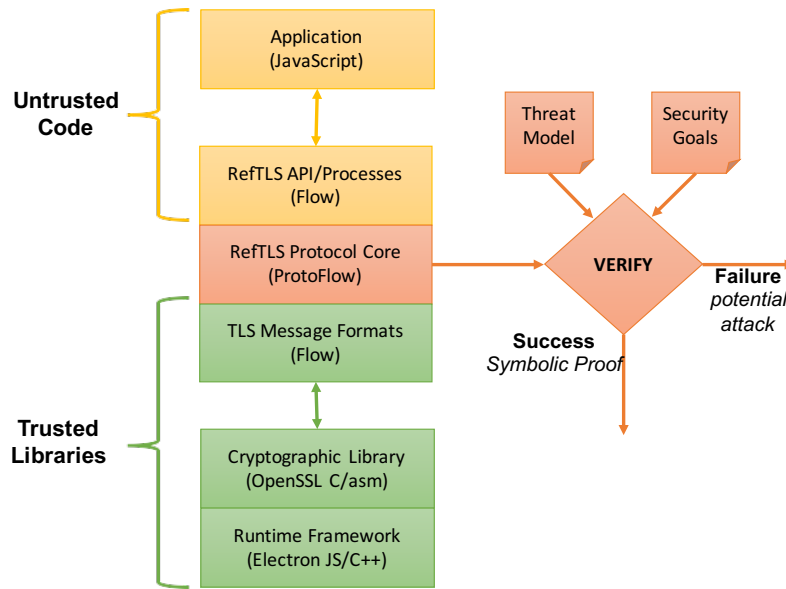
Figure 5.6: RefTLS Architecture.
