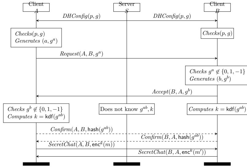
Figure 1.1: Telegram’s MTPROTO Protocol for Secret Chats.
