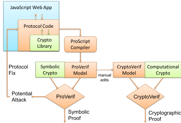
Figure 5.1: Verification Approach.
