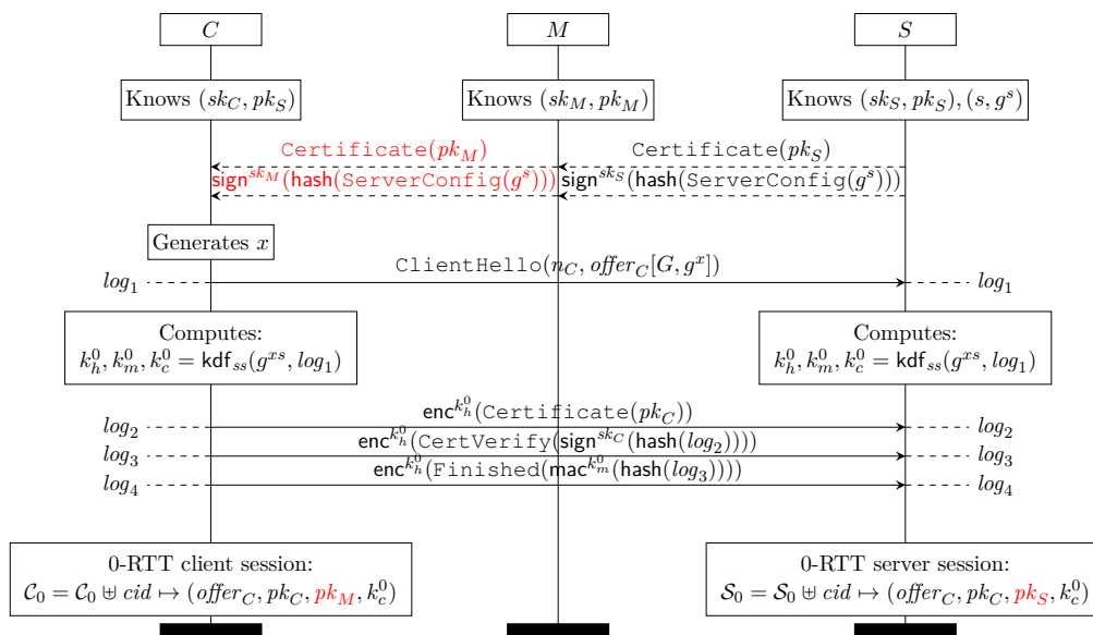
Figure B.2: Unknown Key Share (UKS) Attack in QUIC, OPTLS and on TLS 1.3 Draft-12 if the server’s certificate is not added to log_1 . The figure shows how a man-in-the-middle can exploit the UKS to mount a credential forwarding attack on 0-RTT client authentication. This attack led to the inclusion of Certificate and ServerConfig in the 0-RTT handshake hash in Draft-7.
