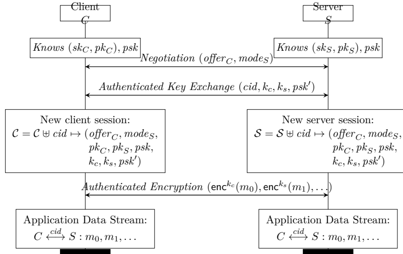
Figure 2.1: TLS Protocol Structure.
