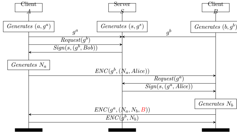
Figure 2: The Needham Schroeder Public-Key Protocol. This simple protocol, first described in 1978, was not broken until 1995 when a man-in-the-middle attack was discovered using automated formal verification in the symbolic model. By adding the component highlighted in red, the vulnerability can be addressed.
