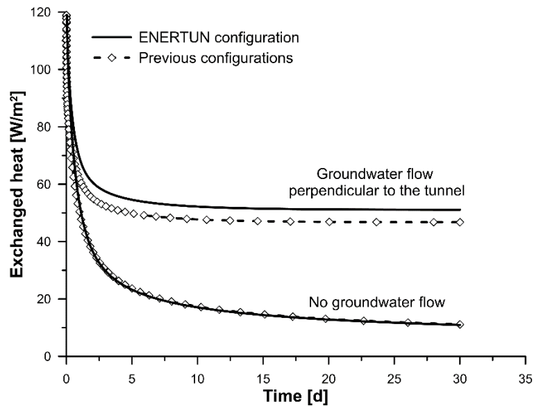
Figure 2.7: Comparison between Enertun and previous configurations in terms of heat (modified from Barla et al., 2019).
