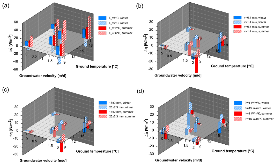
Figure 5.16: Effect of (a) fluid inlet temperature, (b) fluid velocity, (c) pipes size and (d) heat transfer coefficient on geothermal potential during winter and summer conditions expressed in terms of heat flux variations in the case perpendicular flow.
